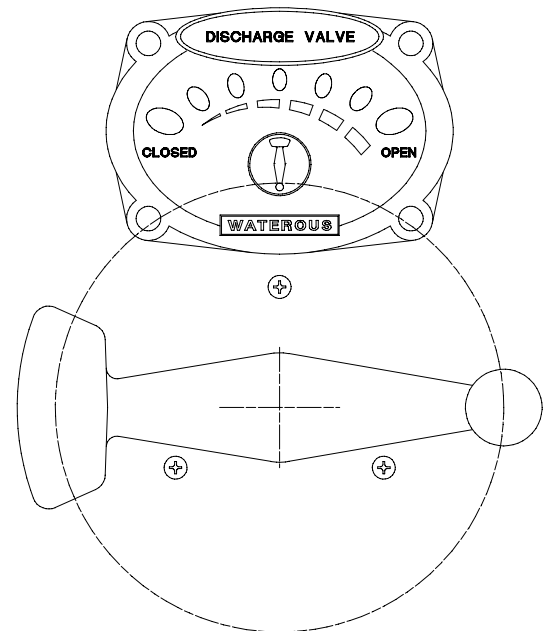
Manual Valve Position Control
