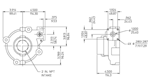
MODEL PB18-G2015-LE
