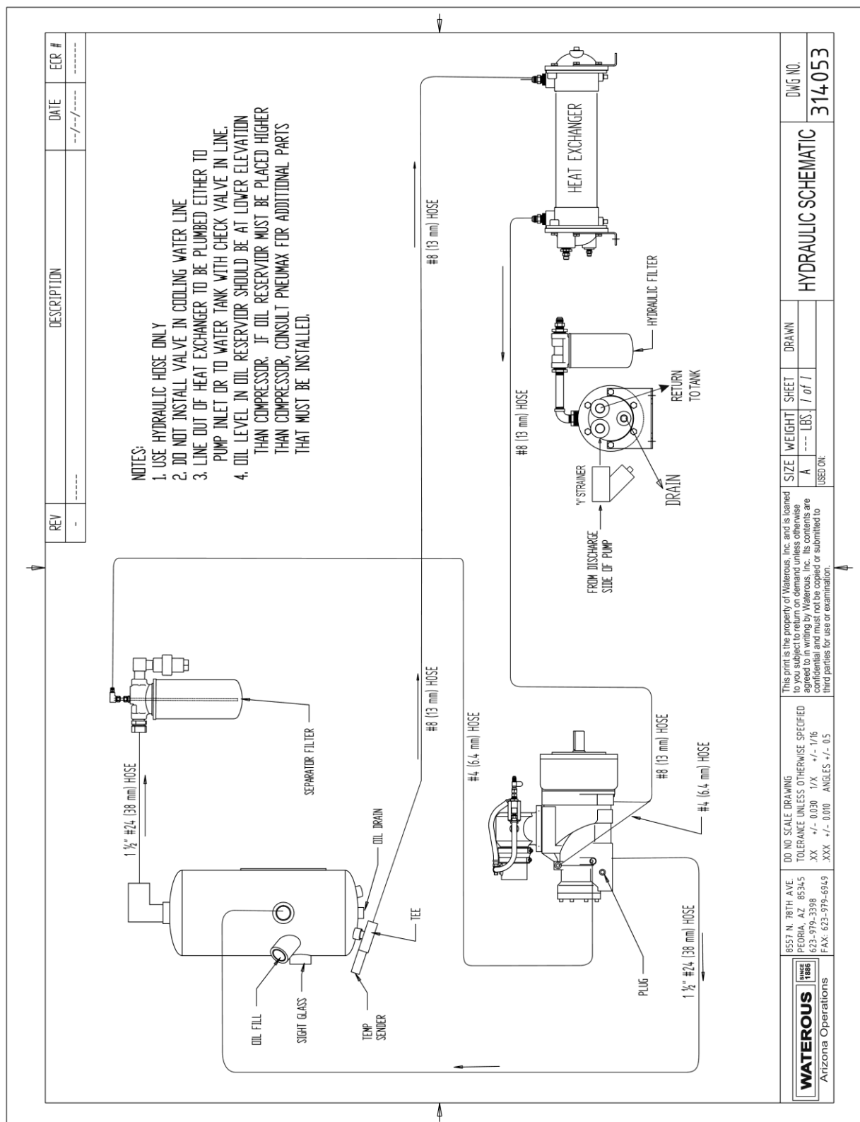
Figure 11 Hydraulic Schematic, Vertical Sump
