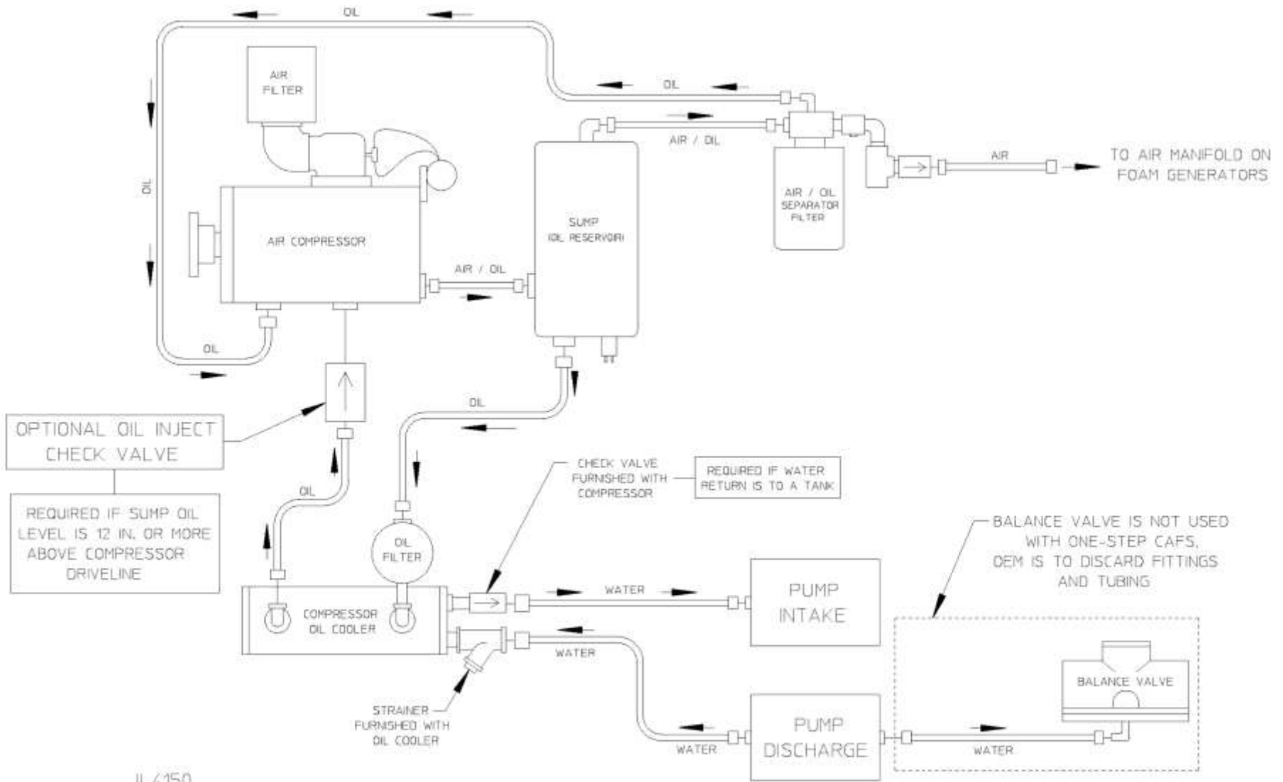
OPTIONAL HOSE AND FITTING KIT ASSEMBLY 83368
