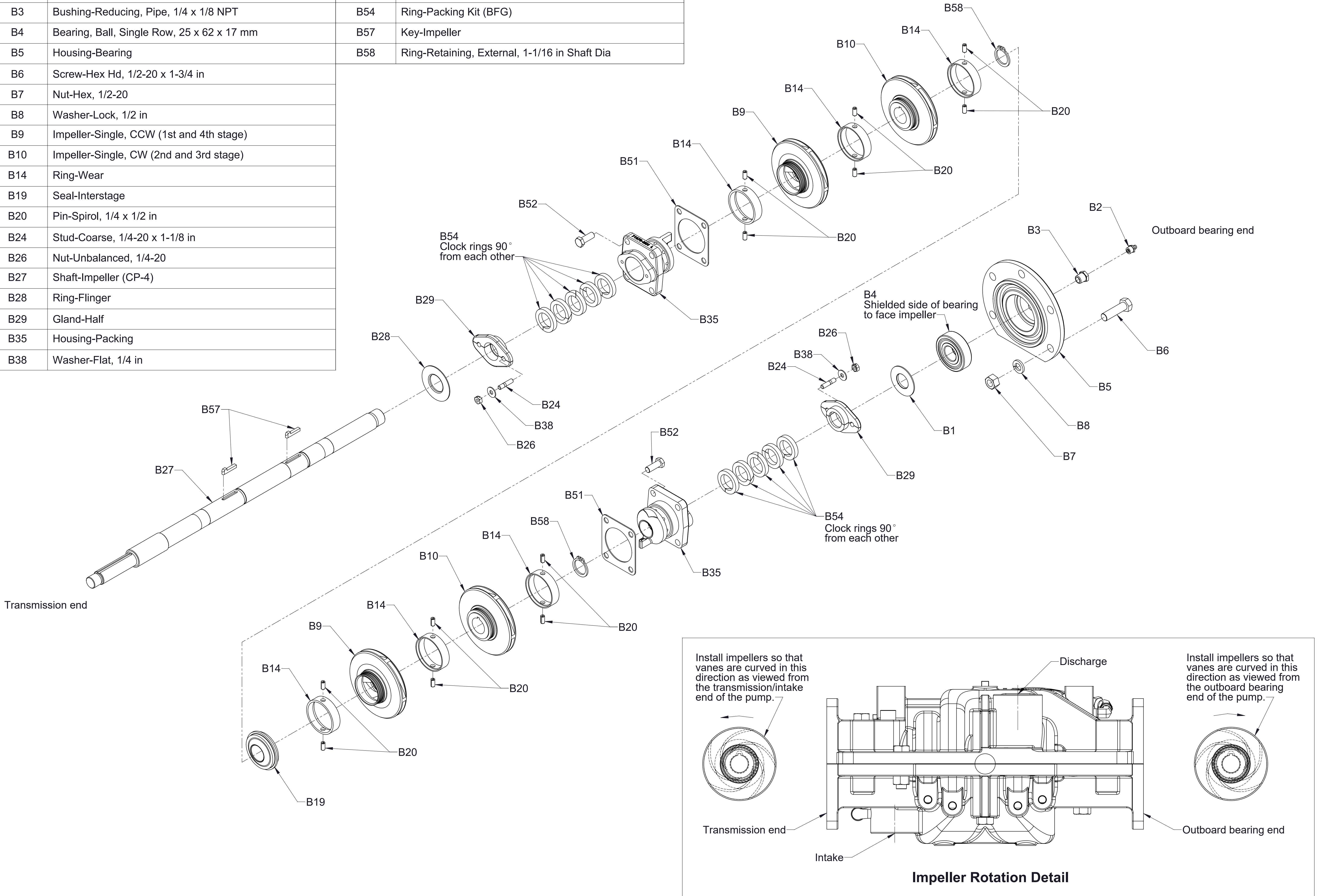
Impeller Shaft Components
