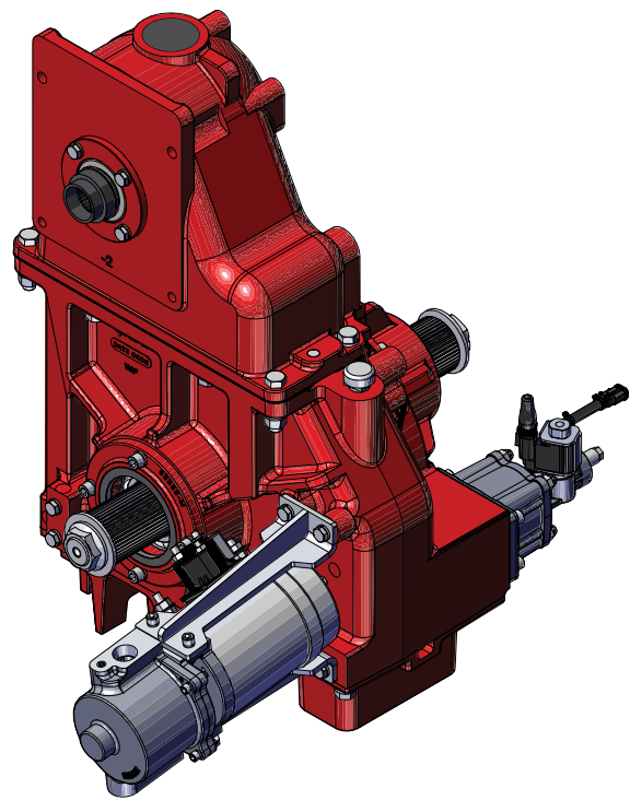
C22—Current Generation
