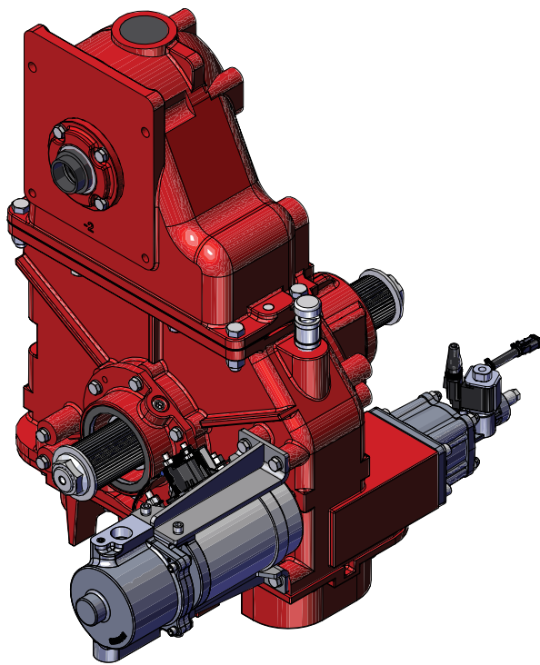
C20—Previous Generation
