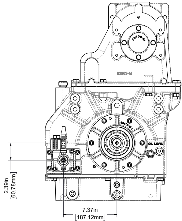
C22 TRANSMISSION
