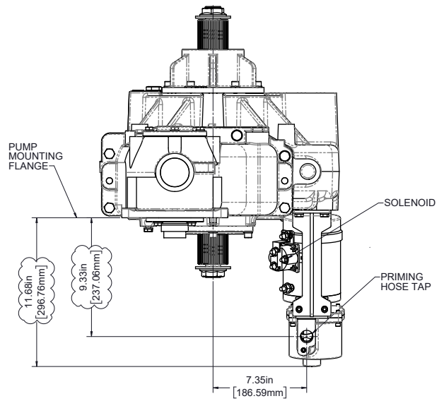
C22 TRANSMISSION
