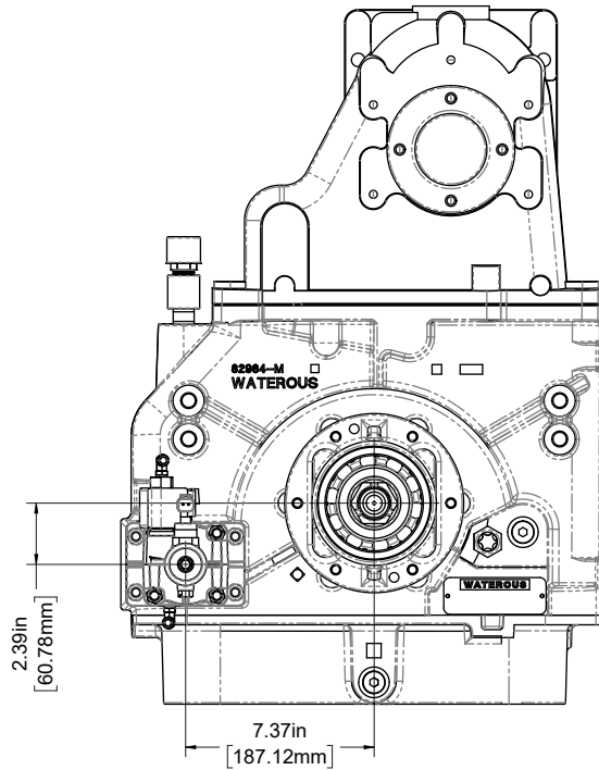
C20 TRANSMISSION
