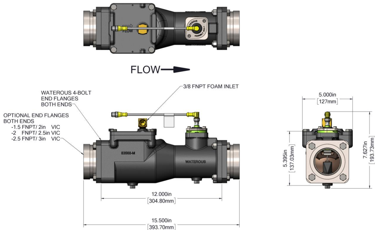
Figure A. Foam Manifolds
