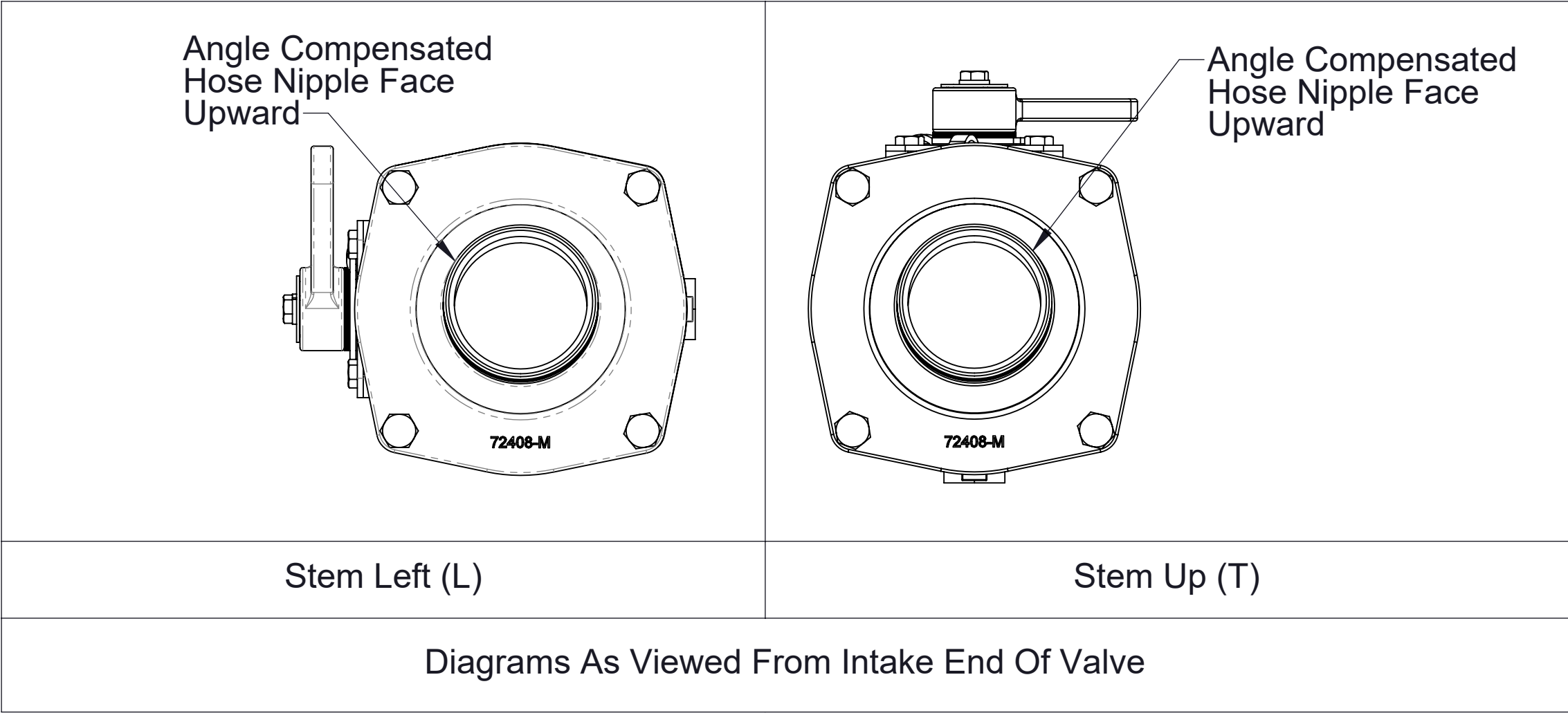
Detail B Stem Mounting Positions Letter "T" or "L" Added So That The Correct Angle Compensation Of The Fitting Is Maintained
