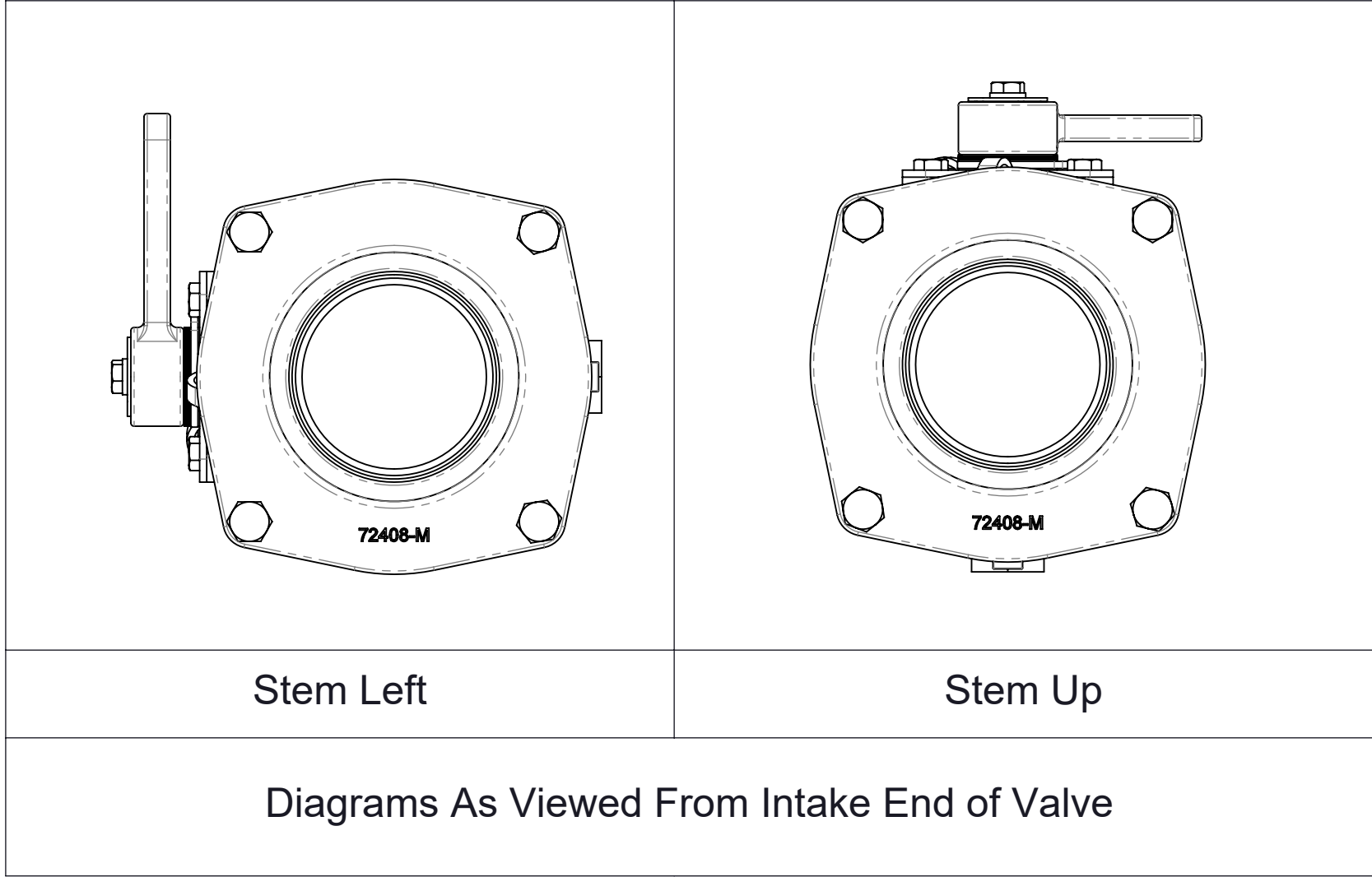
Detail A Stem Mounting Positions Note: Obtained By Rotating Valve
