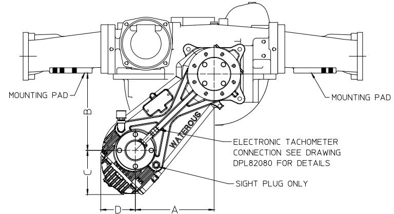
MODEL CSPA, ASS'Y NO. 82062-4 MODEL CSUPA, ASS'Y NO. 82062-5 MODEL CSPA 1.90 RATIO SHOWN
