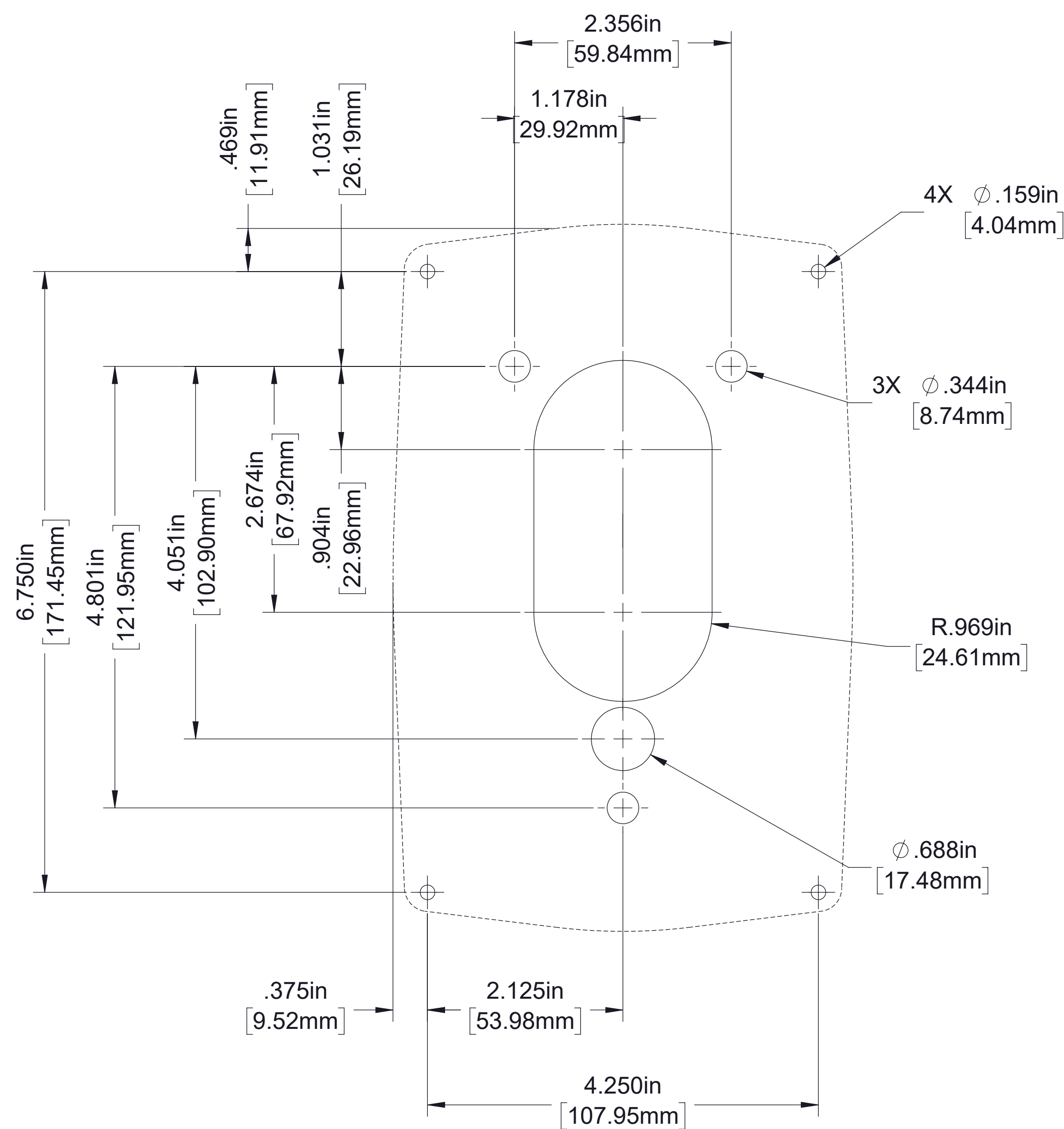
Panel Hole Layout
