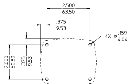
PANEL HOLE LAYOUT
