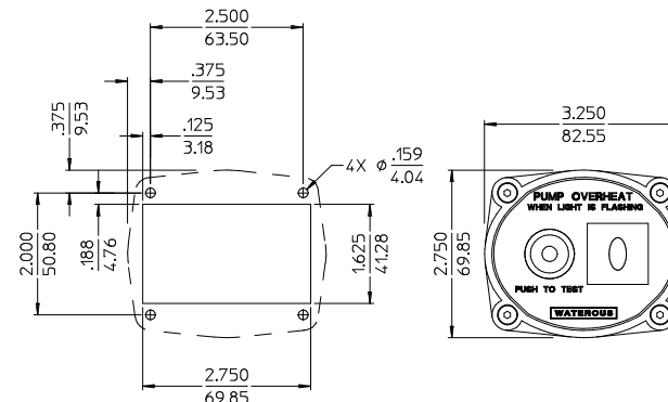
PANEL HOLE LAYOUT
