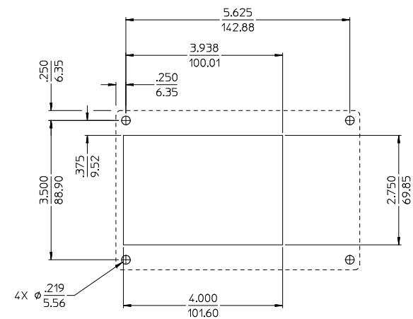
IN-CAB PANEL HOLE LAYOUT
