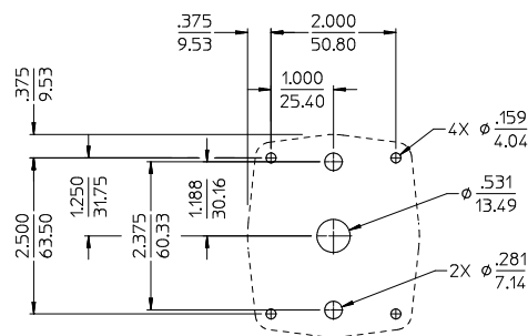
PANEL HOLE LAYOUT
