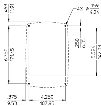
PANEL HOLE LAYOUT
