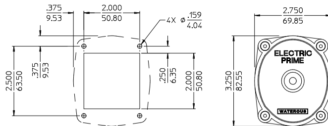
PANEL HOLE LAYOUT
