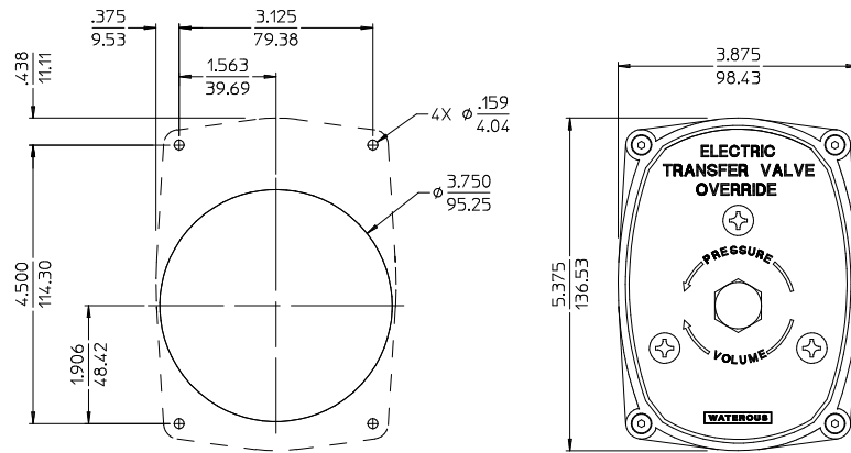
PANEL HOLE LAYOUT
