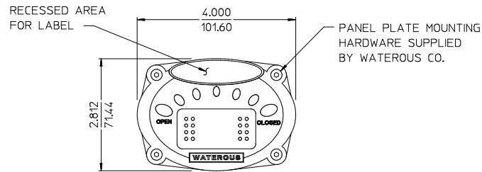
ELECTRIC ROTARY ACTUATOR
