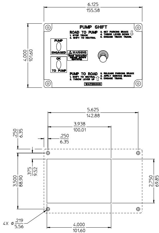
IN-CAB PANEL HOLE LAYOUT
