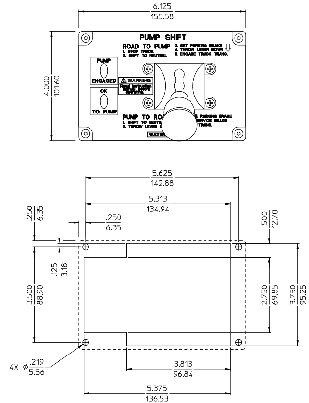
IN-CAB PANEL HOLE LAYOUT
