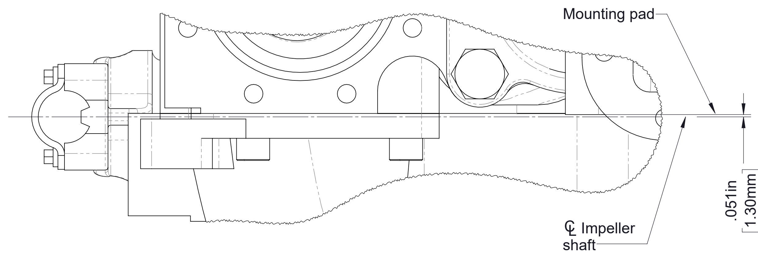
DETAIL A
