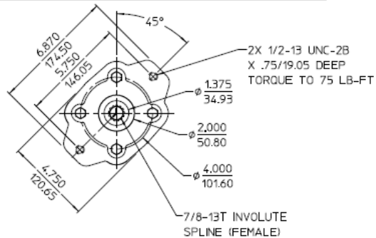
VIEW F-F HYDRAULIC PUMP ADAPTER FLANGE USED FOR SAE J744 CLASS B 2-BOLT HYDRAULIC PUMP WITH MALE 7/8-13T 16/32 PITCH INVOLUTE SPLINE
