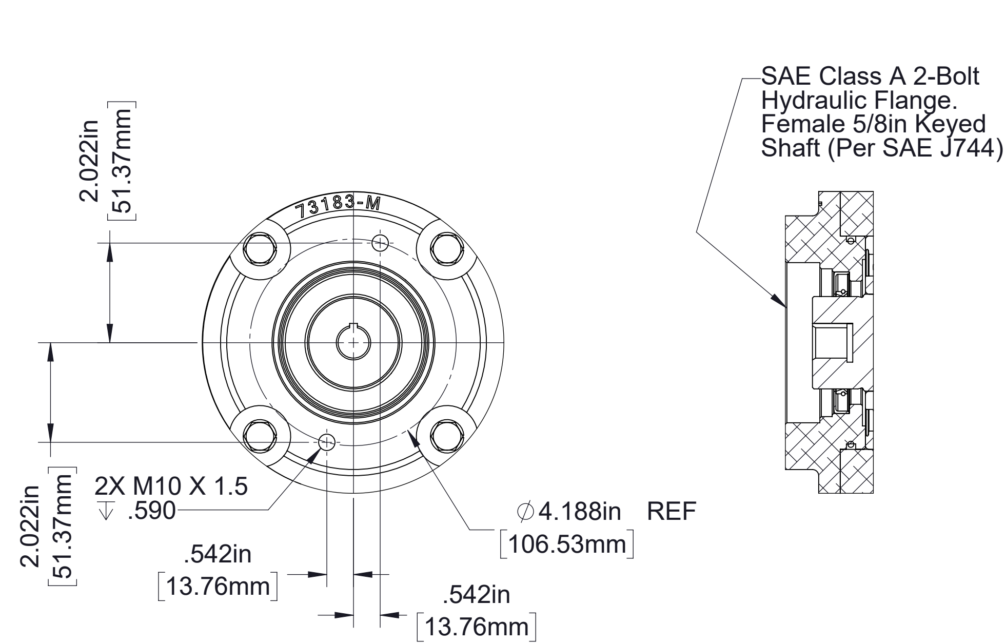
Detail B Hydraulic Flange Adapter Output
