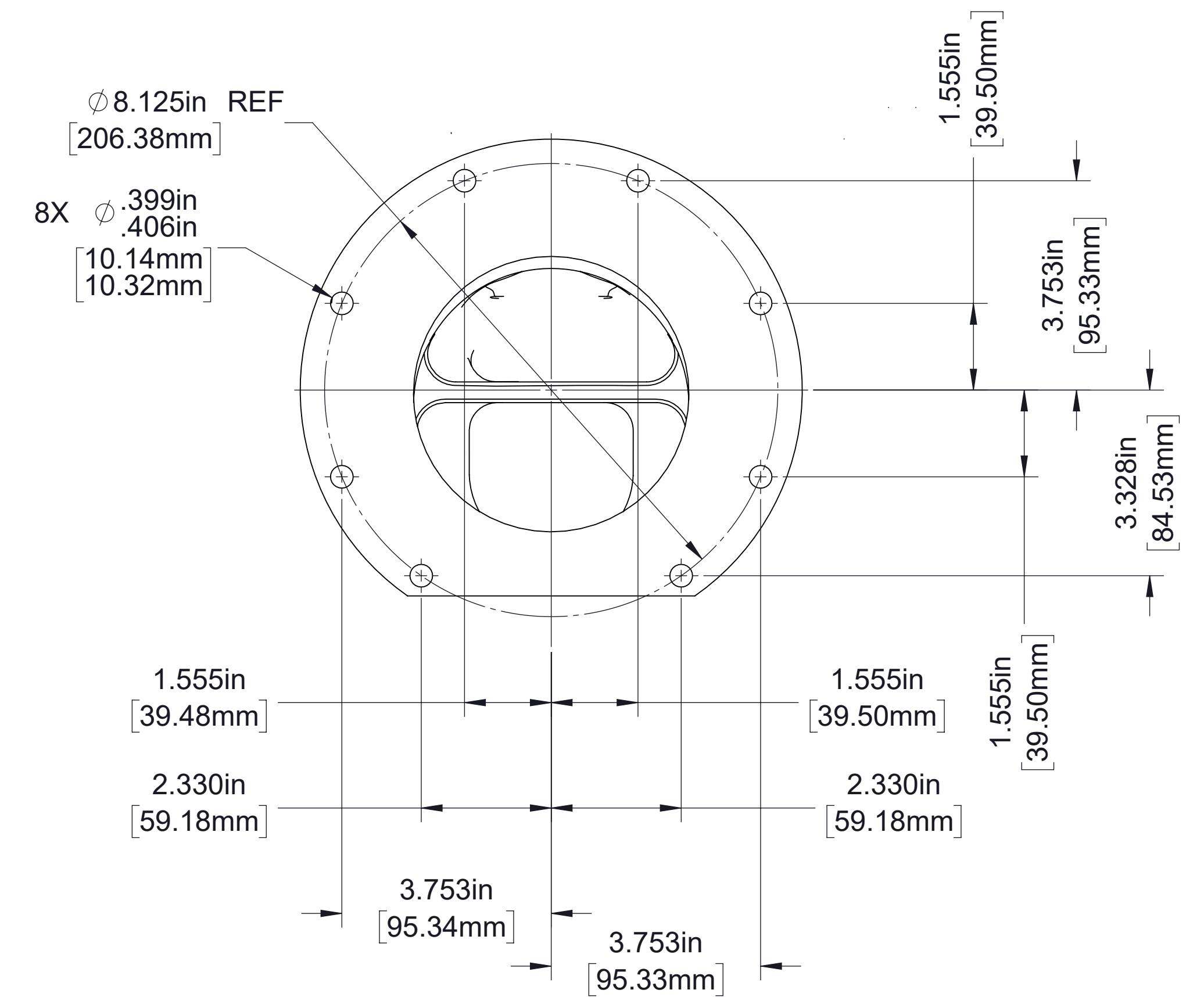
Detail A Discharge Flange (See Page 4 For Optional 5in Victaulic Discharge Adapter)
