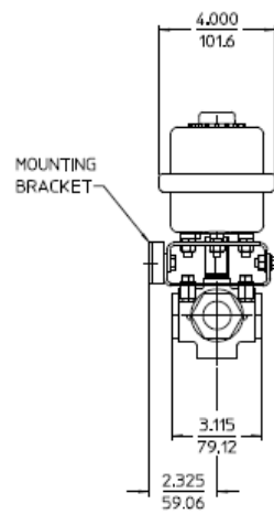
ELECTRIC VALVE
