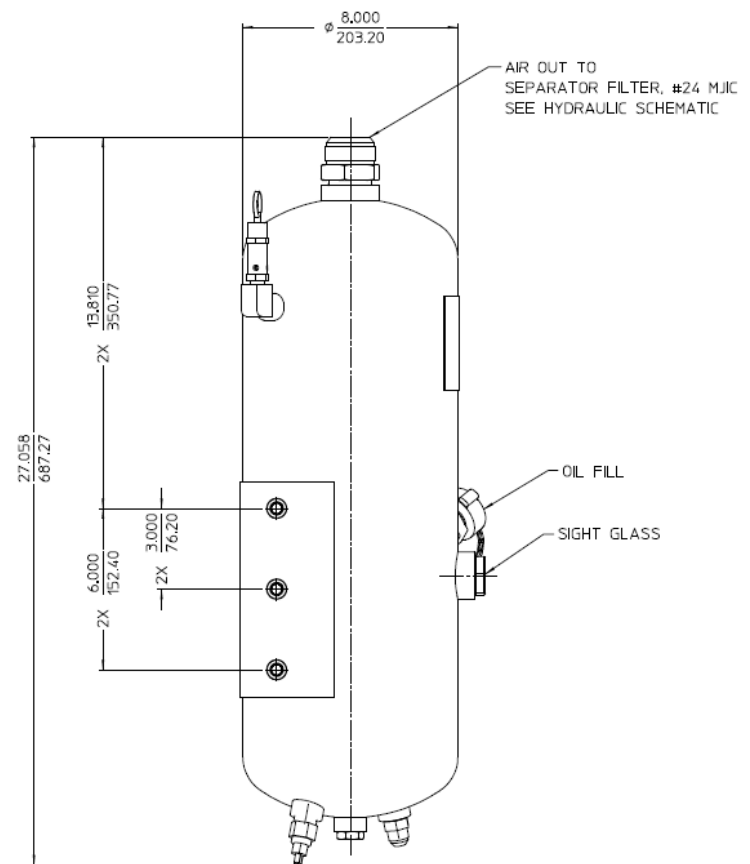
140-P SUMP (OIL RESERVIOR)
