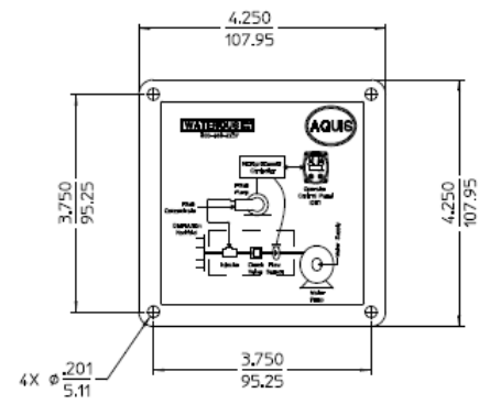
OPTIONAL SCHEMATIC PANEL PLATE
