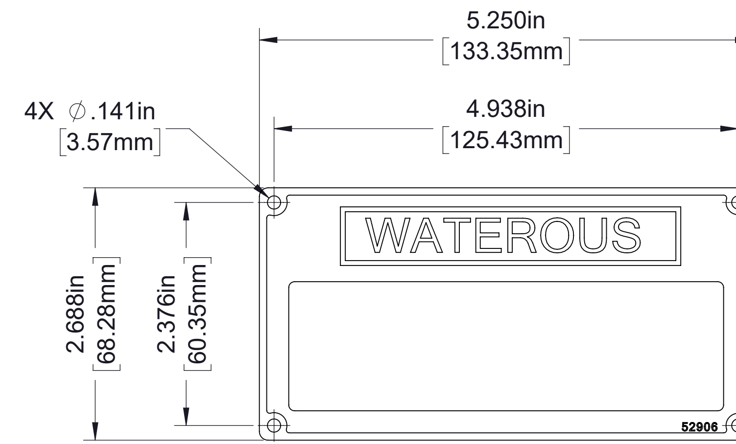
Serial Plate
