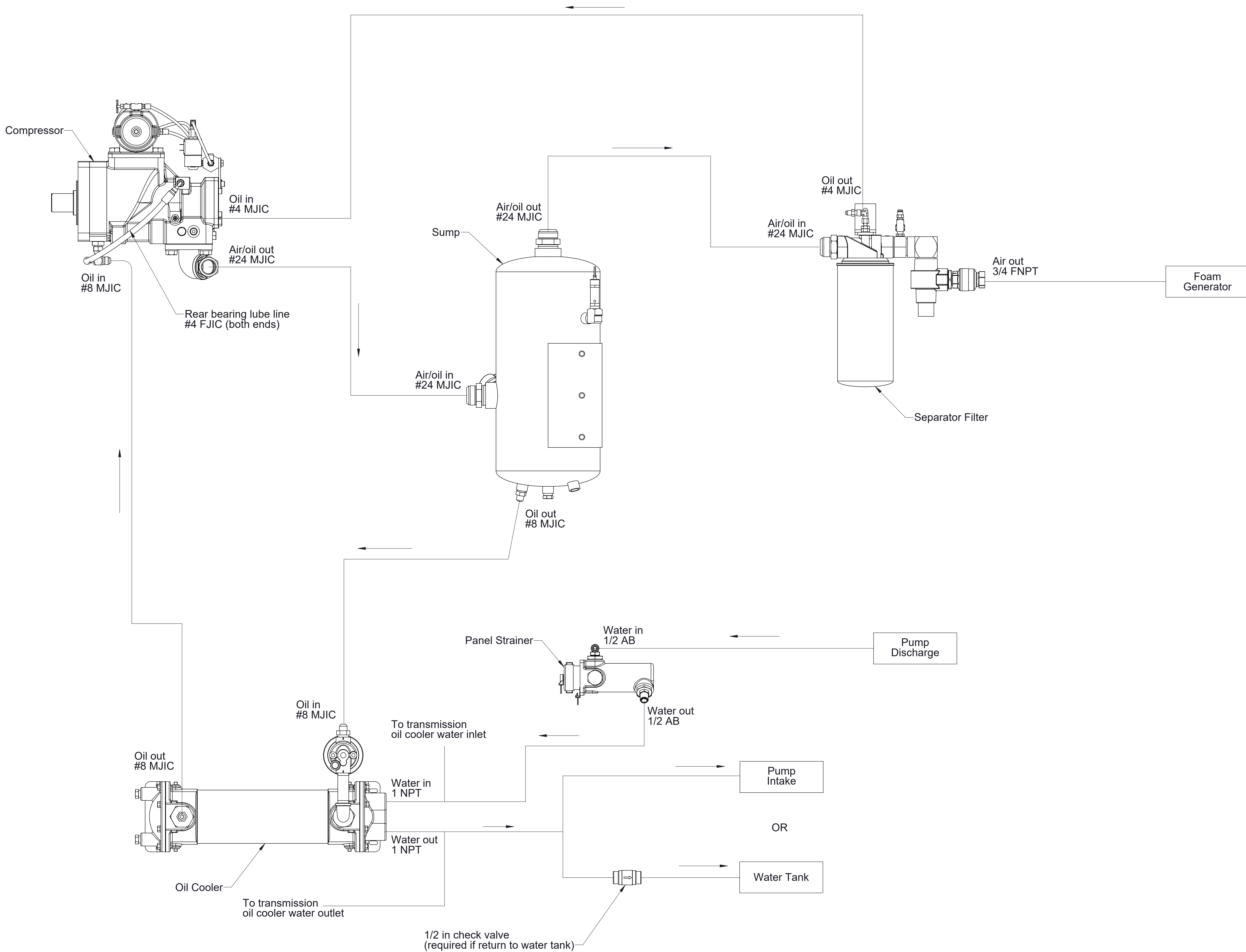
Hydraulic Schematic
