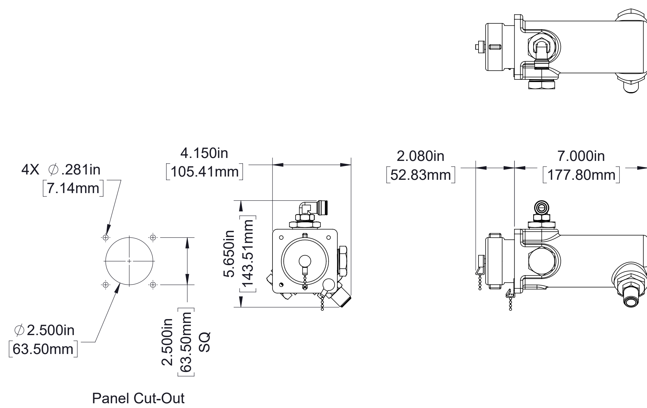
Panel Mounted Strainer
