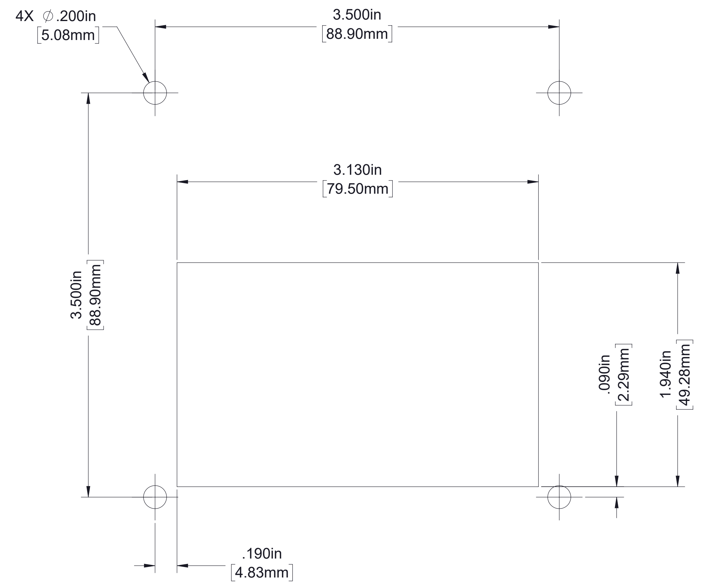
Panel Hole Cutout
