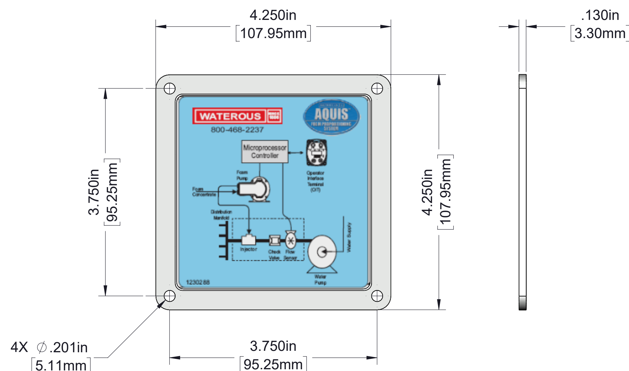
System Schematic Panel Plate (all models)
