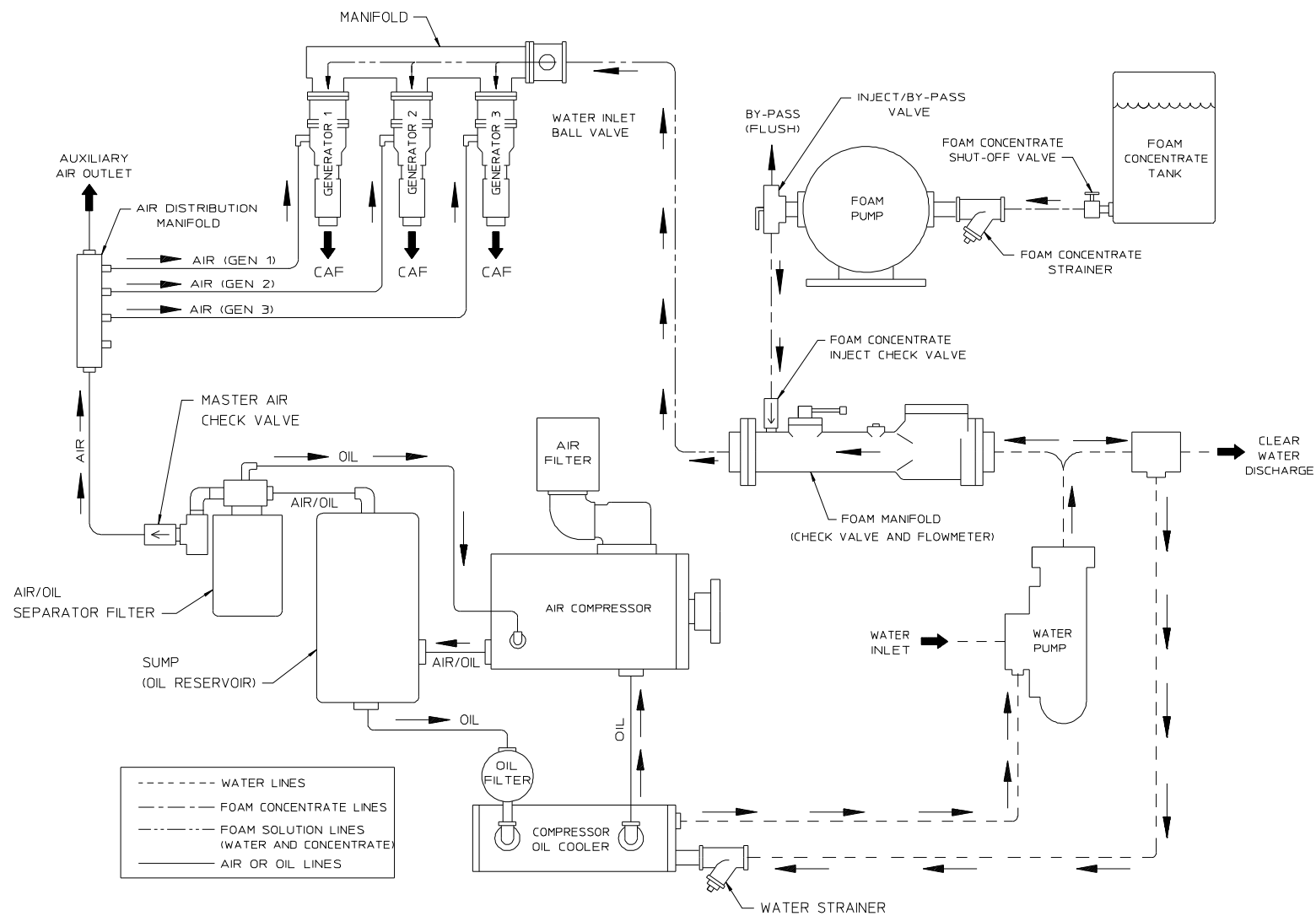
SYSTEM SCHEMATIC
