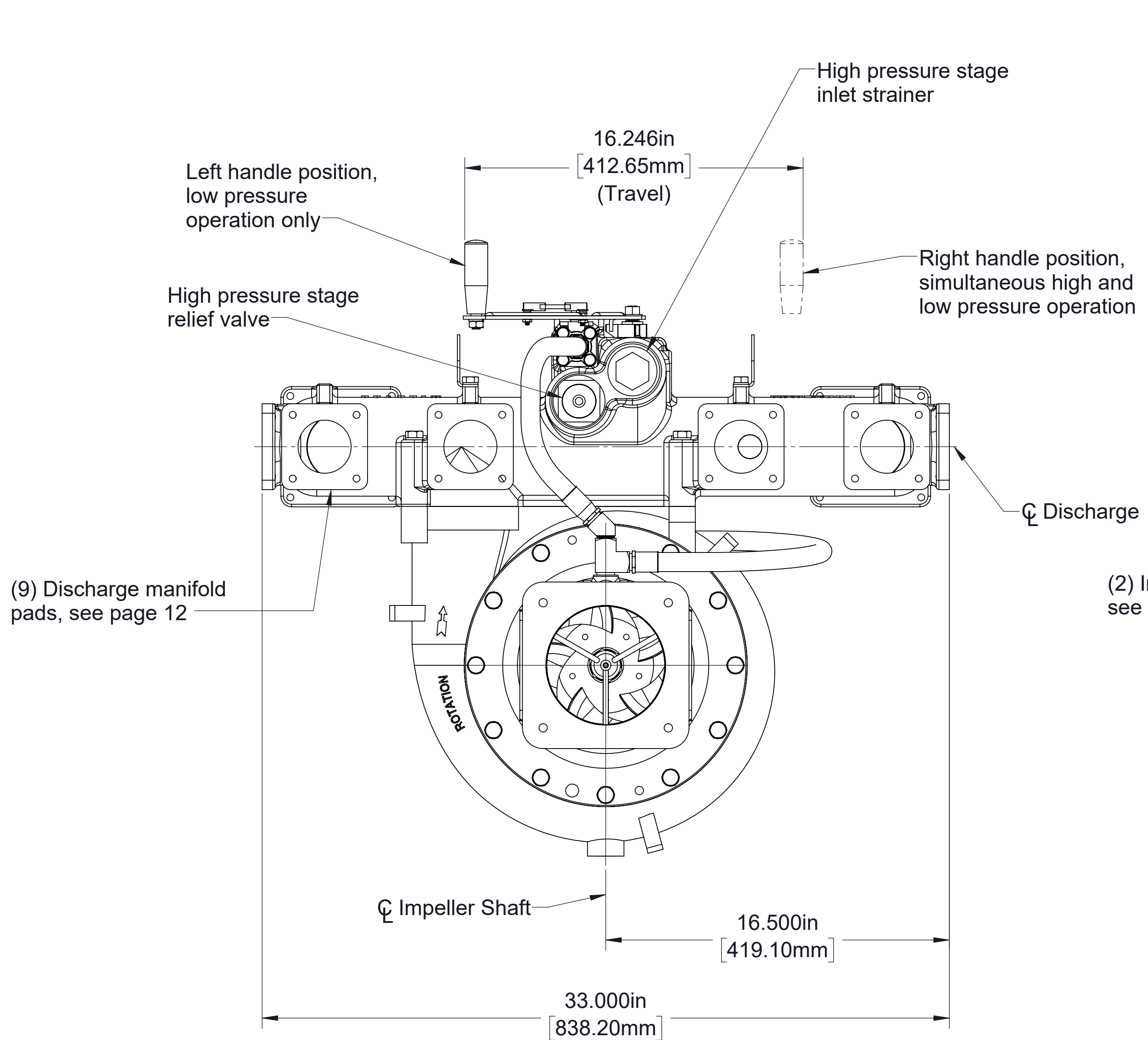
HLUD Pump with Manual Crossover Valve Actuator Counter-Clockwise Input Rotation
