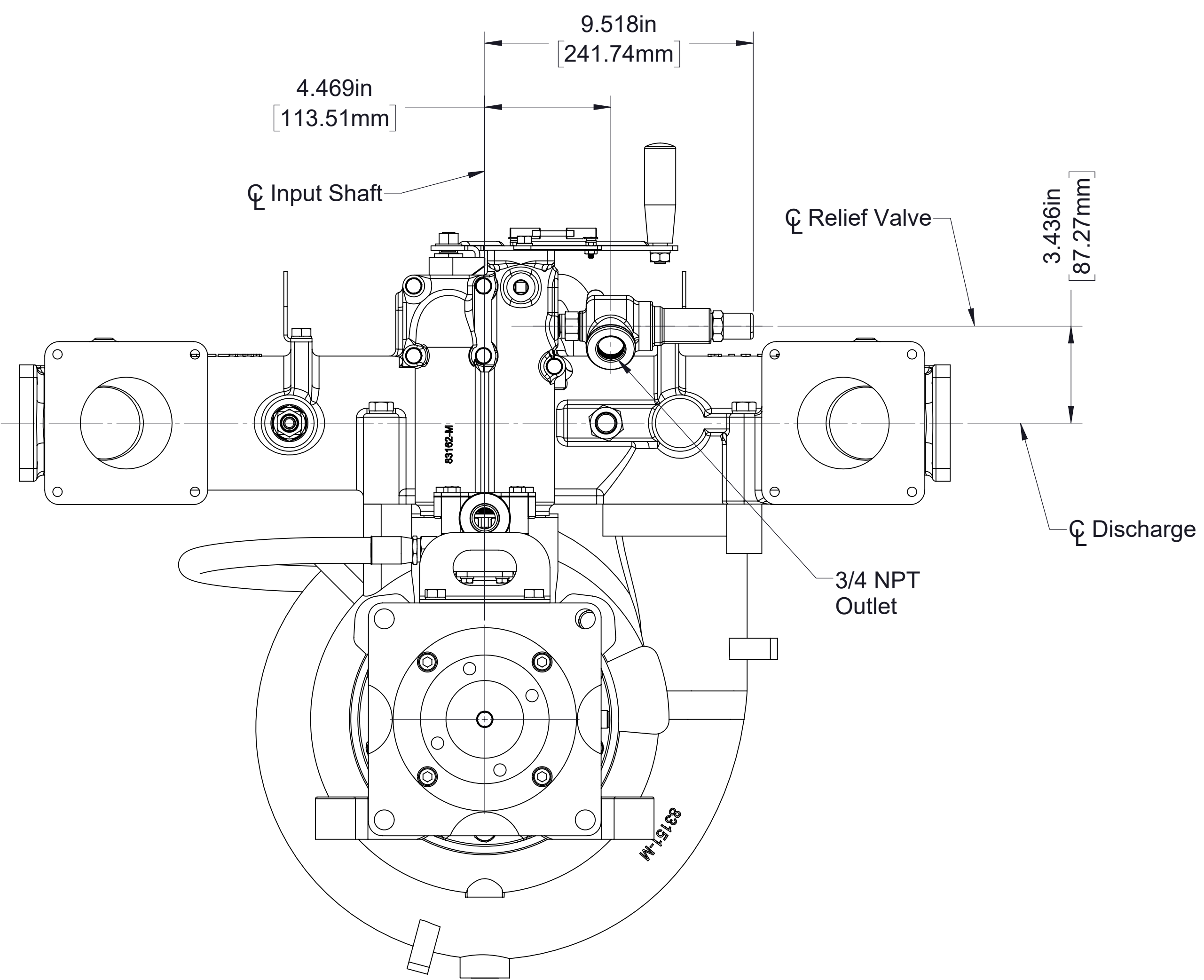
External High Pressure Relief Valve
