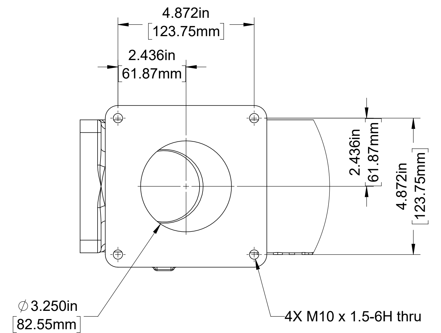
View D-D
