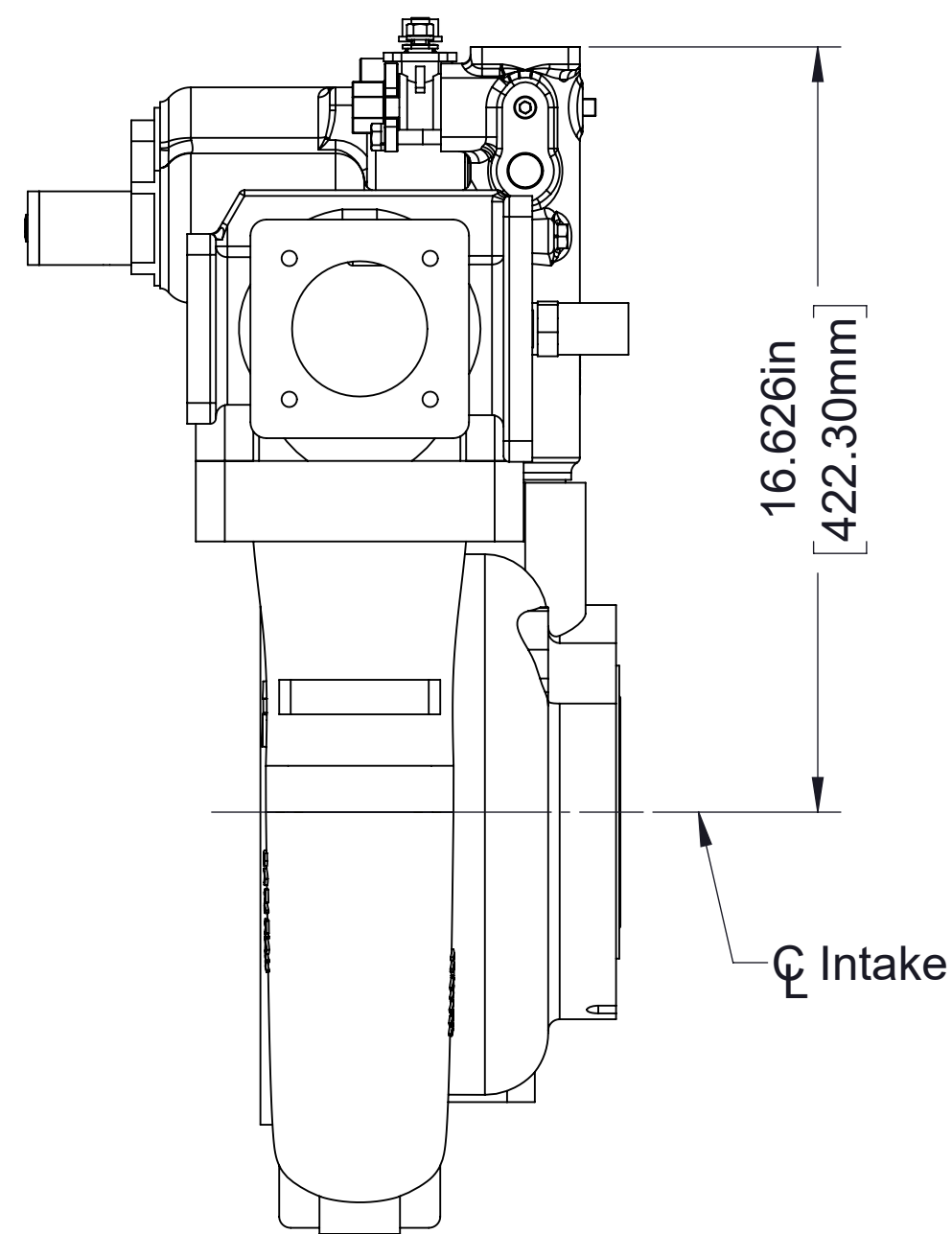
Discharge Manifold
