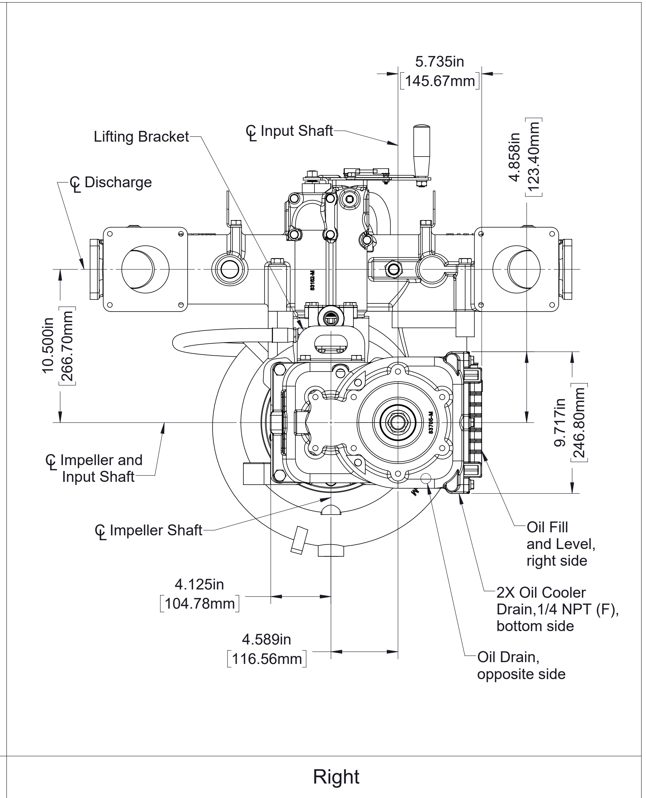
Horizontal
