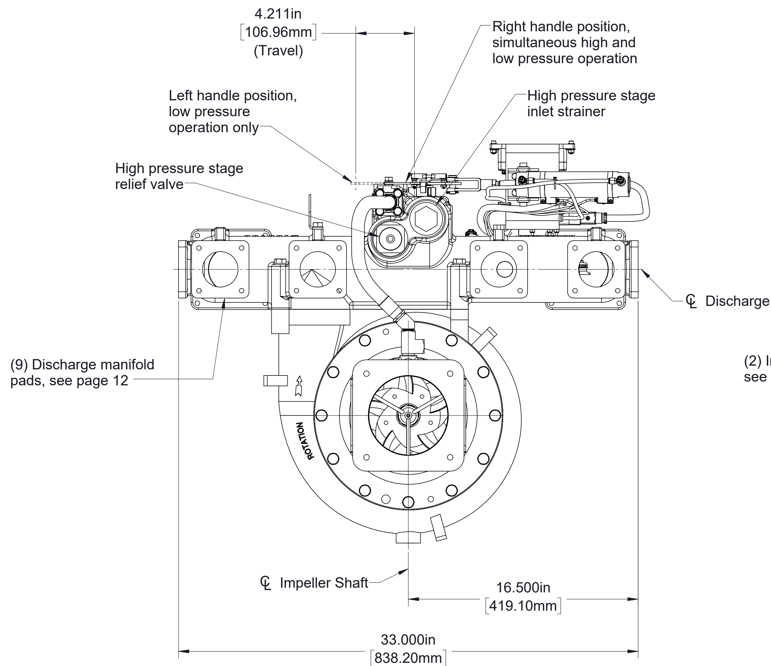
HLUD Pump with Pneumatic Crossover Valve Actuator Counter-Clockwise Input Rotation
