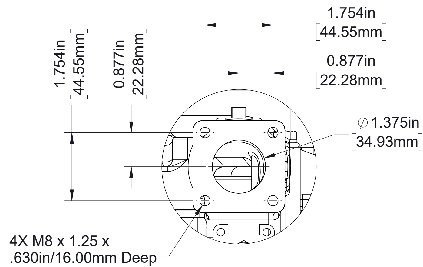
Detail B
