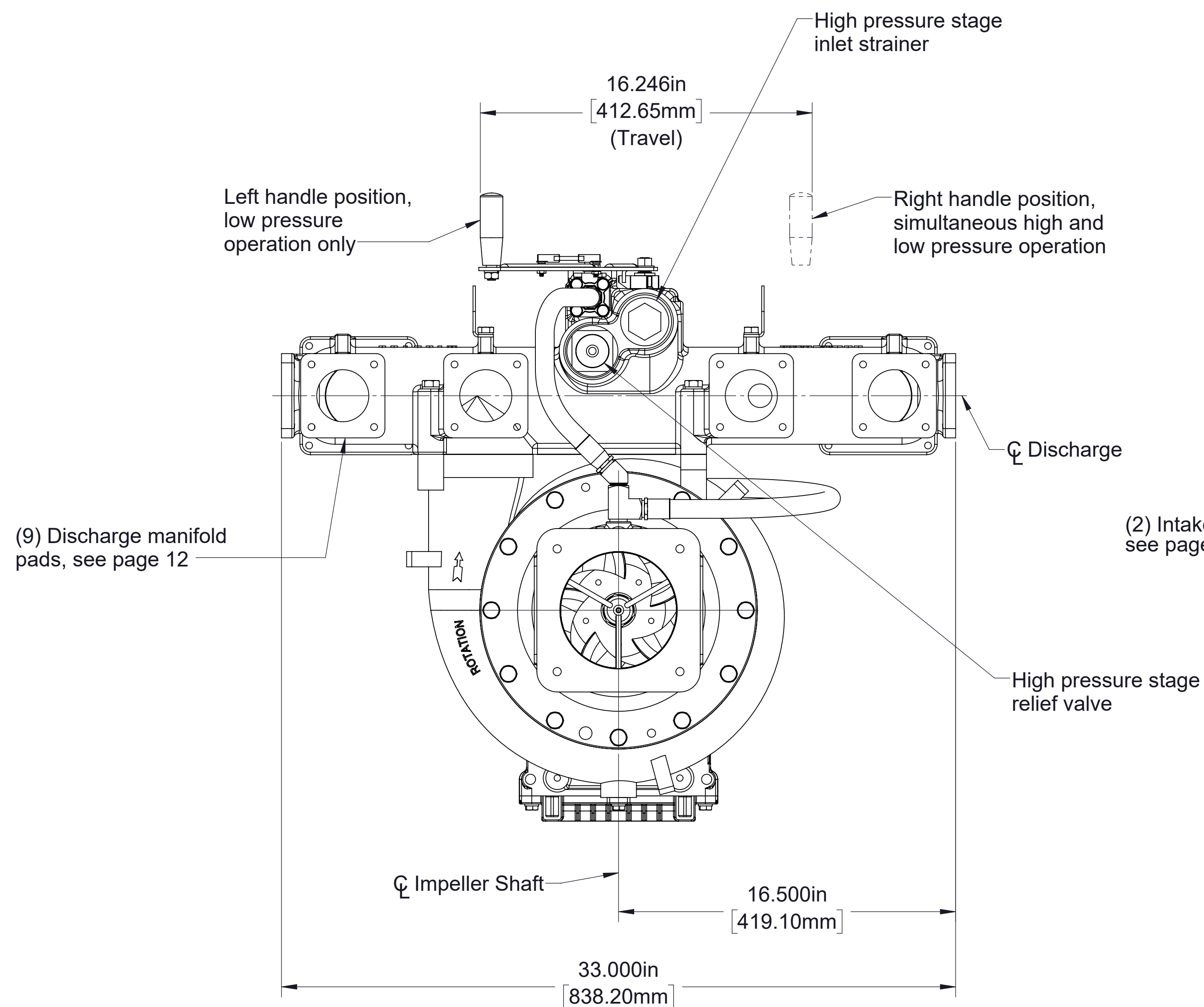
HLUK Pump with Manual Crossover Valve Actuator Clockwise Input Rotation
