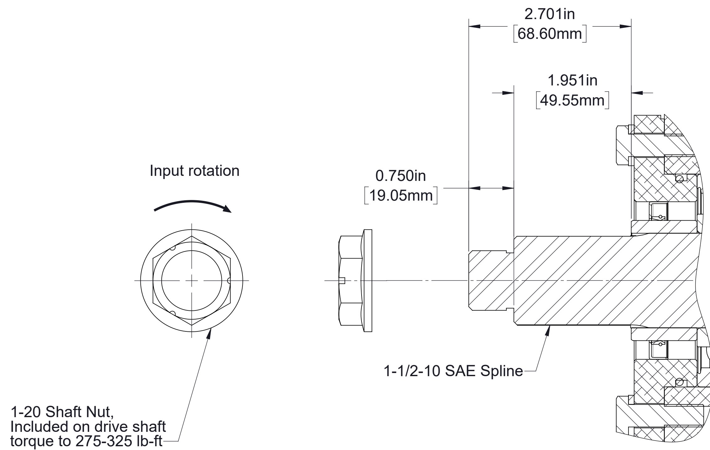
Input Shaft Detail
