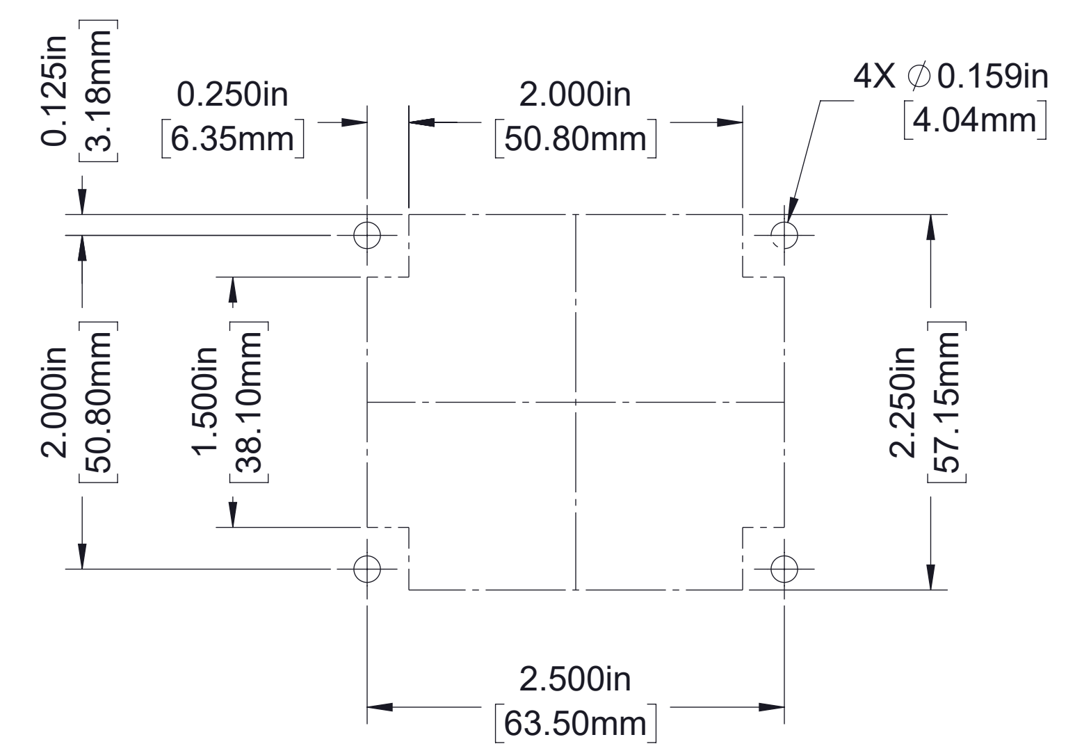
Panel Hole Layout
