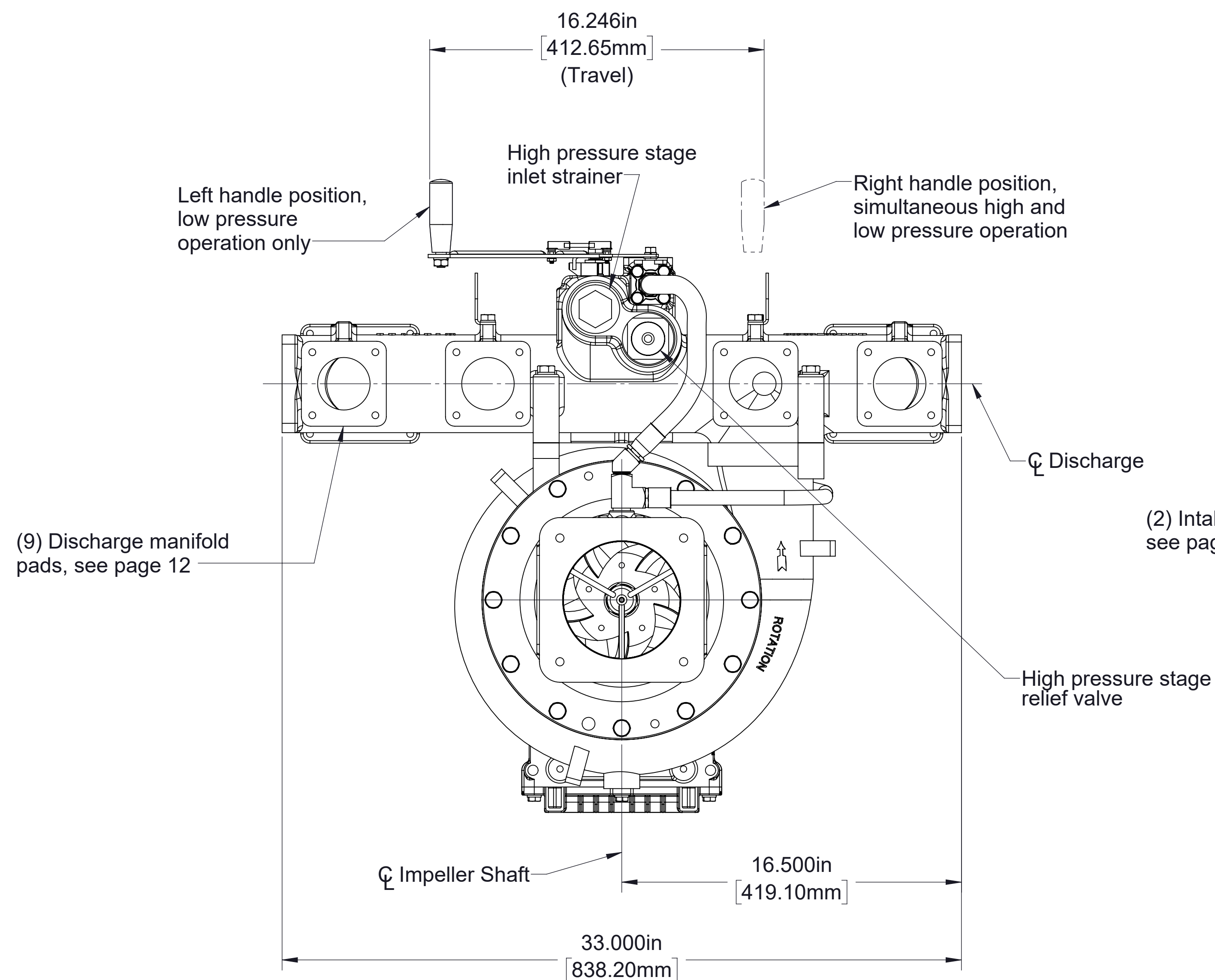
HLUK Pump with Manual Crossover Valve Actuator Counter-Clockwise Input Rotation
