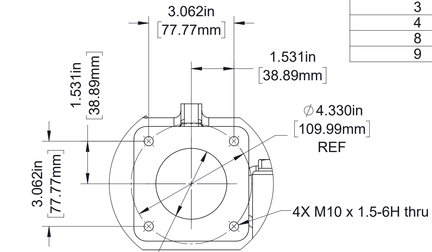
Detail C
