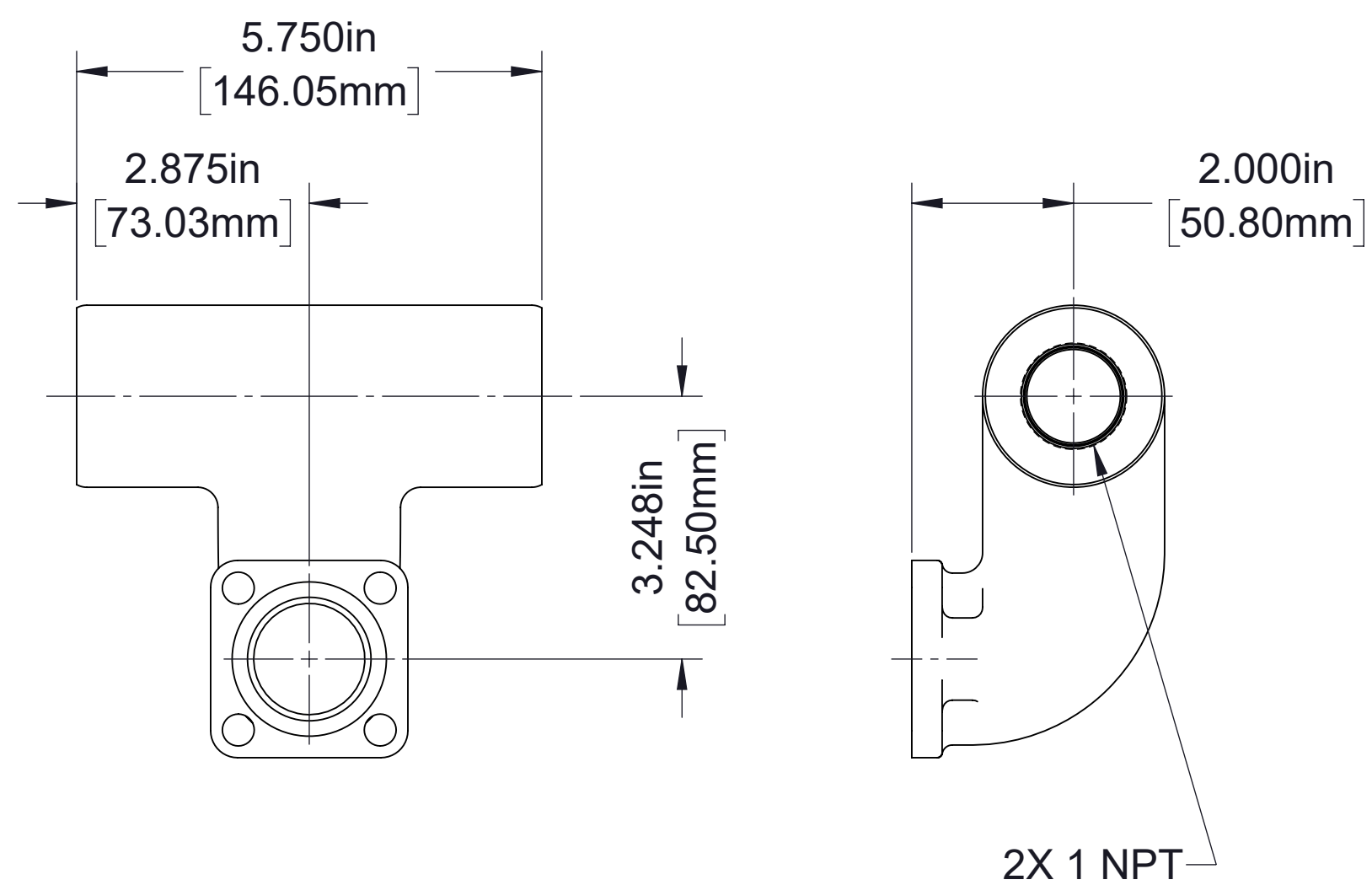
Manifold
