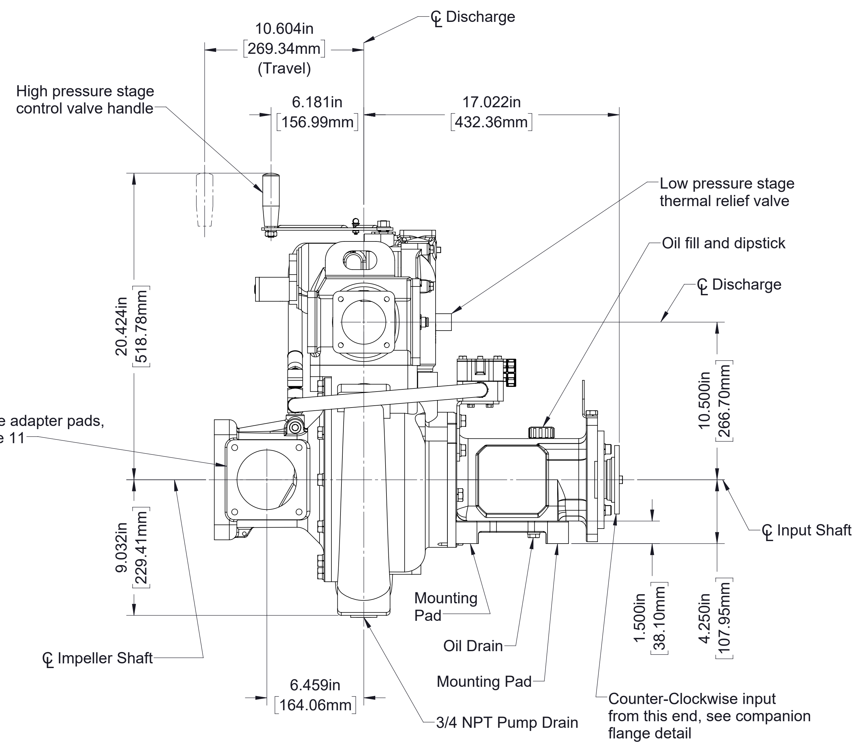
HLUD Pump with Manual Crossover Valve Actuator Counter-Clockwise Input Rotation
