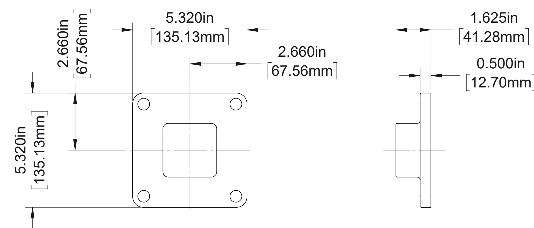
Blind Flange
