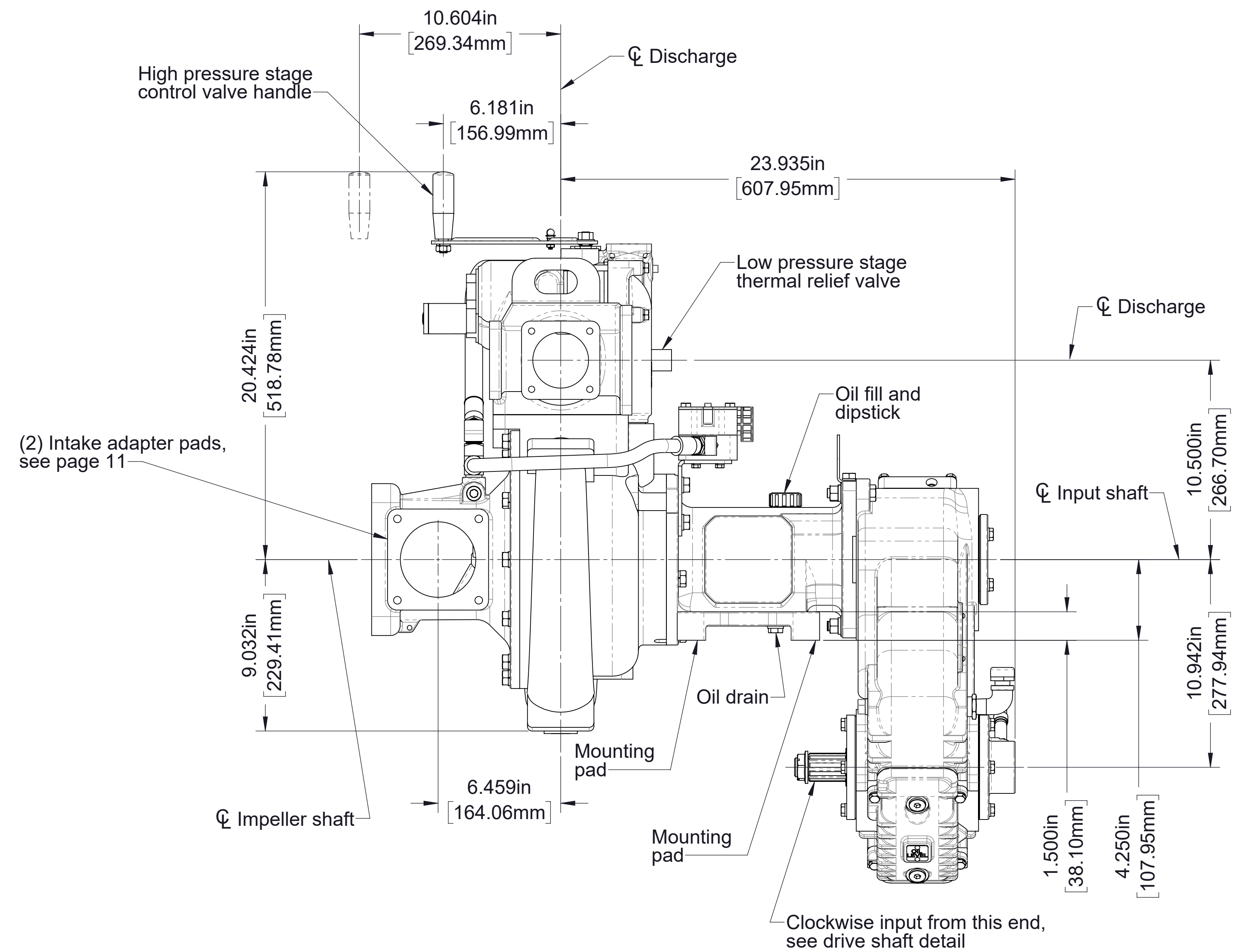
HLUPA Pump with Manual Crossover Valve Actuator Clockwise Input Rotation
