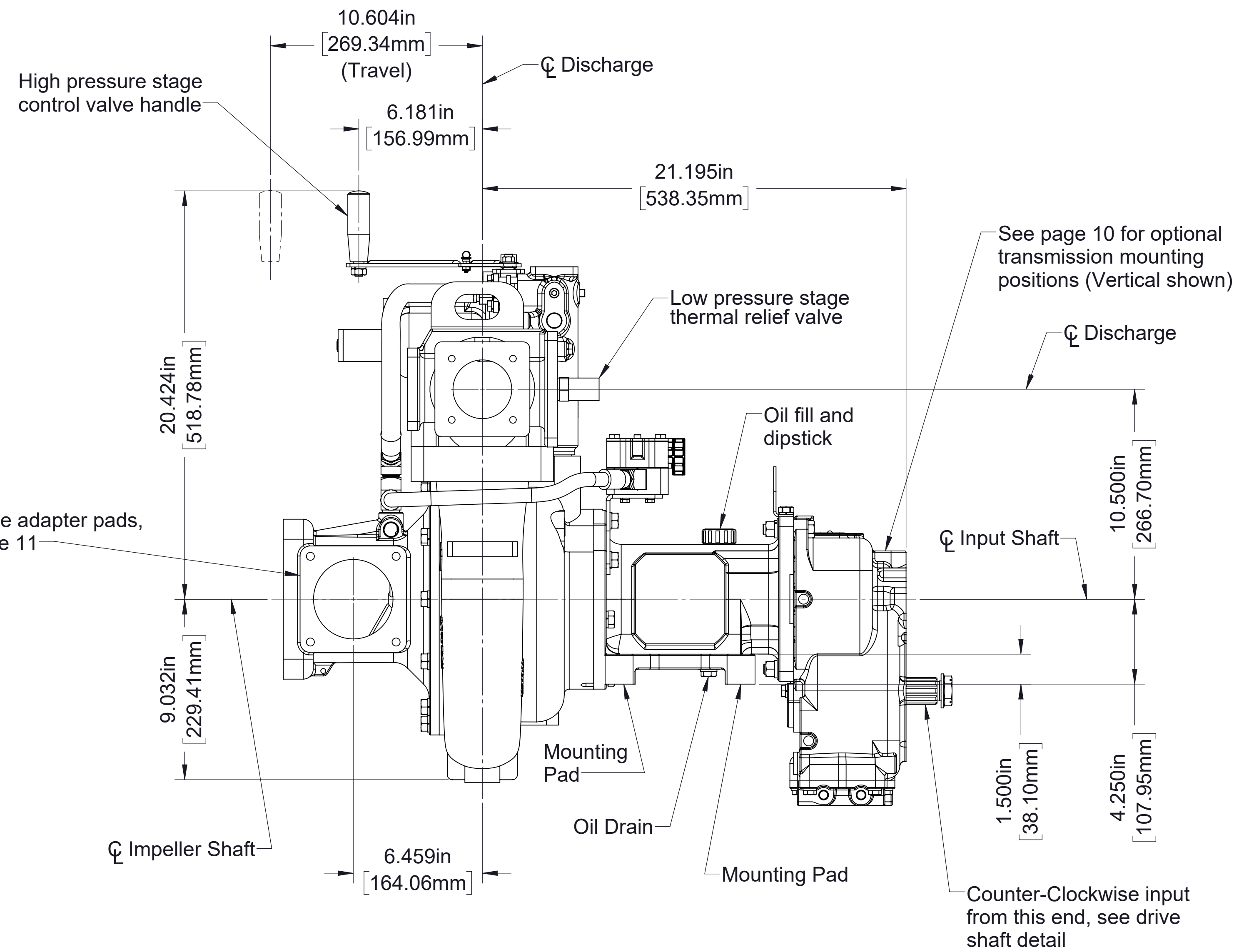
HLUK Pump with Manual Crossover Valve Actuator Counter-Clockwise Input Rotation
