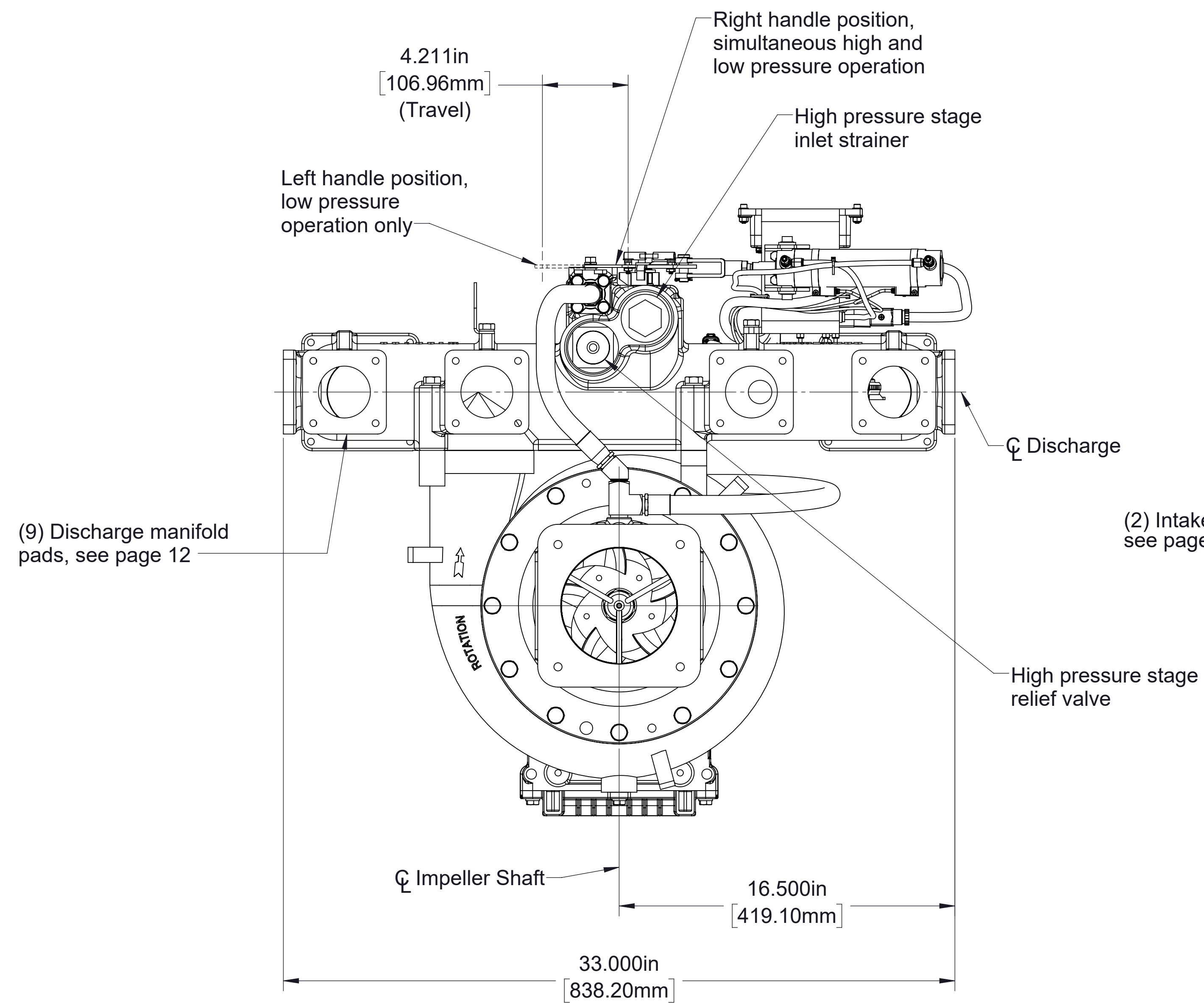
HLUK Pump with Pneumatic Crossover Valve Actuator Clockwise Input Rotation
