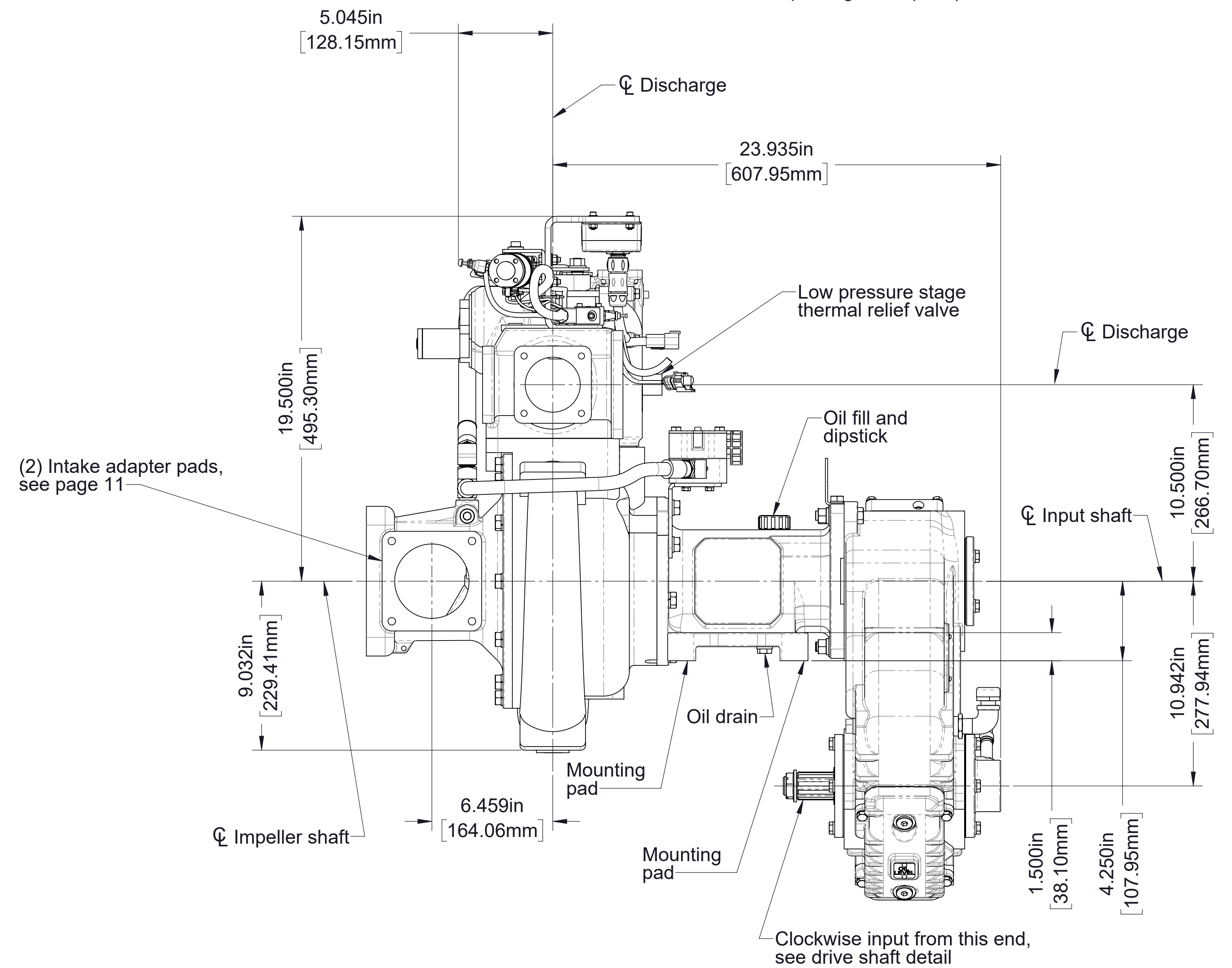
HLUPA Pump with Pneumatic Crossover Valve Actuator Clockwise Input Rotation
