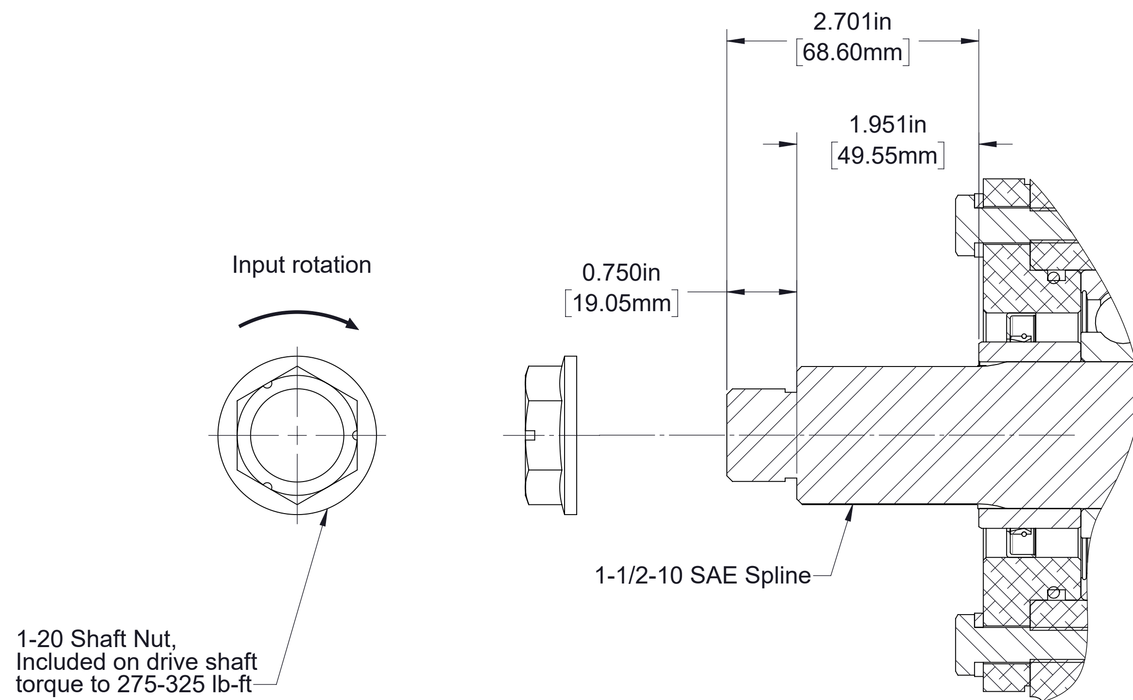
Input Shaft Detail
