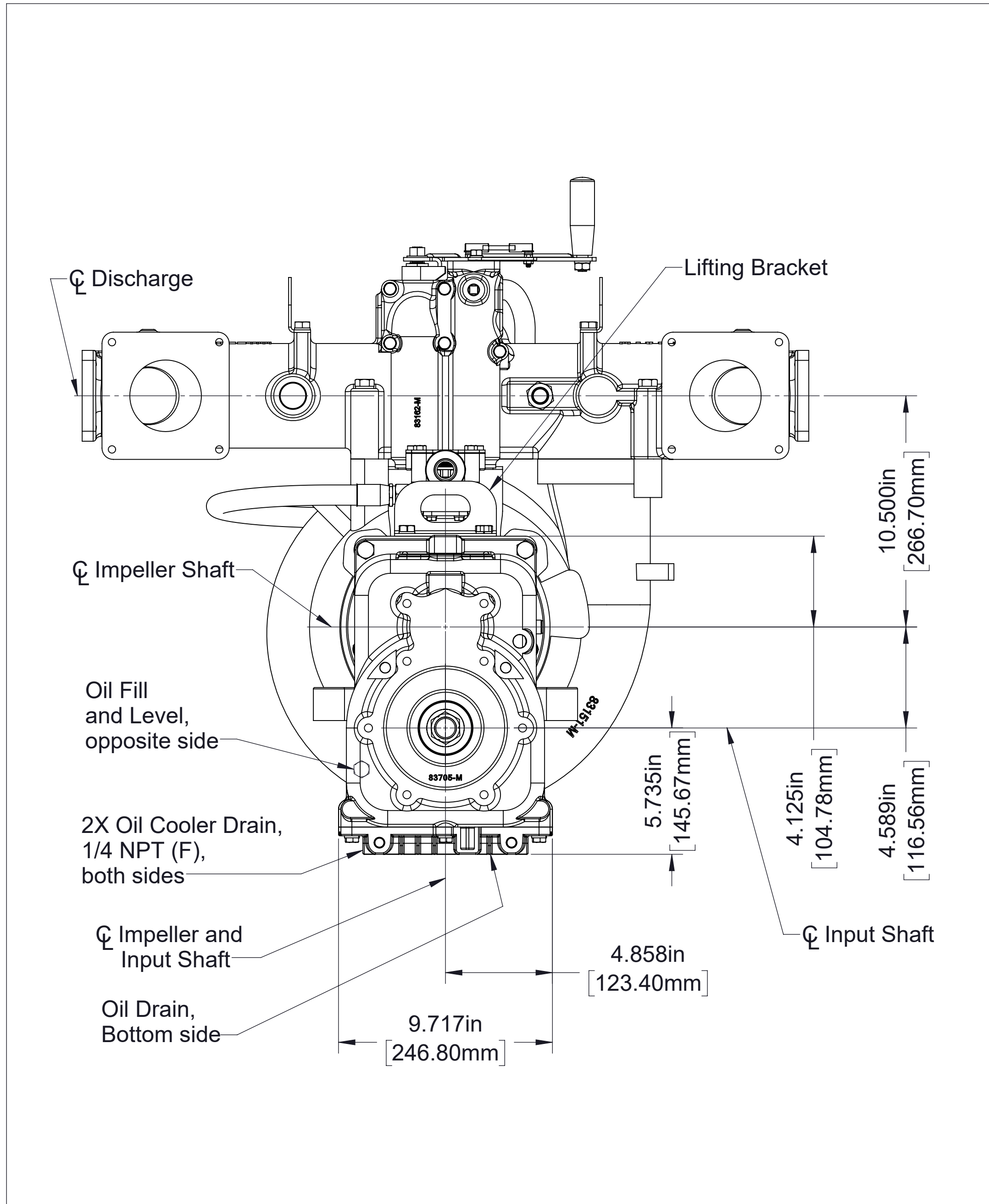
Vertical
