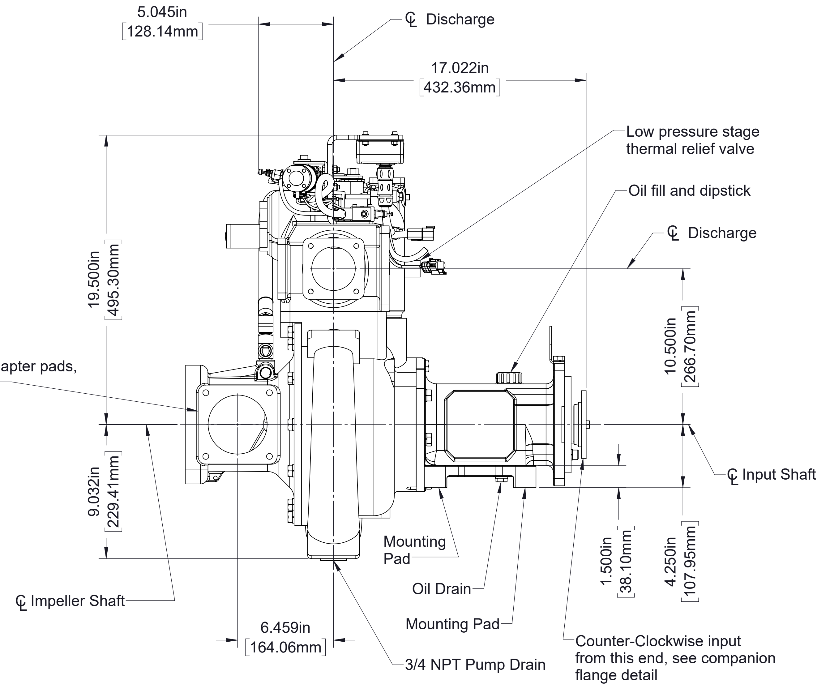
HLUD Pump with Pneumatic Crossover Valve Actuator Counter-Clockwise Input Rotation
