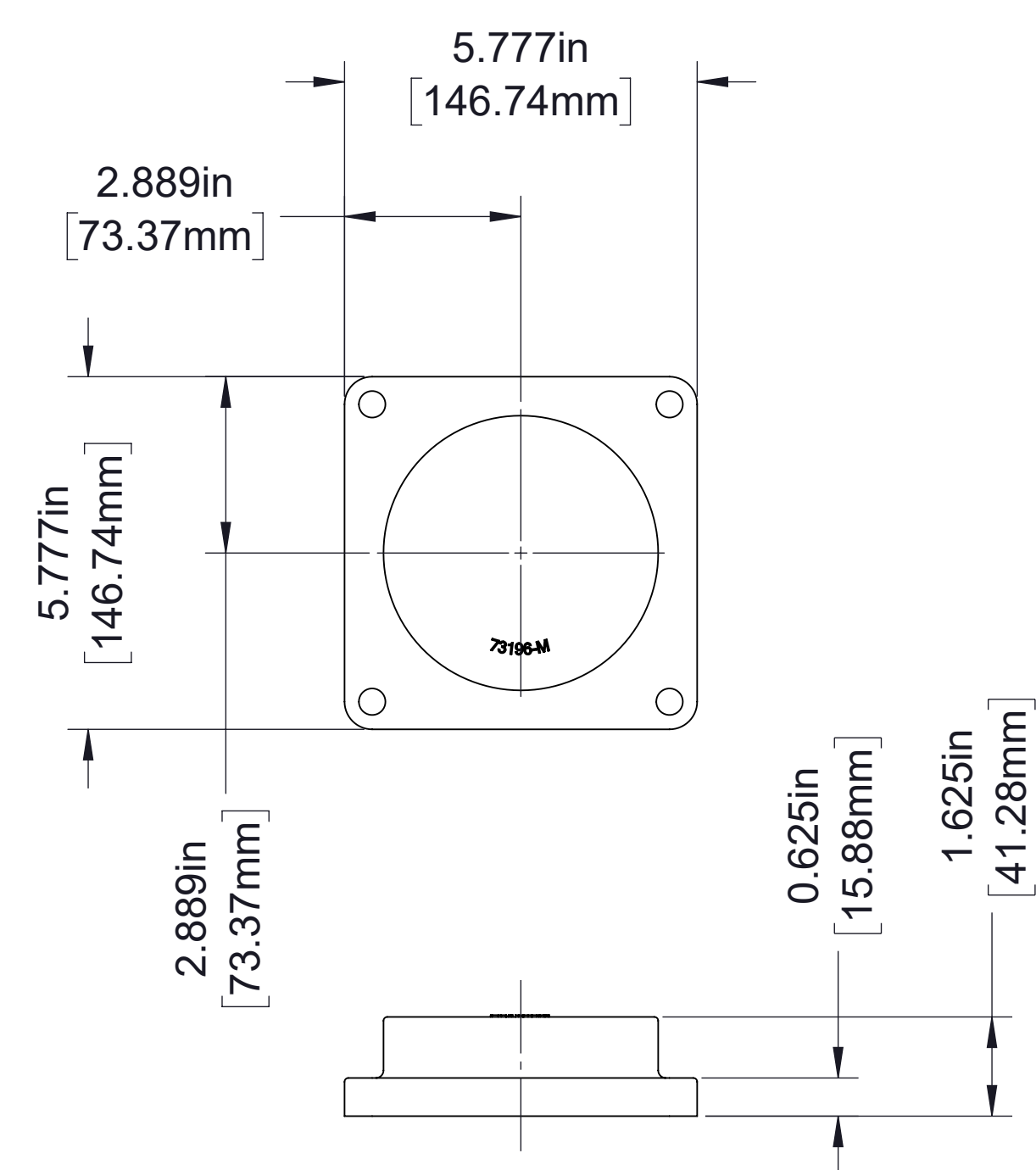
Blind Flange
