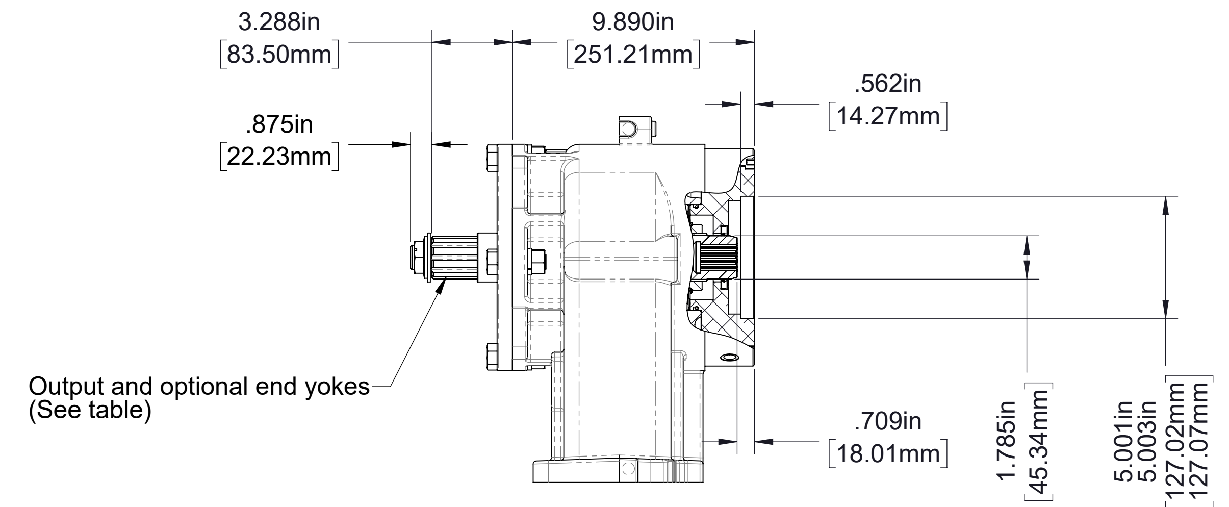
Front Facing End Yoke with Rear Facing SAE Class C, 4-Bolt (Dual)
