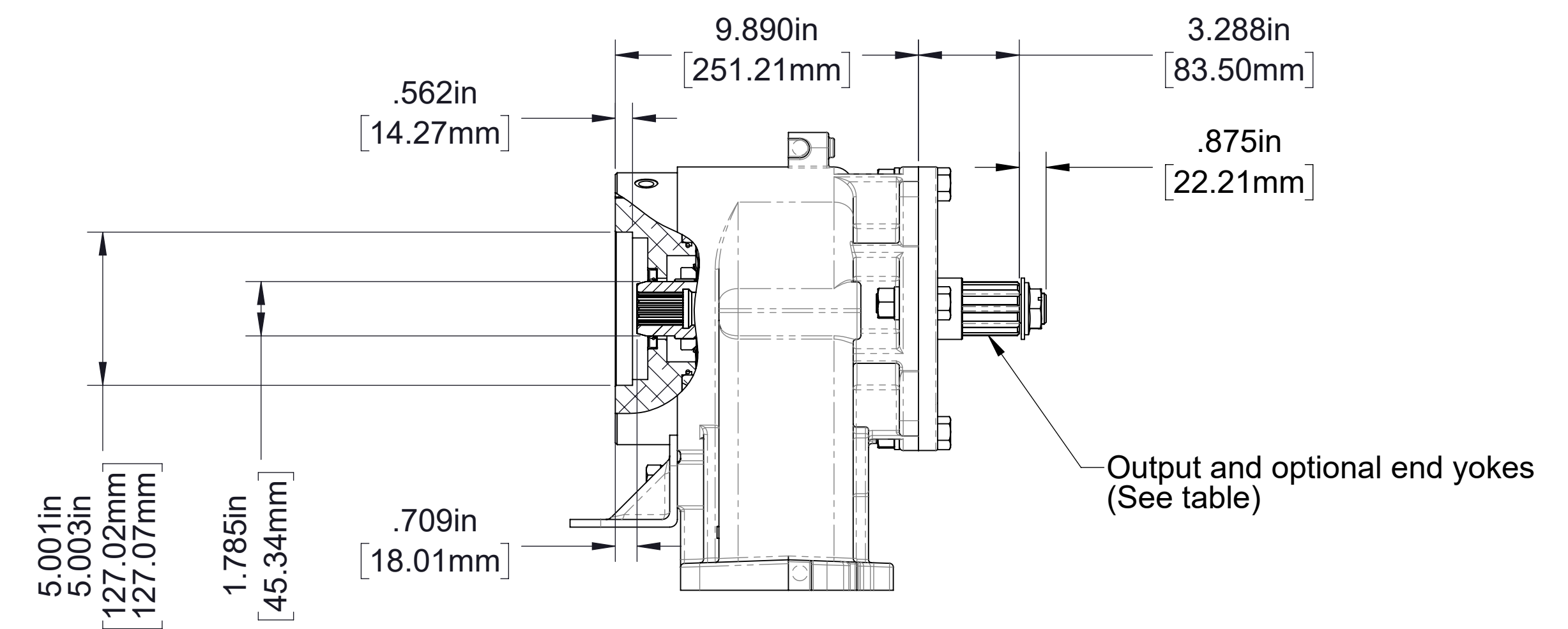
Front Facing SAE Class C, 4-Bolt with Rear Facing End Yoke (Dual)
