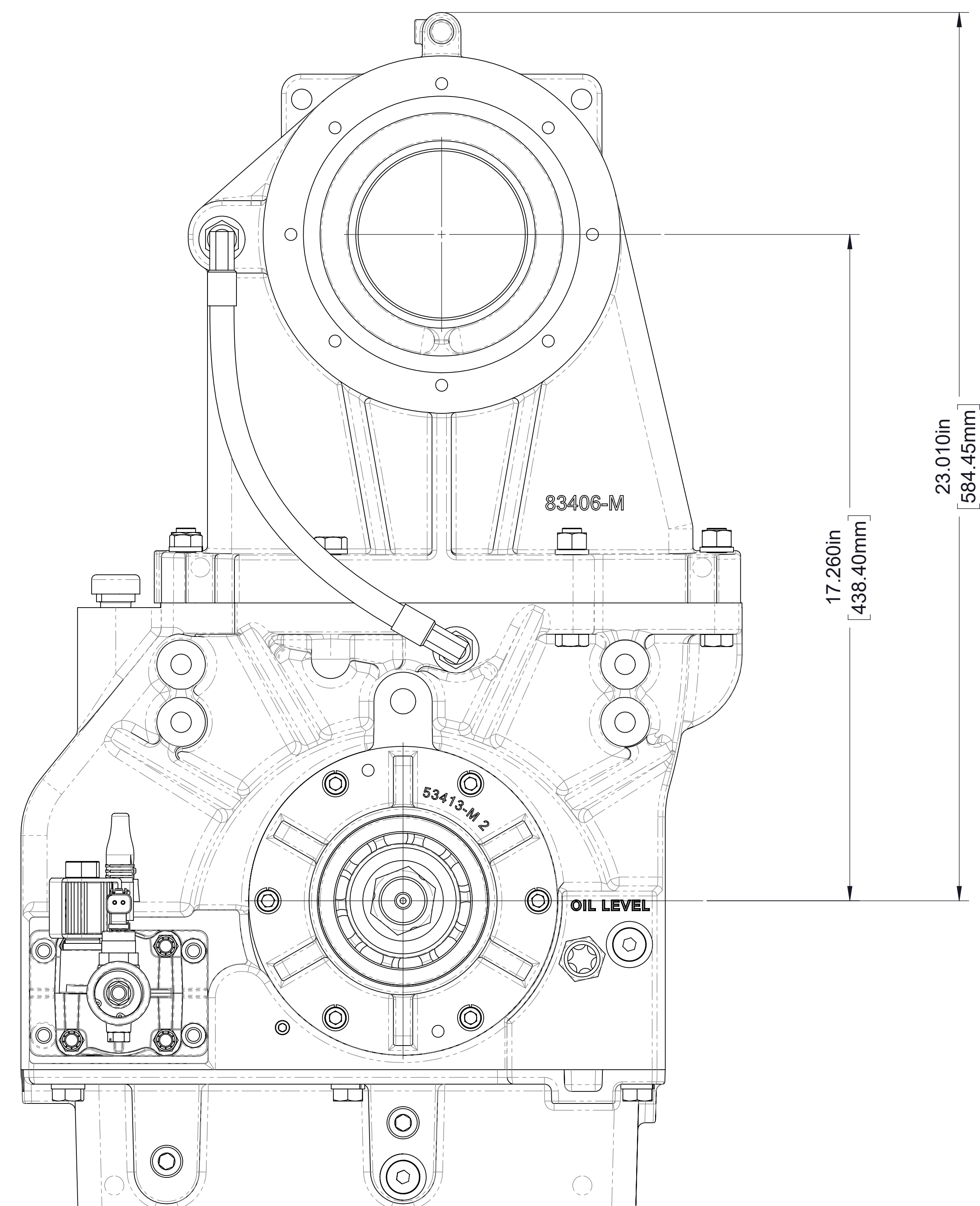
TC23 Model (1.95 ratio)
