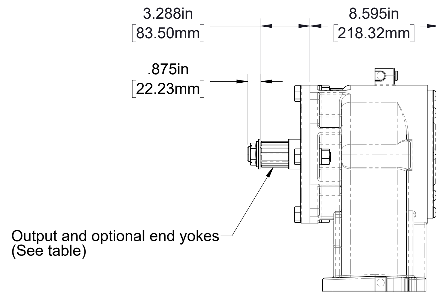
Front Facing End Yoke (Single)
