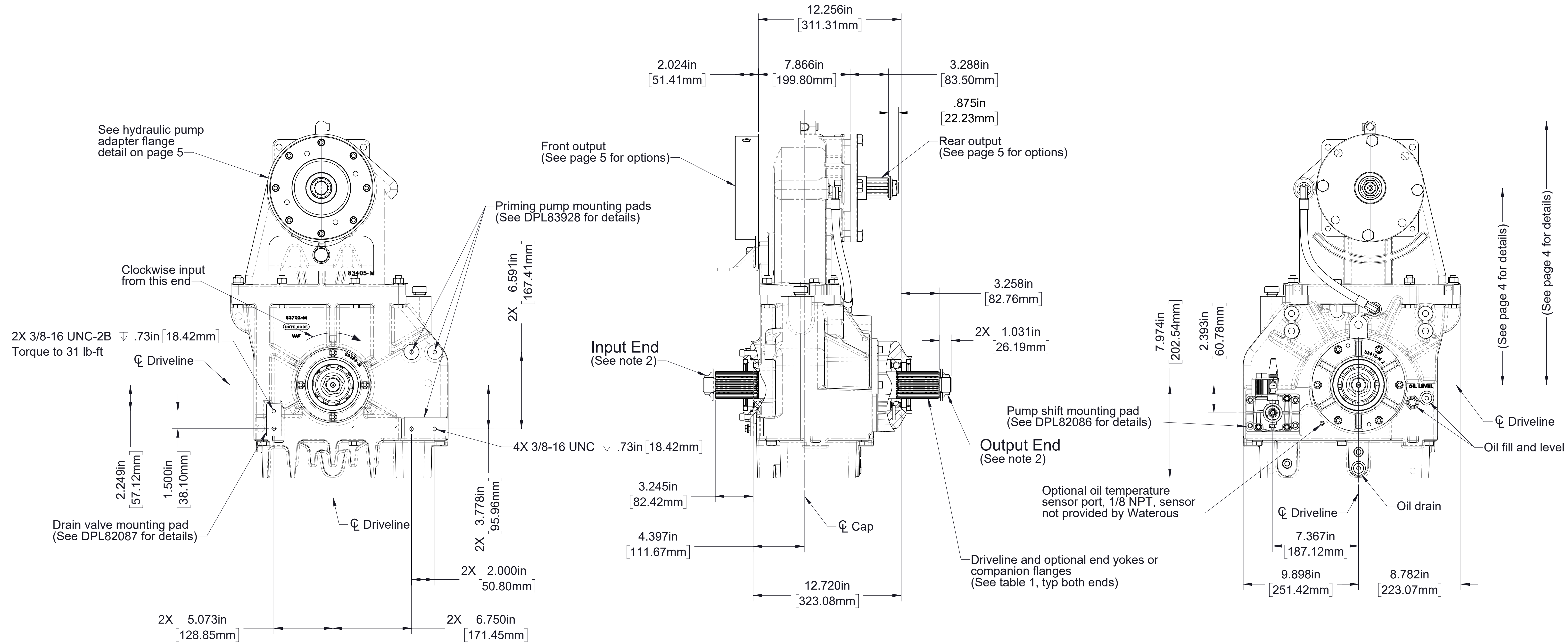
TC23 Models, Input and Output Shaft Split shaft drive, clockwise input (TC23 1.77 ratio shown)
