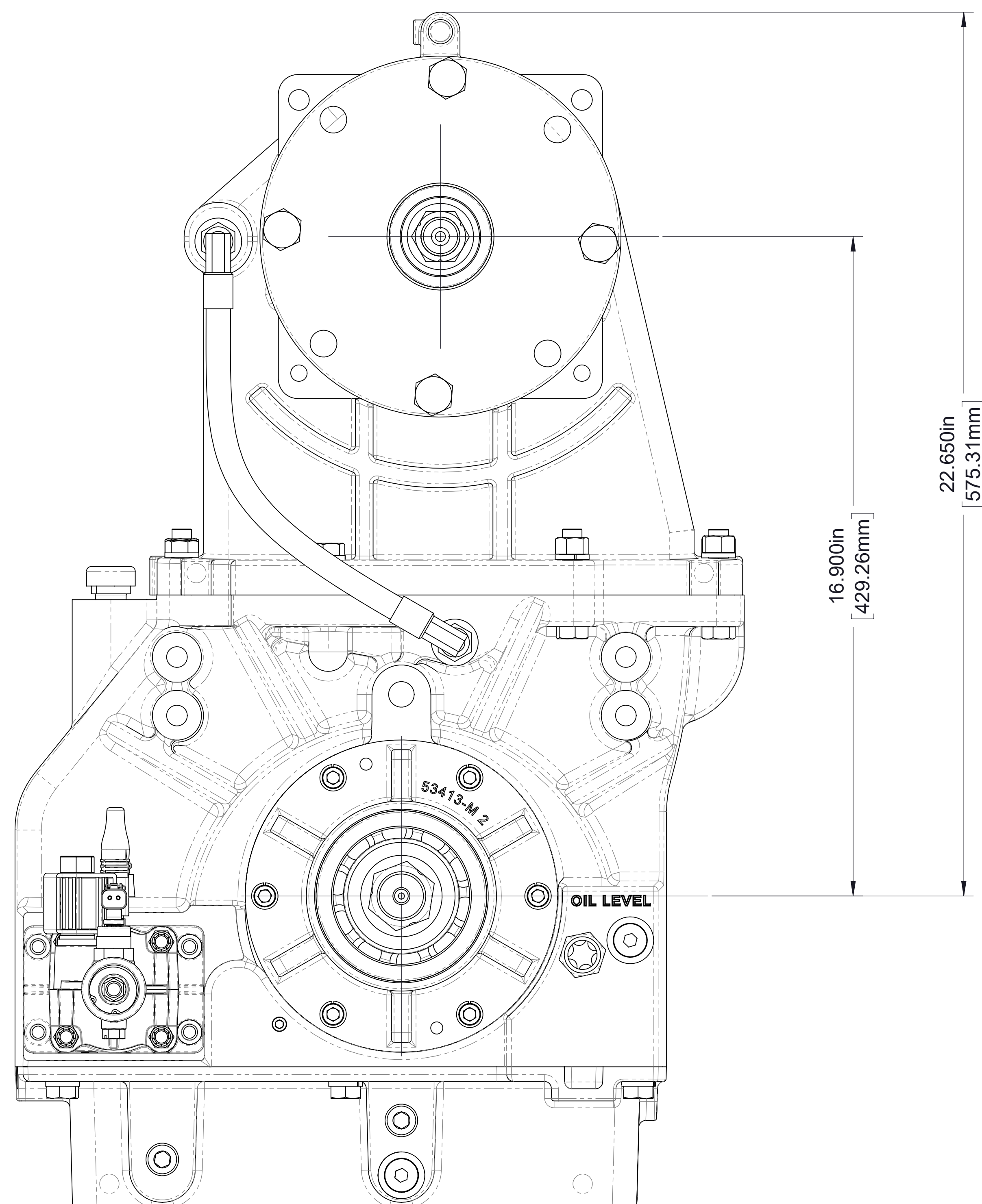
TC23 Model (1.77 ratio)
