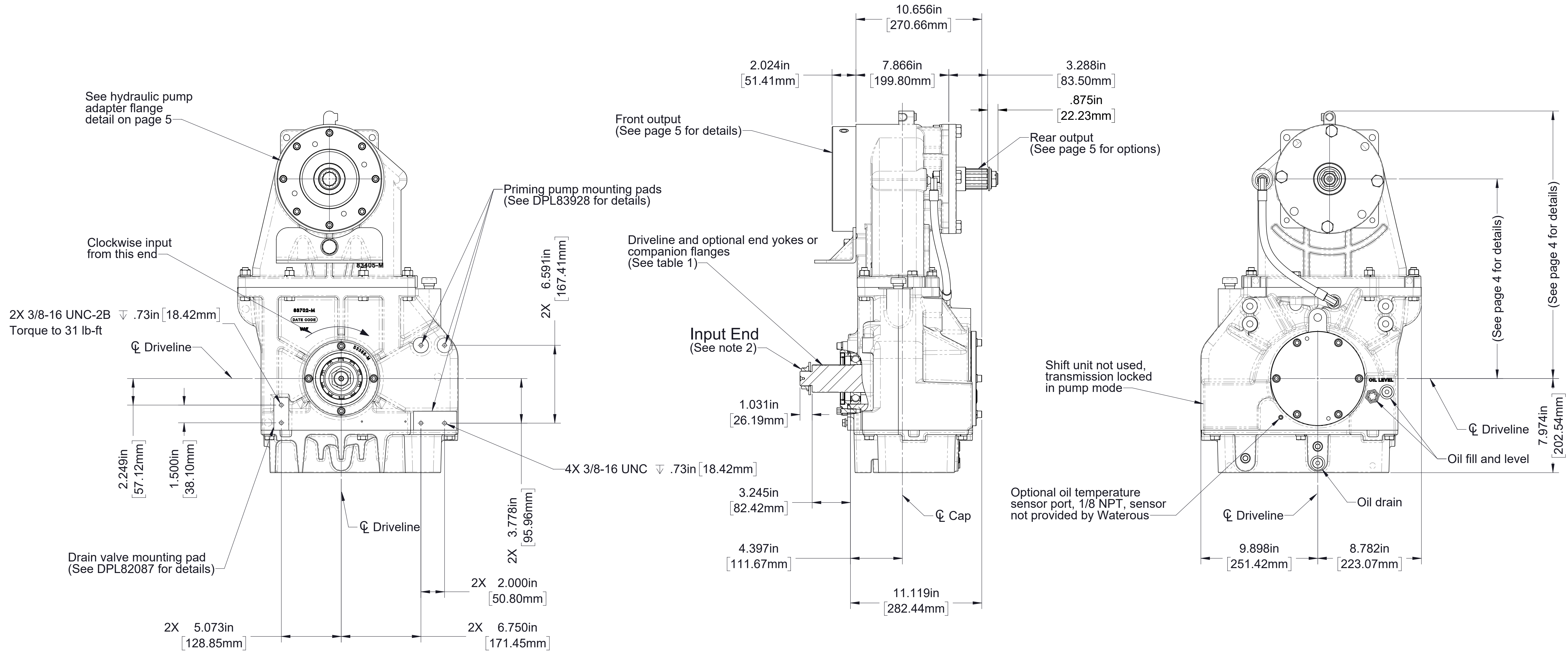
TC23 Models, Input Shaft Only Split shaft drive, clockwise input (TC23 1.77 ratio shown)
