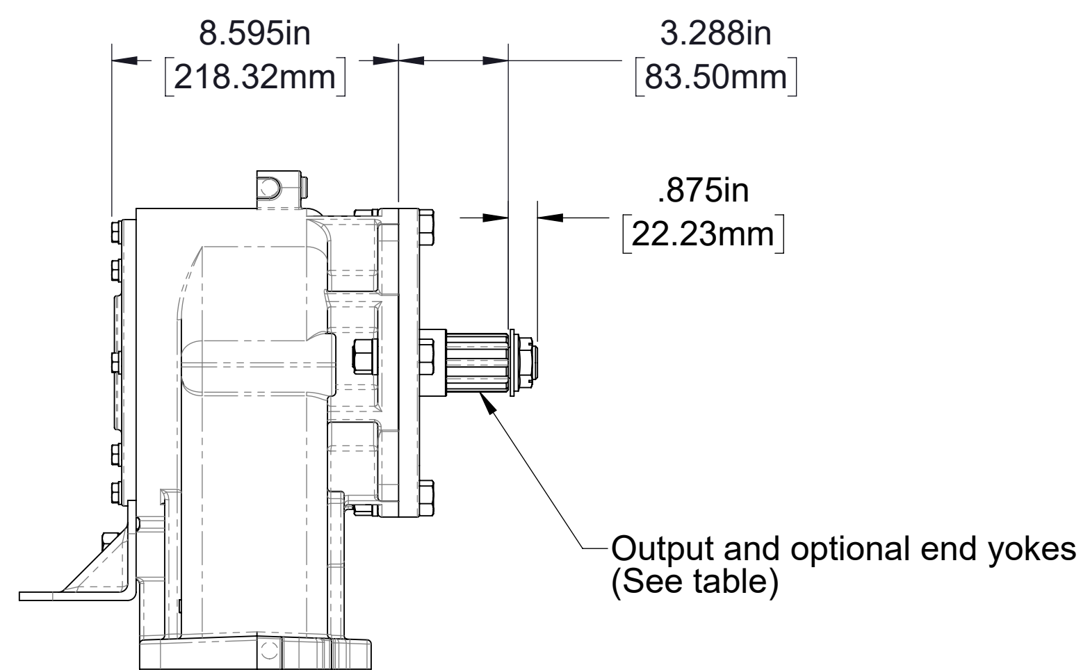
Rear Facing End Yoke (Single)
