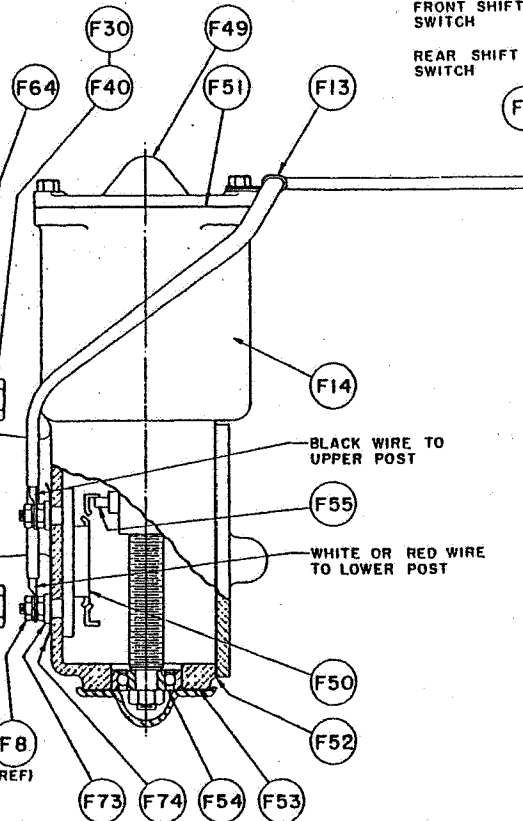
DUAL ELECTRIC SHIFT FIRE PUMP
