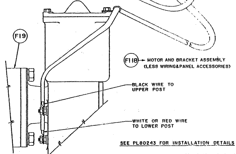
REAR SHIFT UNIT (BRACKET MOUNTED) (SEE PAGE 1 FOR DETAILS)
