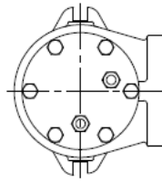
RIGHT FACING DISCHARGE ASSEMBLY 80397-1
