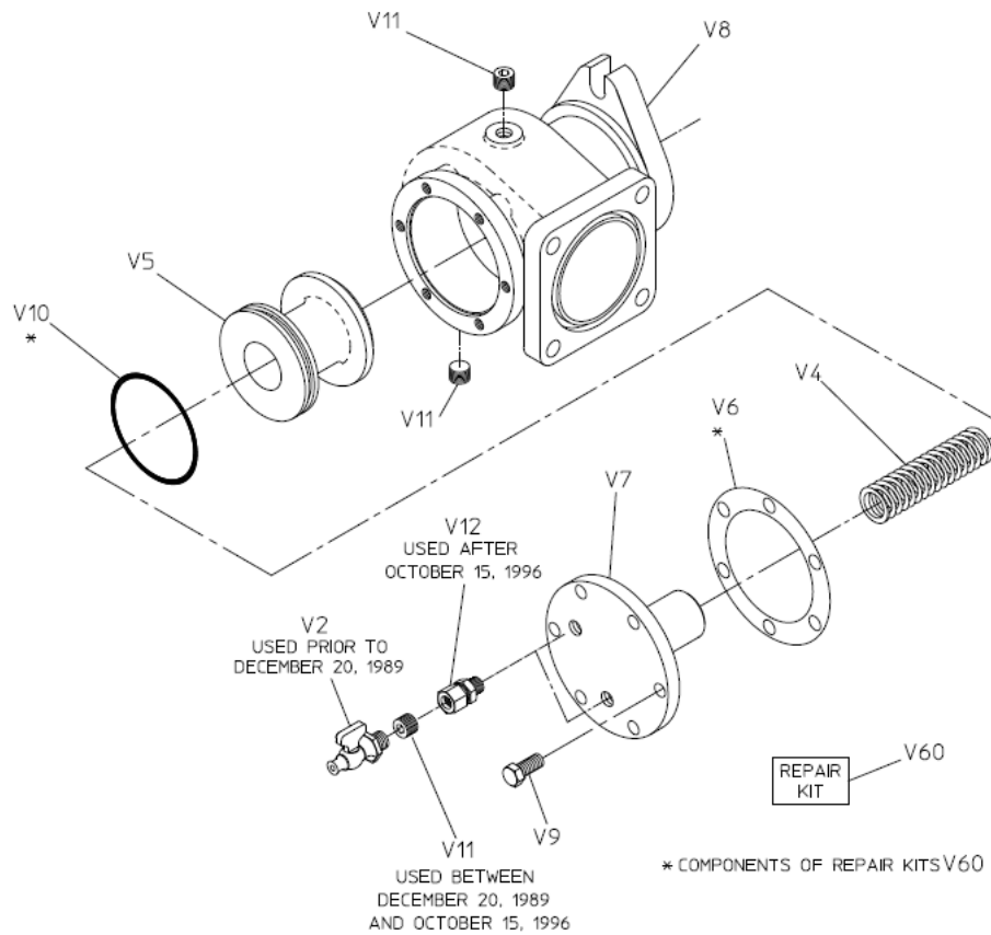
LEFT FACING DISCHARGE ASSEMBLY 80397-3 AND 80397-4
