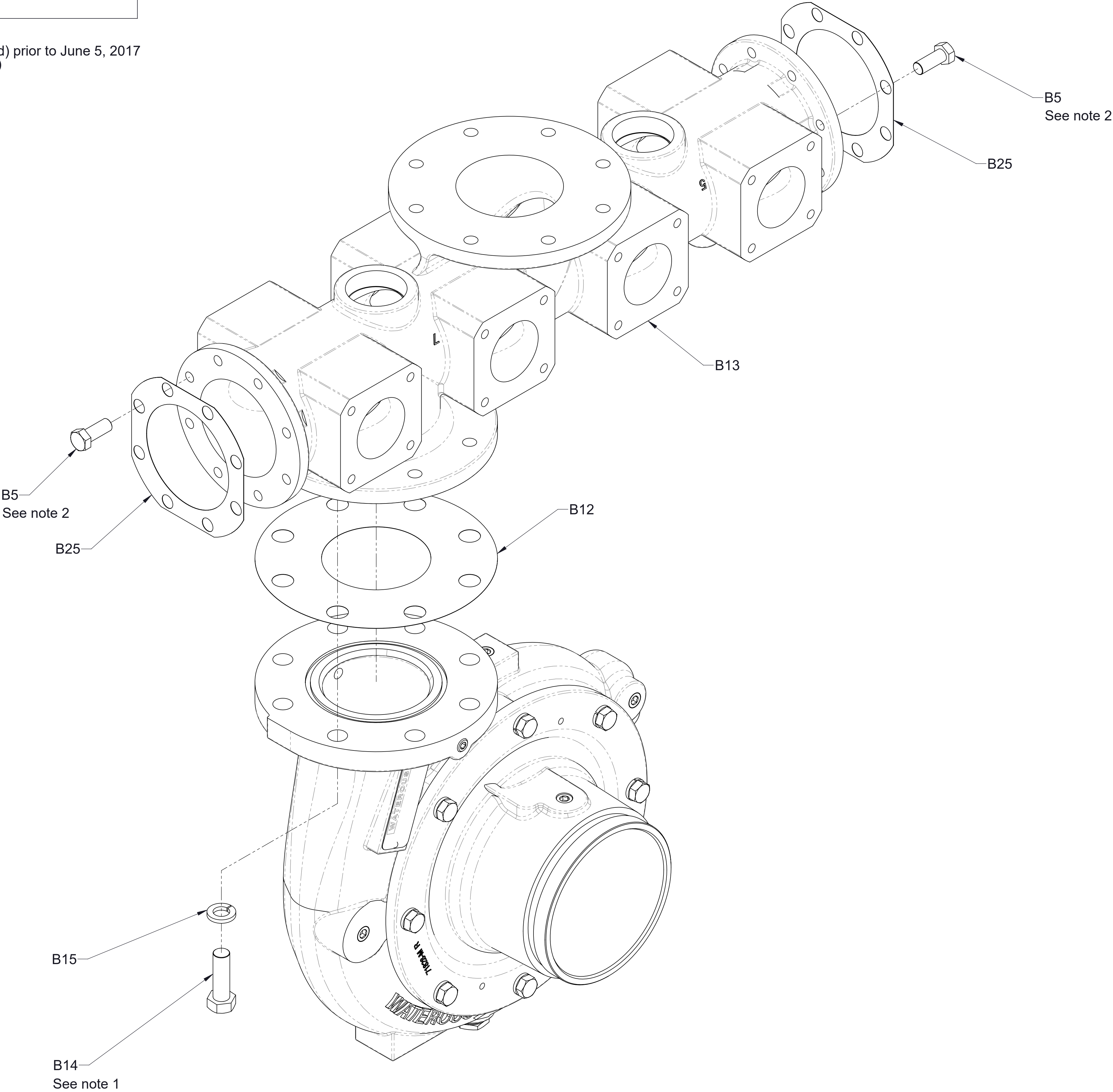
Discharge Manifold With 4 in. End Flanges
