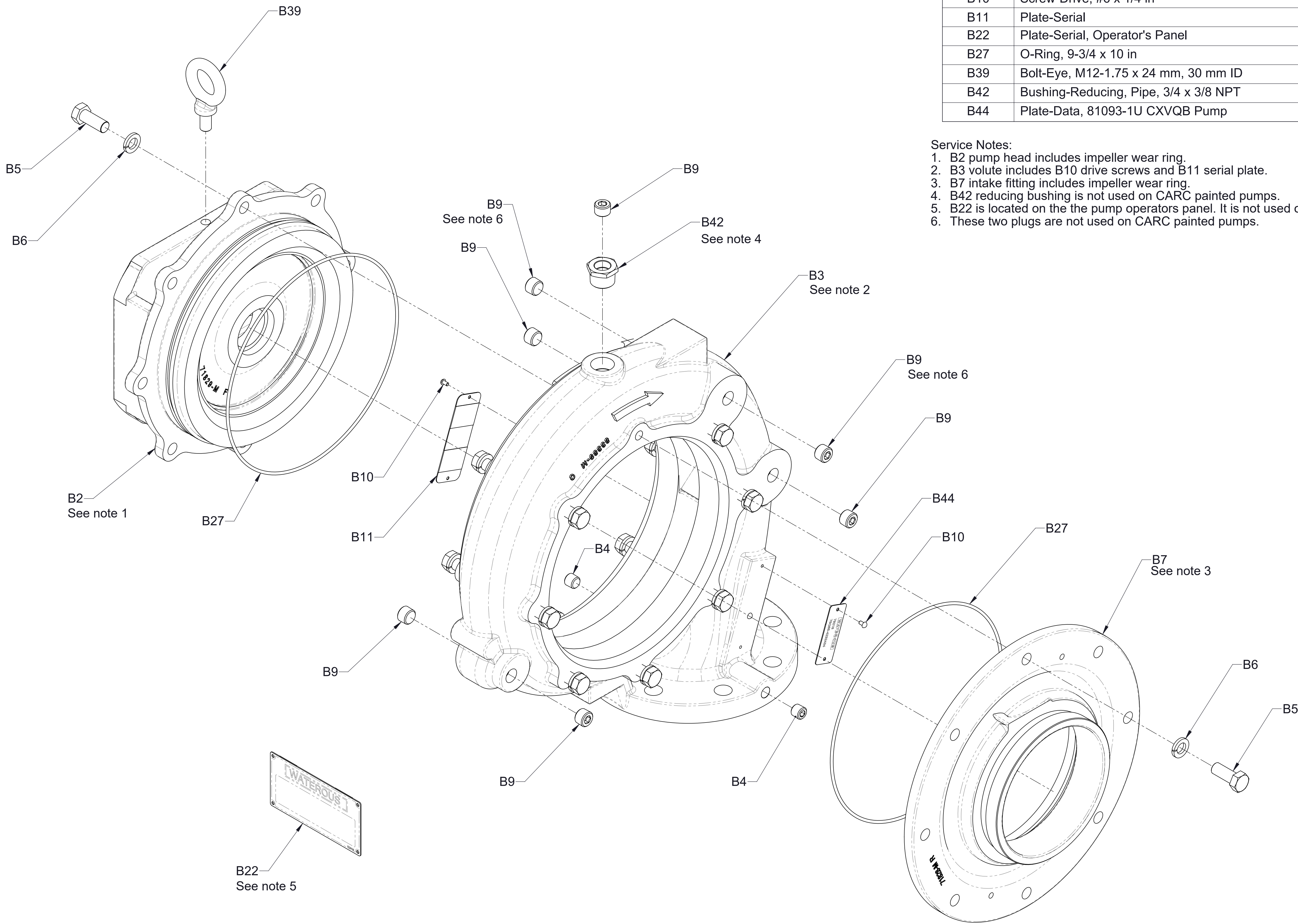
Body and Intake Fitting QB Series Transnsmission (Rear Facing Pump)
