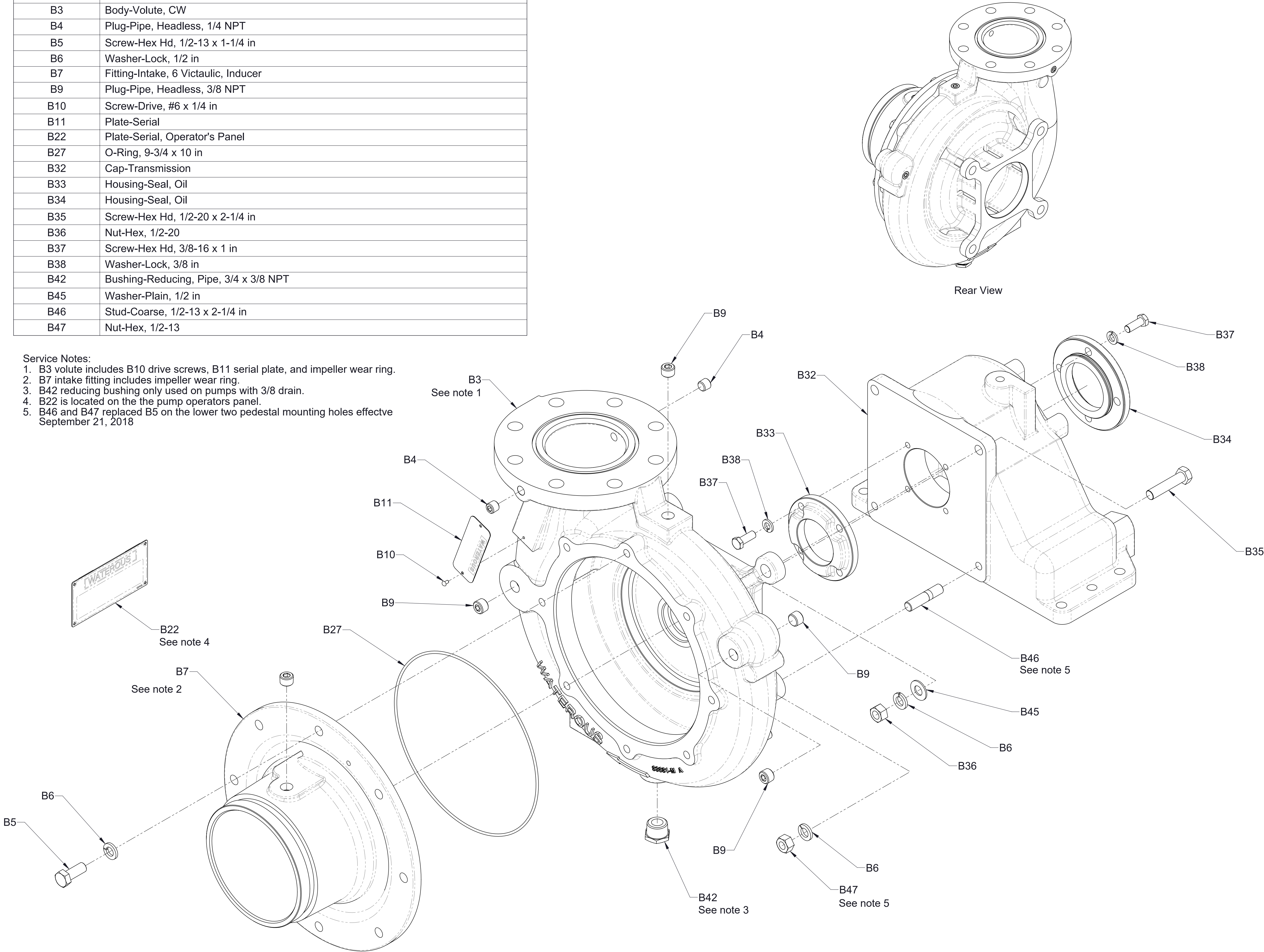
Body and Intake Fitting (One-Piece Volute) D Series Transnsmission
