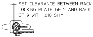
RACK LOCKING PLATE ADJUSTMENT (UNLOCKED POSITION)
