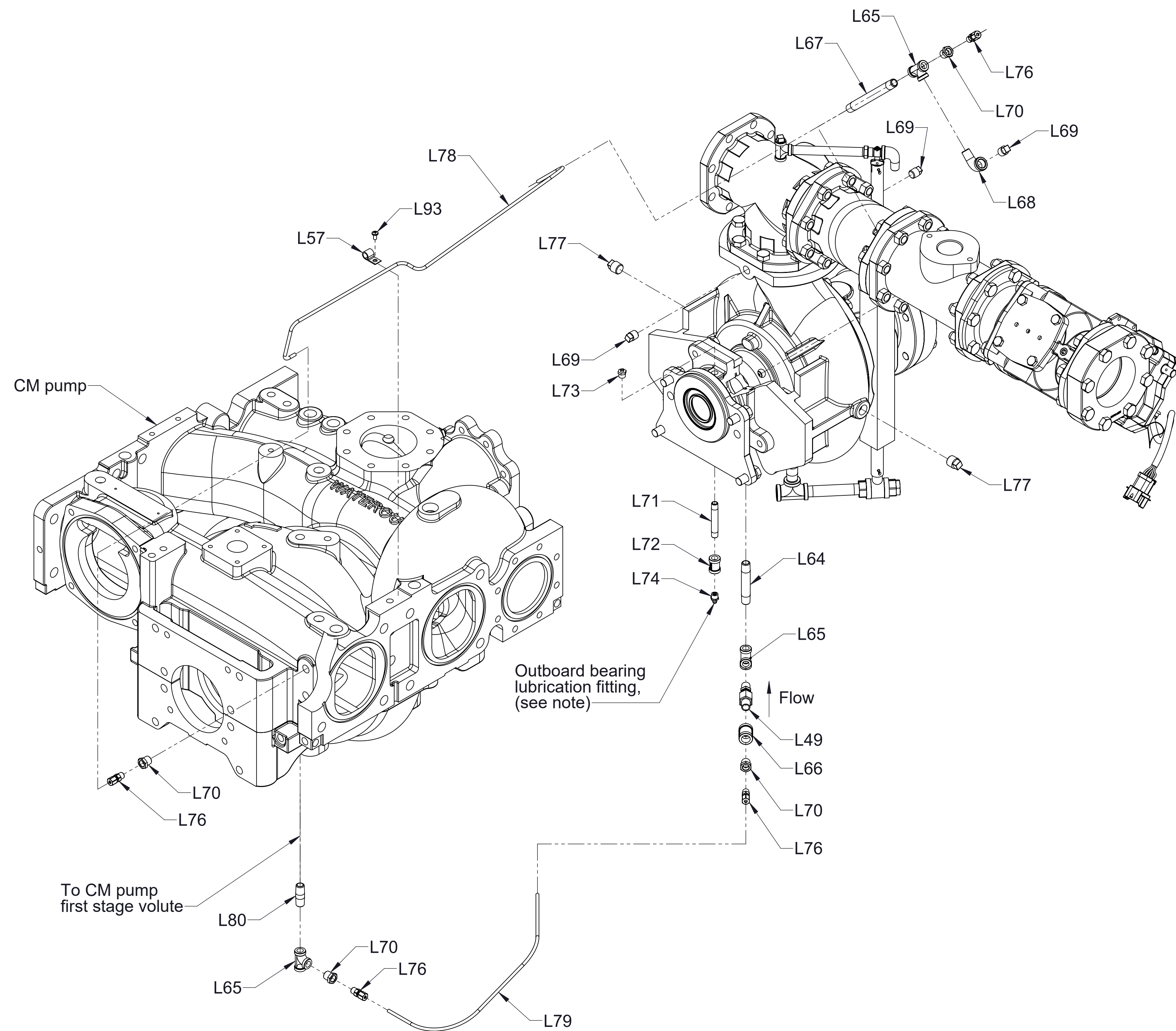
Seal Cooling Line Piping and Outboard Bearing Lubrication (Prior to November 25, 2013)
