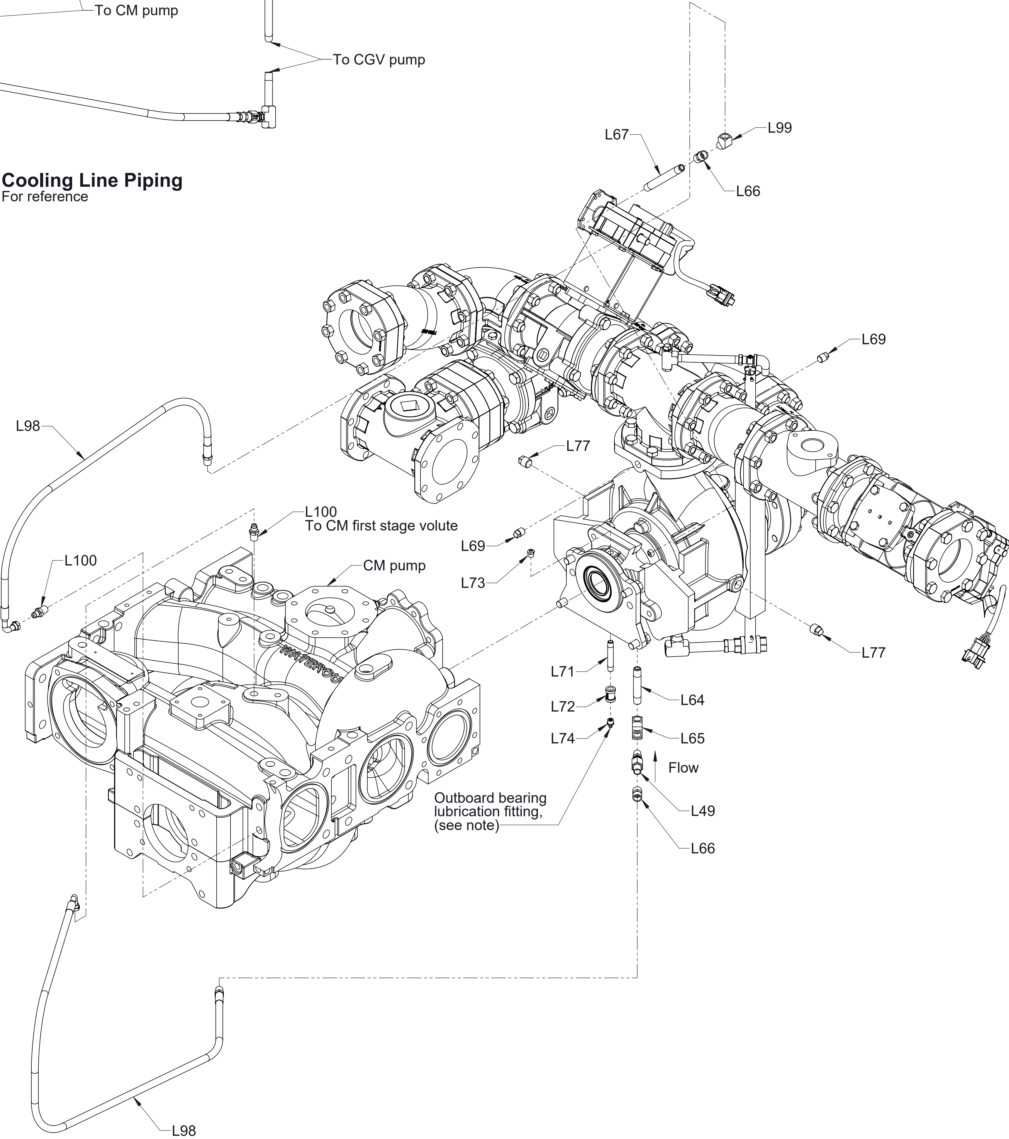
Seal Cooling Line Piping and Outboard Bearing Lubrication (After November 25, 2013)
