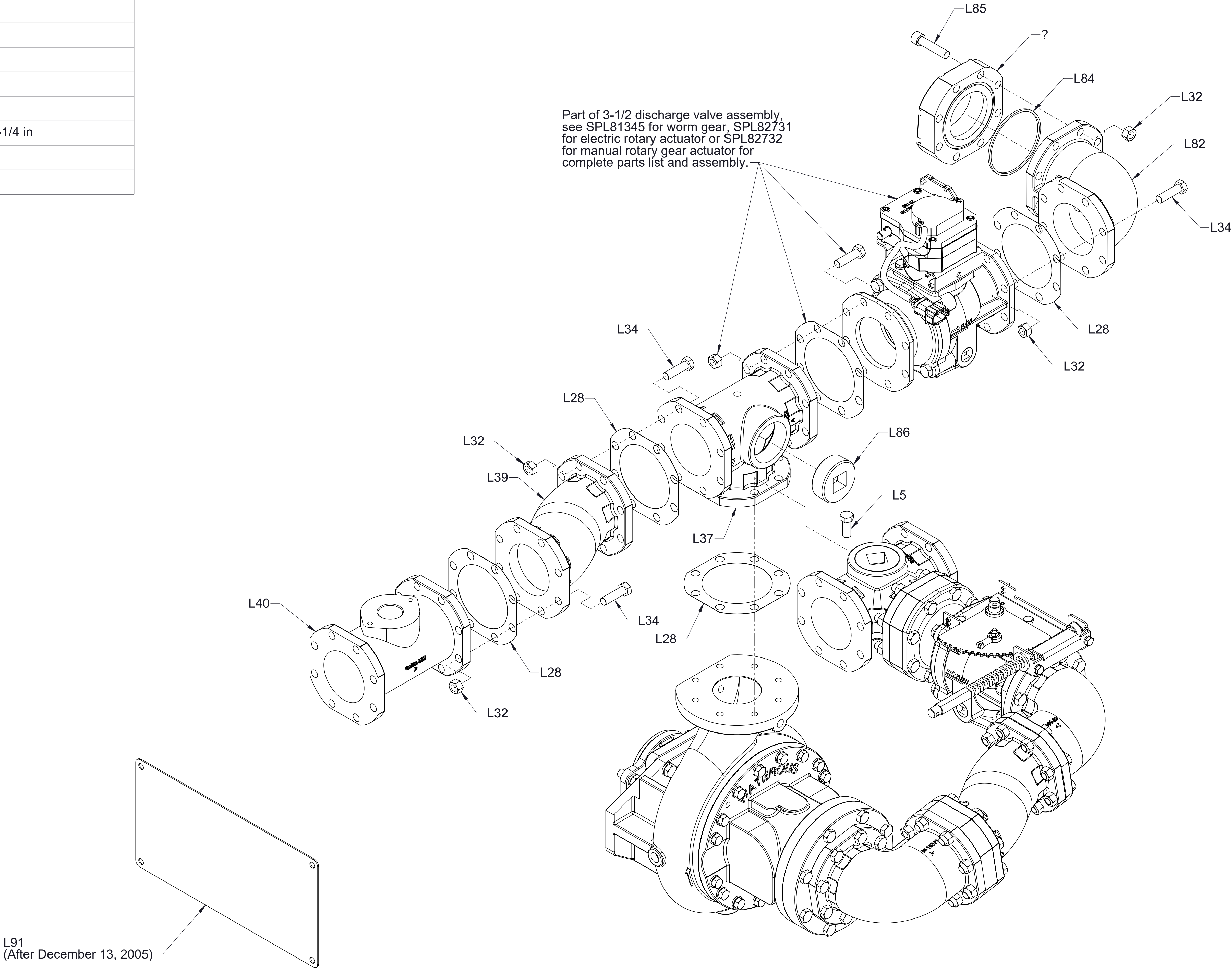
Tee from CM Discharge (Discharge Piping), one discharge valve (see page 6 for intake piping)
