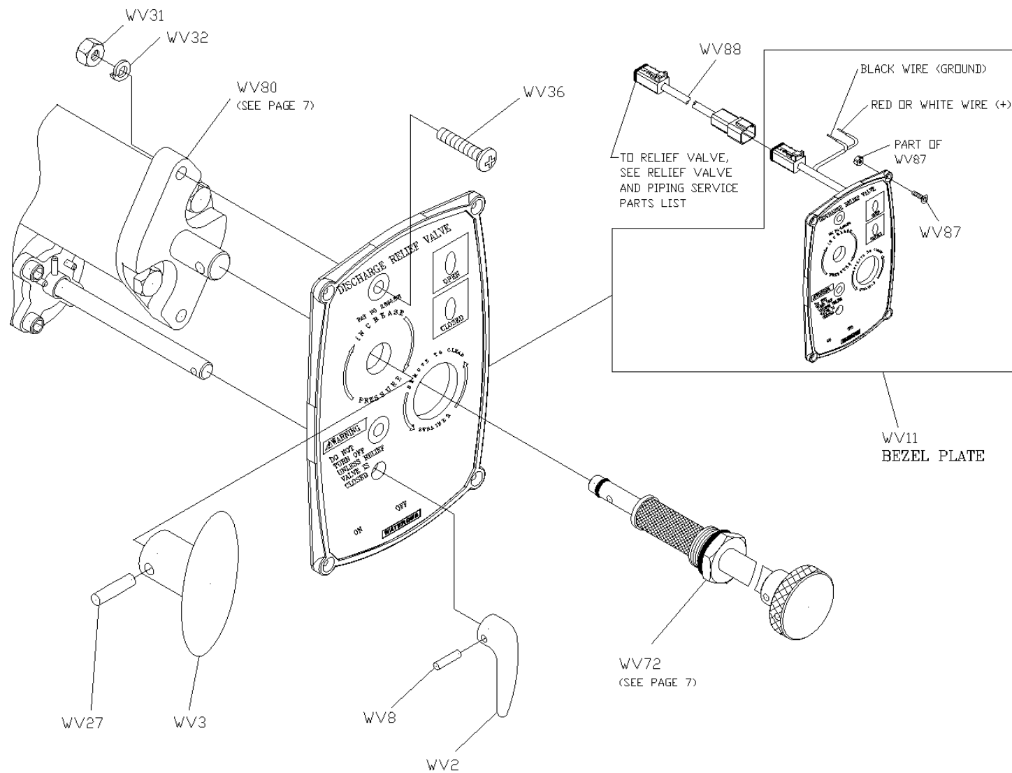
PANEL PLATE DESIGN AFTER APRIL 21, 2006 (BEZEL)
