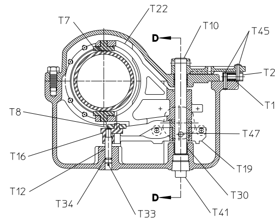
SECTION C-C
