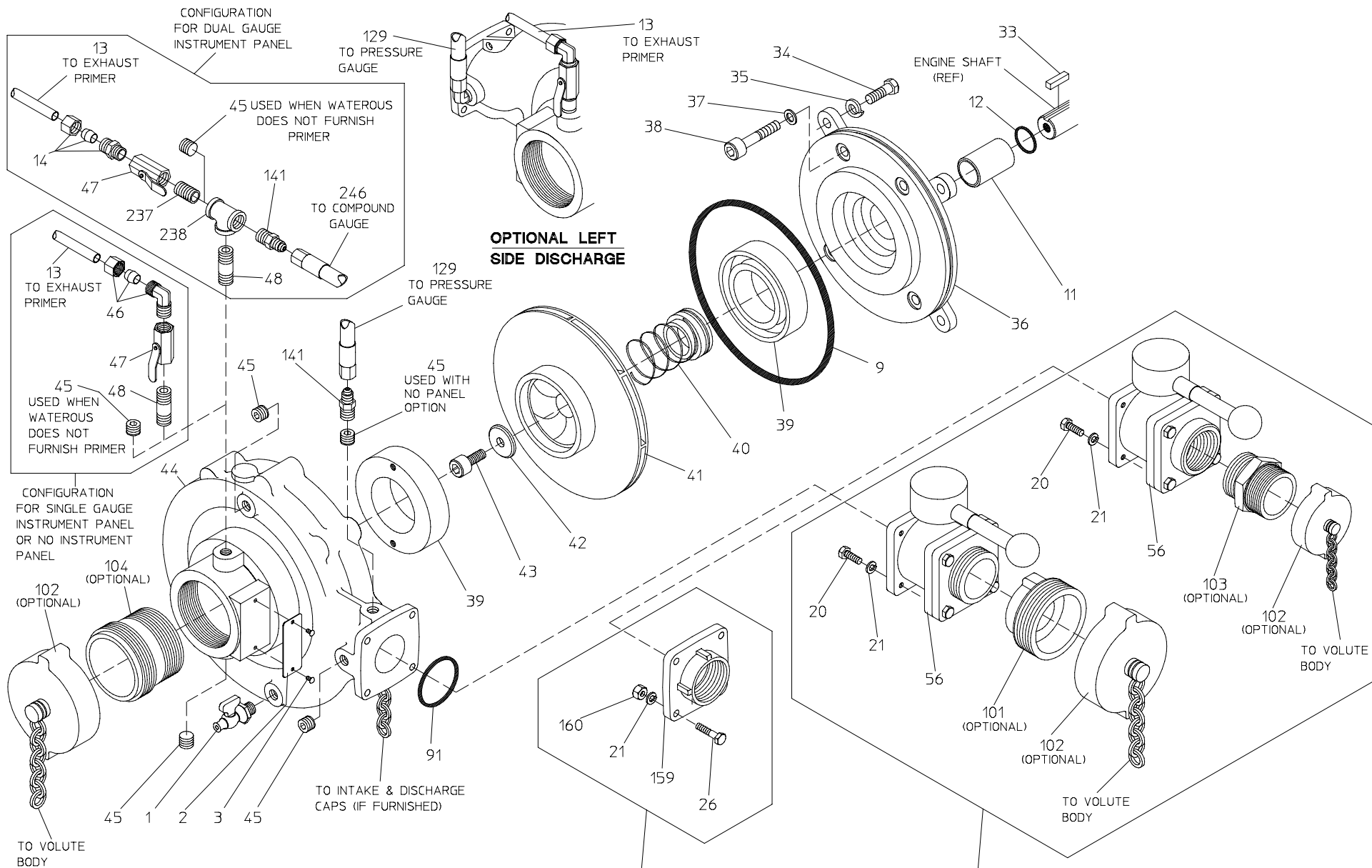
PUMP ASSEMBLY FOR MODELS PB18-2515 & PB18-2515B
