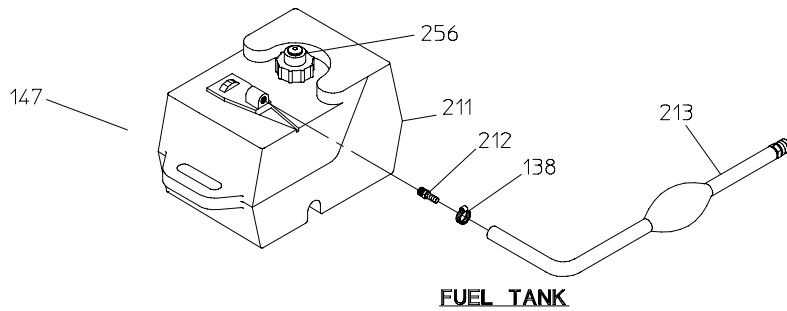
FUEL TANK
