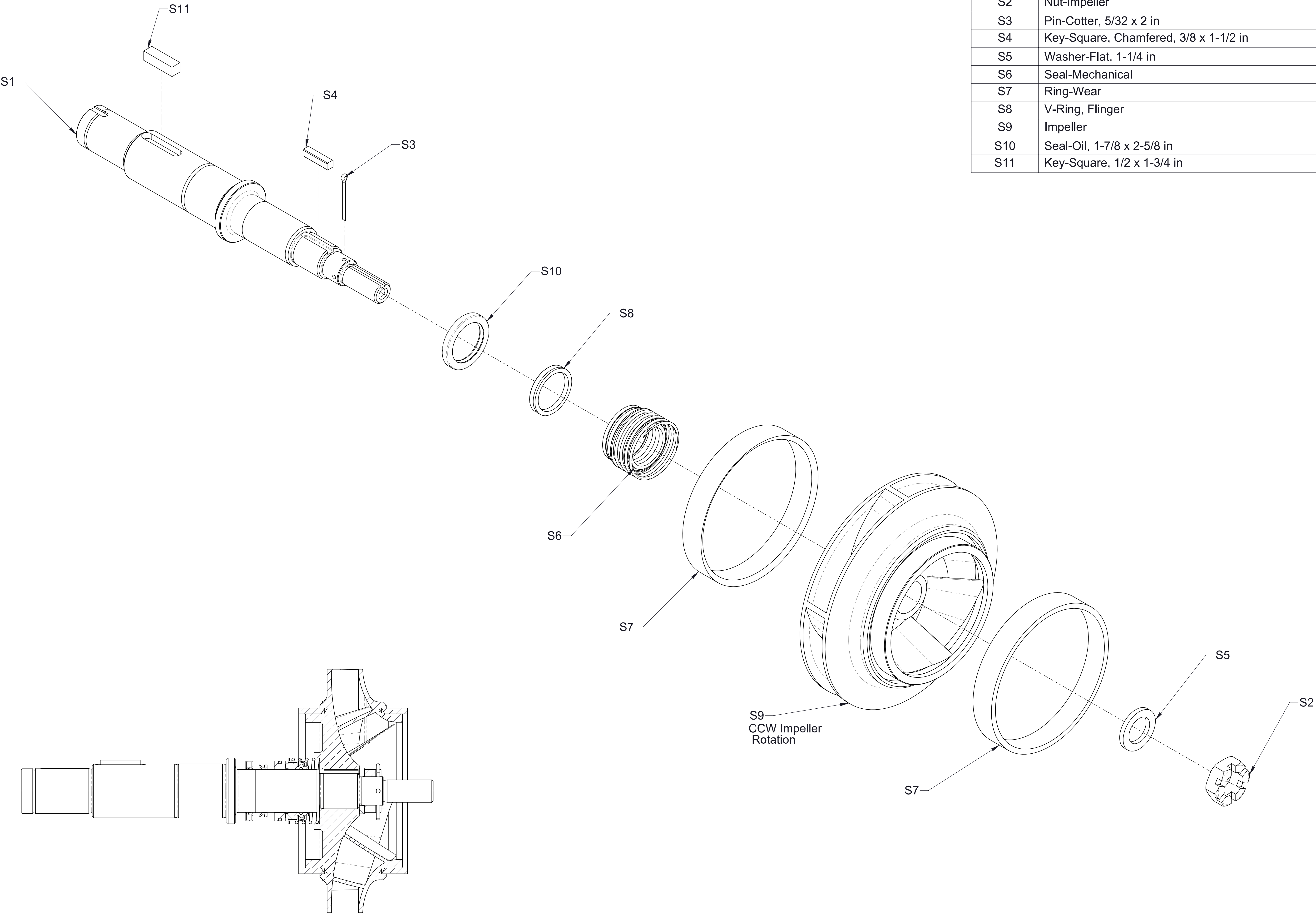
Section View
