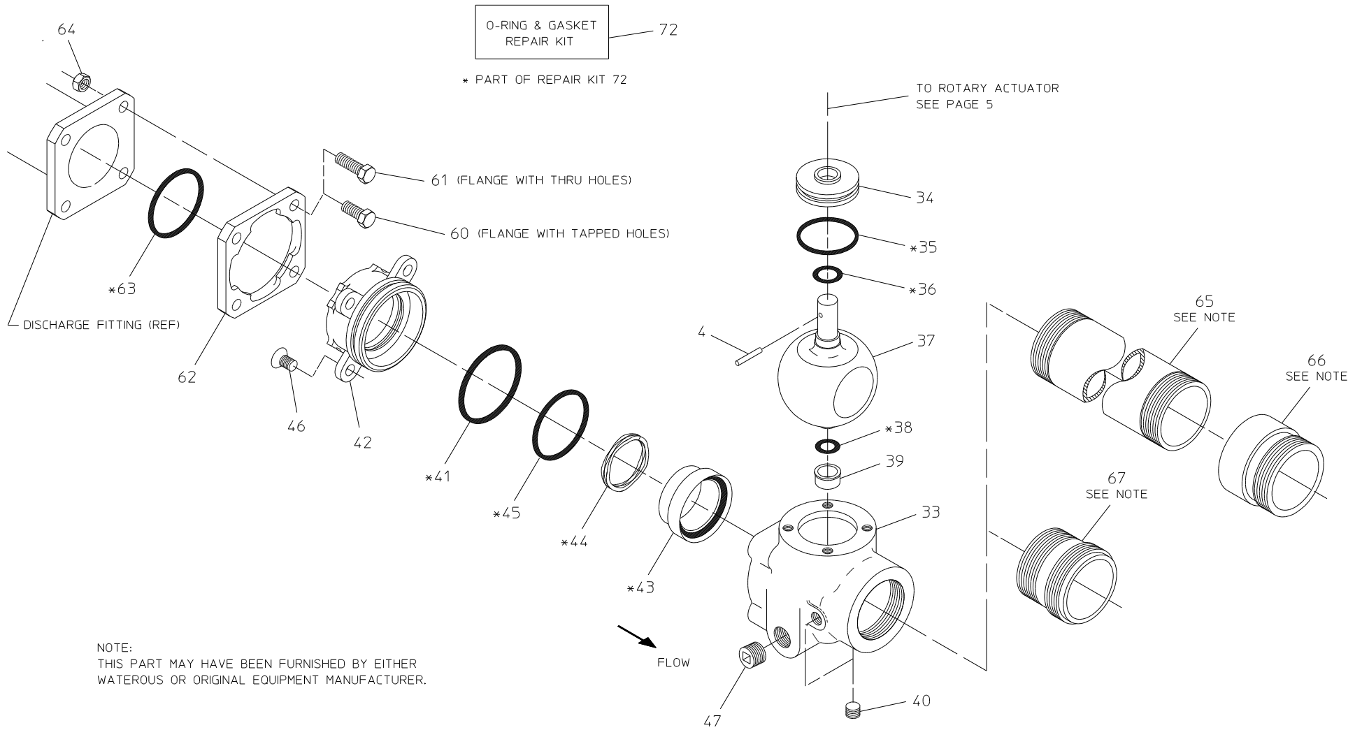
2-1/2 IN. STANDARD ELECTRIC BALL VALVE
