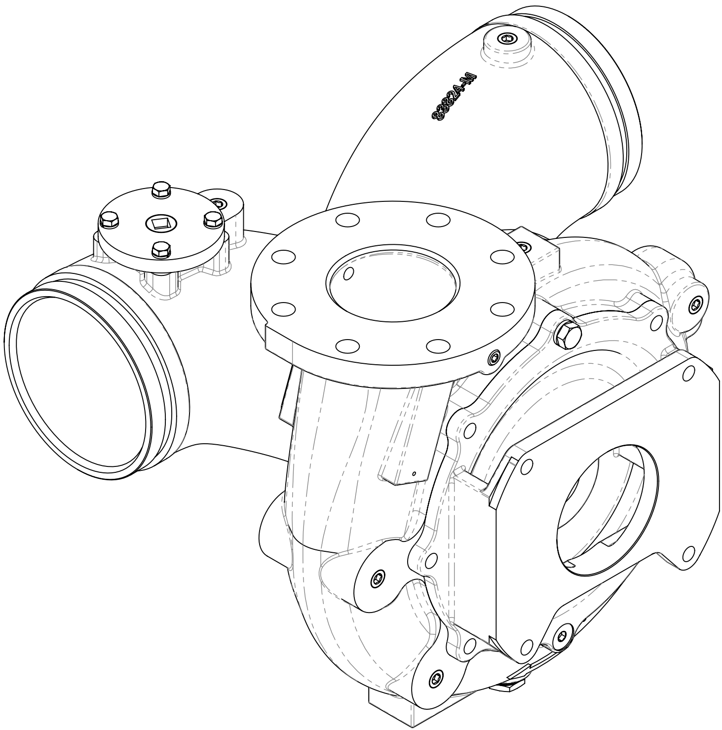
Rear View
