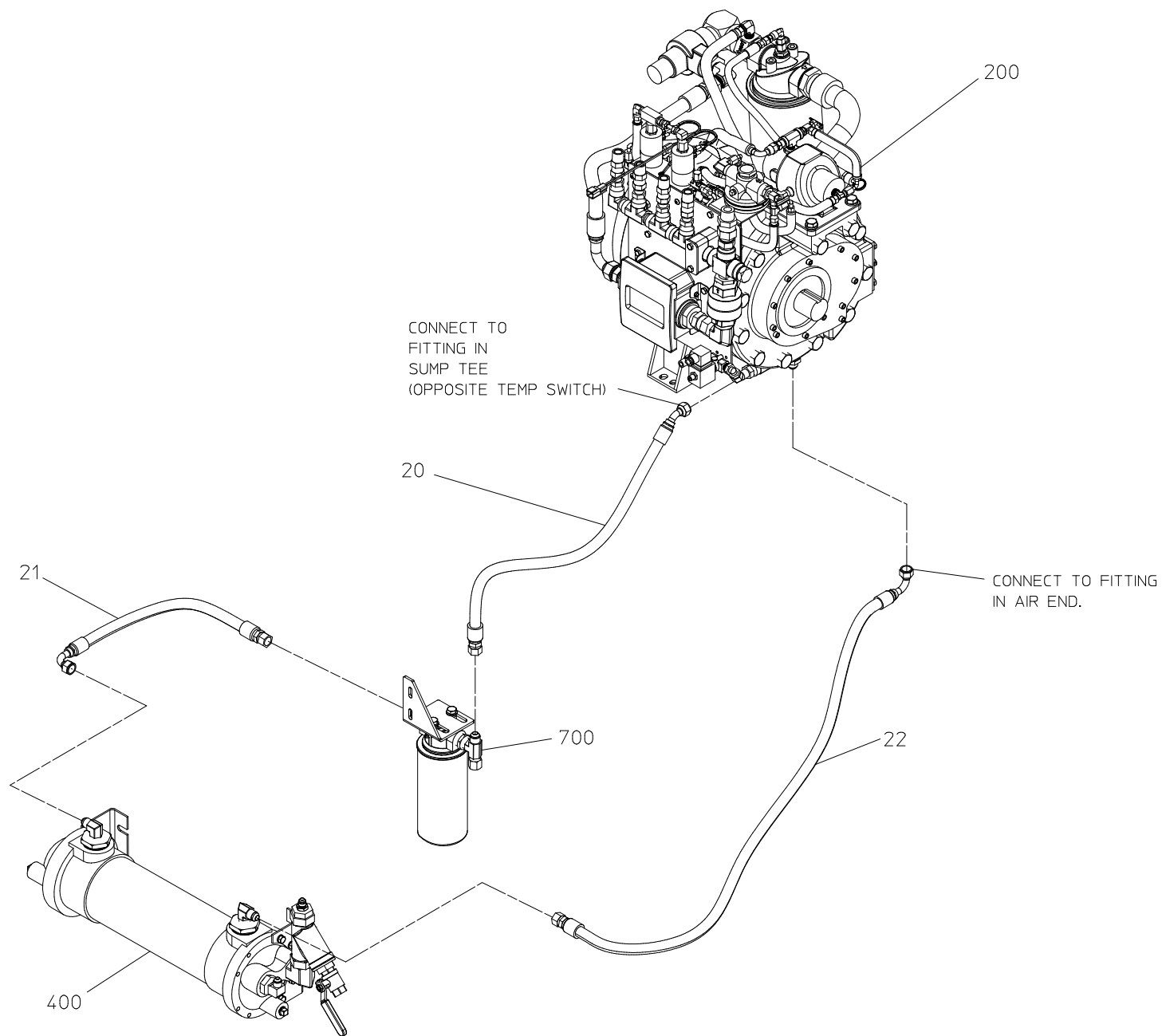
OIL COOLER AND FILTER – OIL LINES
