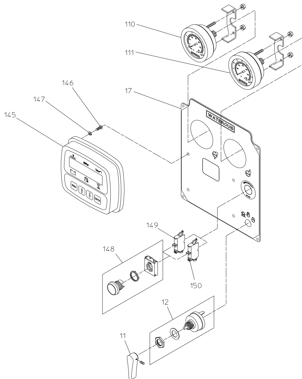
INSTRUMENT PANEL SINGLE AND DUAL OPTIONS
