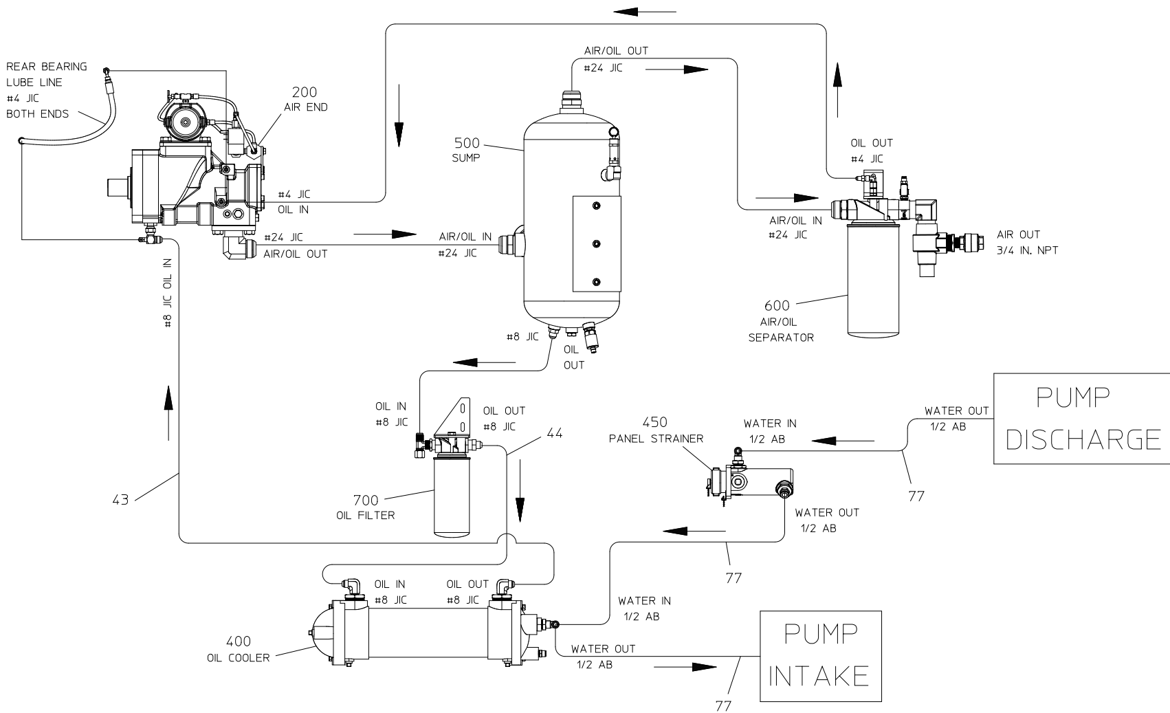
SCHMATIC - HYDRAULIC PANEL MOUNTED STRAINER
