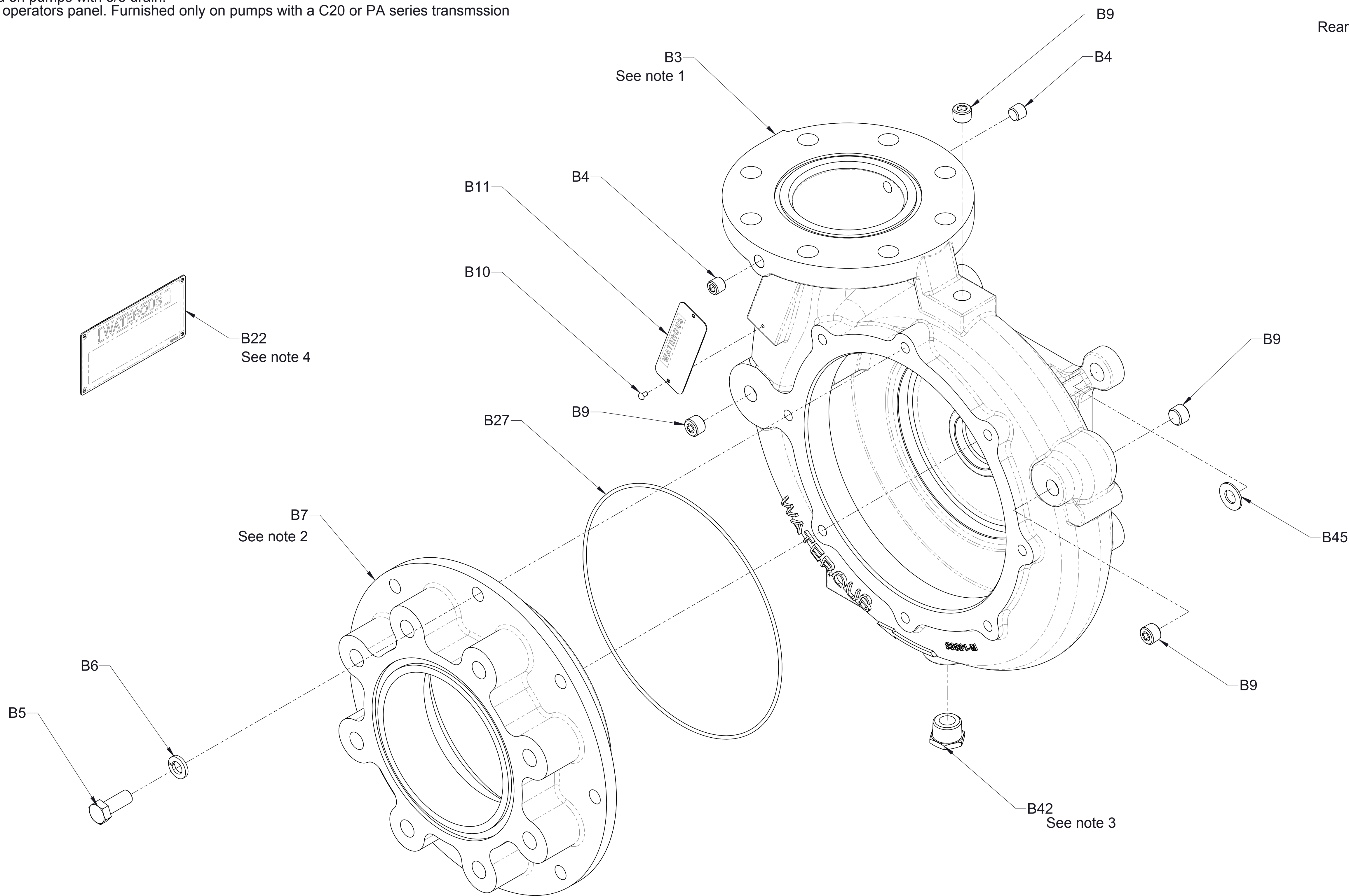
Body and Intake Fitting (One-Piece Volute) C20, K, T, and P Series Transnsmission
