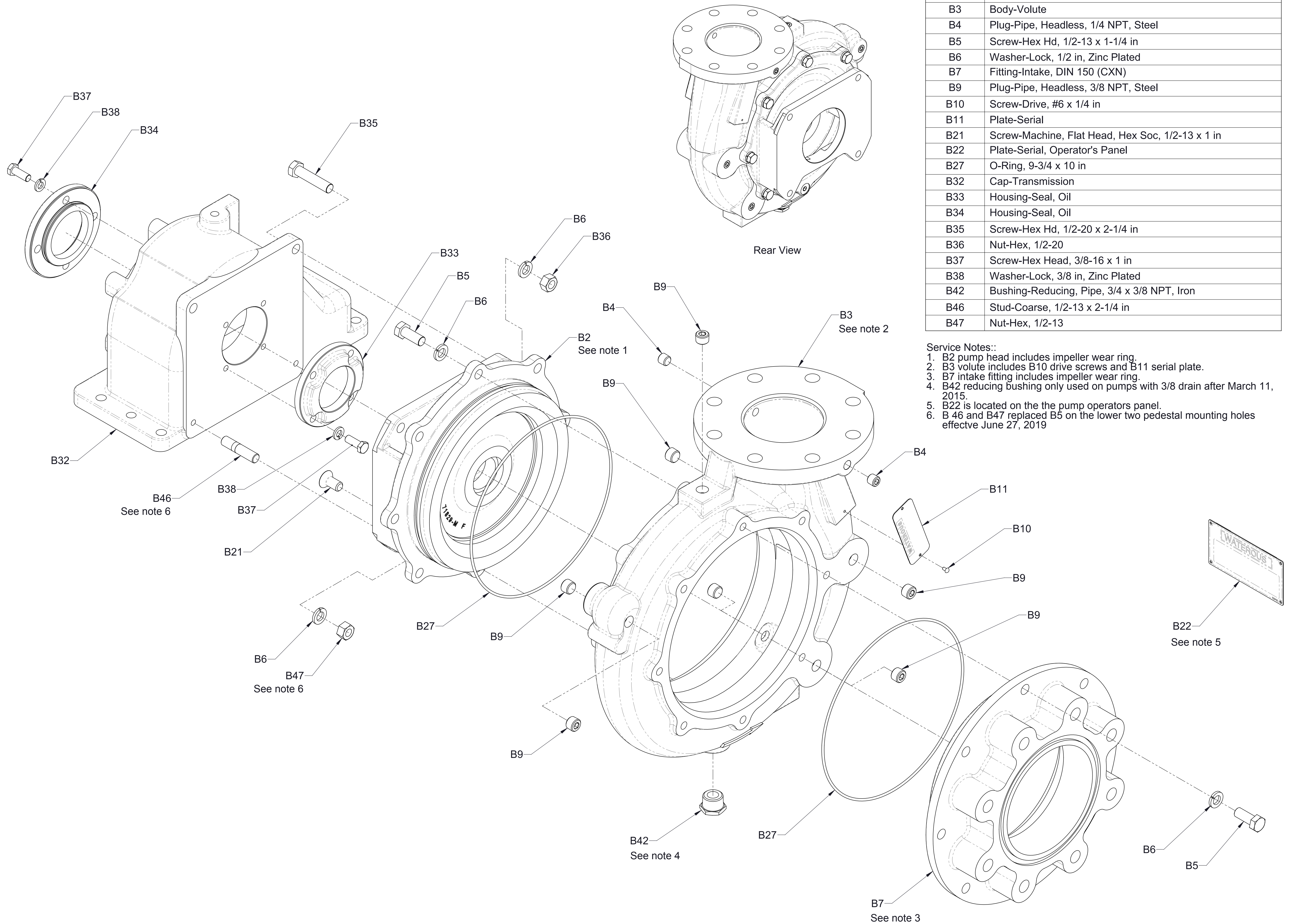
Body and Intake Fitting (Two-Piece Volute) D Series Transnmission
