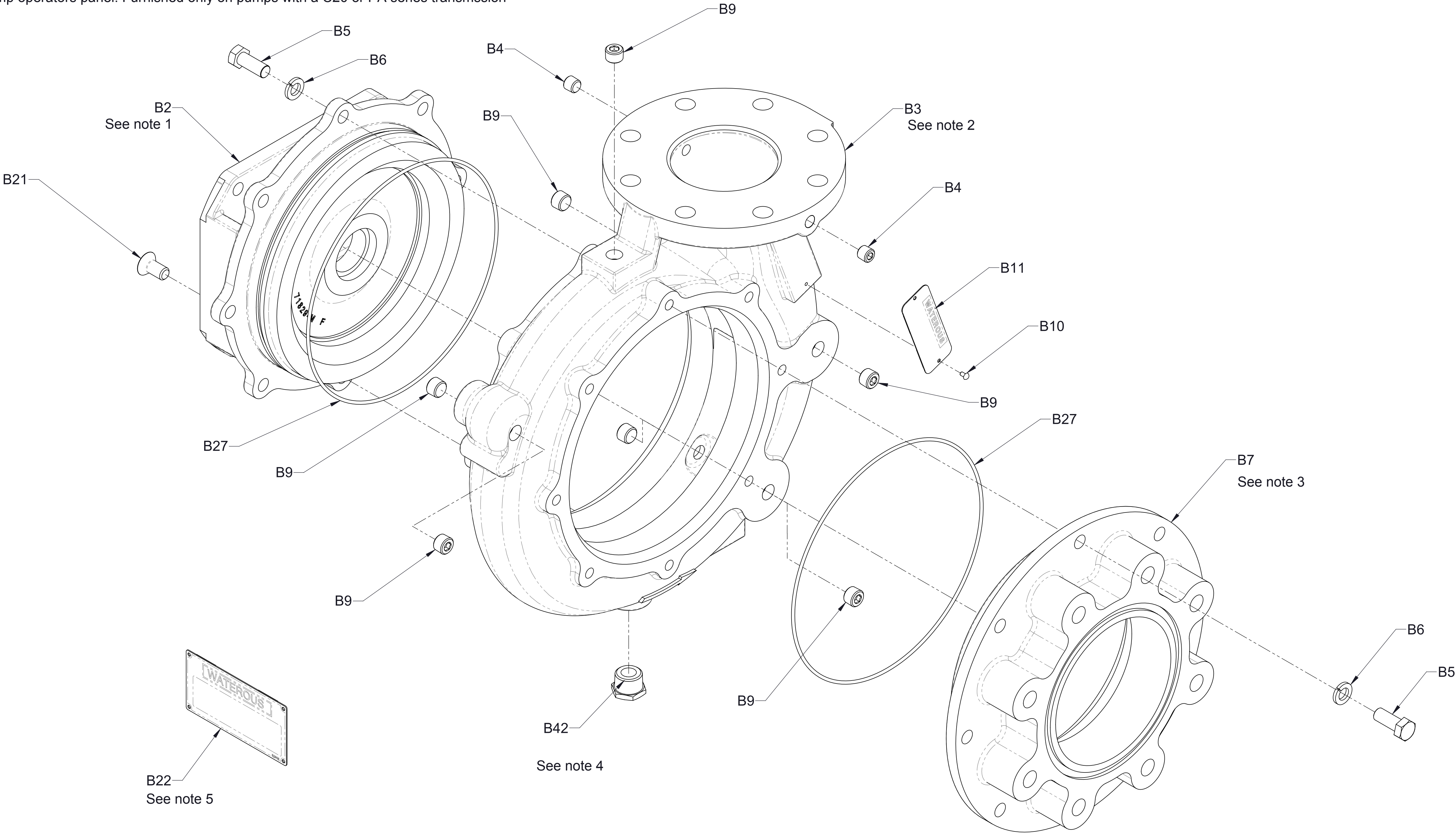
Body and Intake Fitting (Two-Piece Volute) C20, K, T, and P Series Transnsmission
