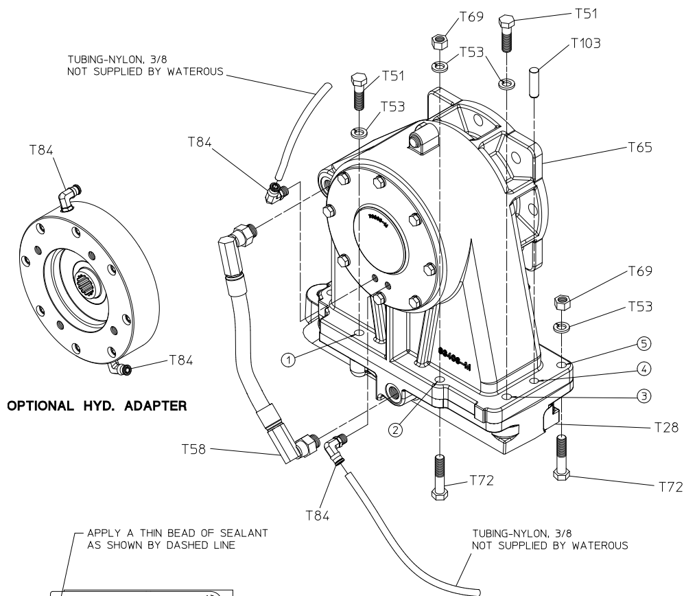
VIEWED FROM OUTPUT SIDE OF CASE
