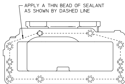
DETAIL A APPLY LOCTITE® 518 SEALANT OR EQUIVALENT TO MATING FLANGES
