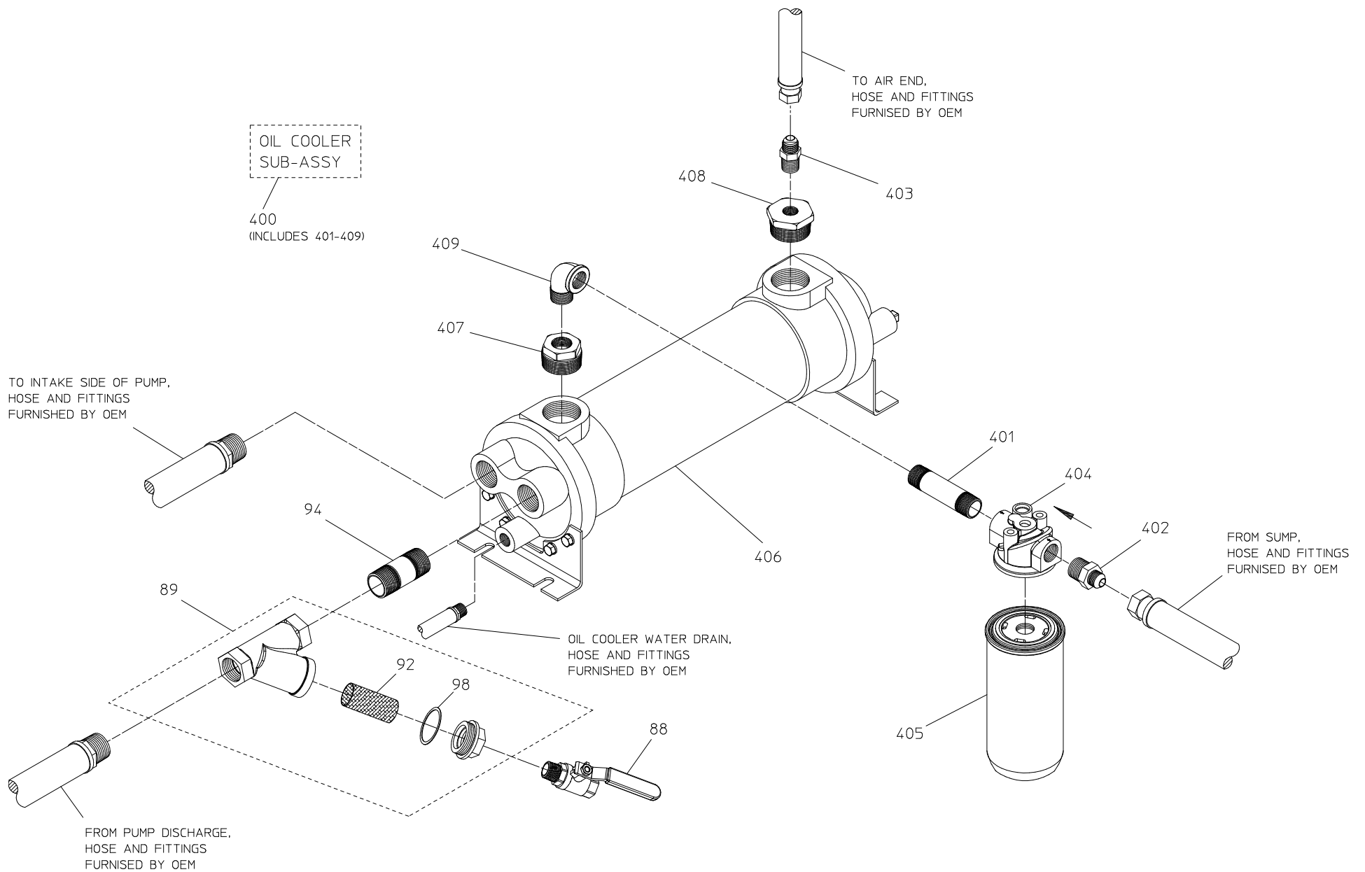
OIL COOLER AND FILTER
