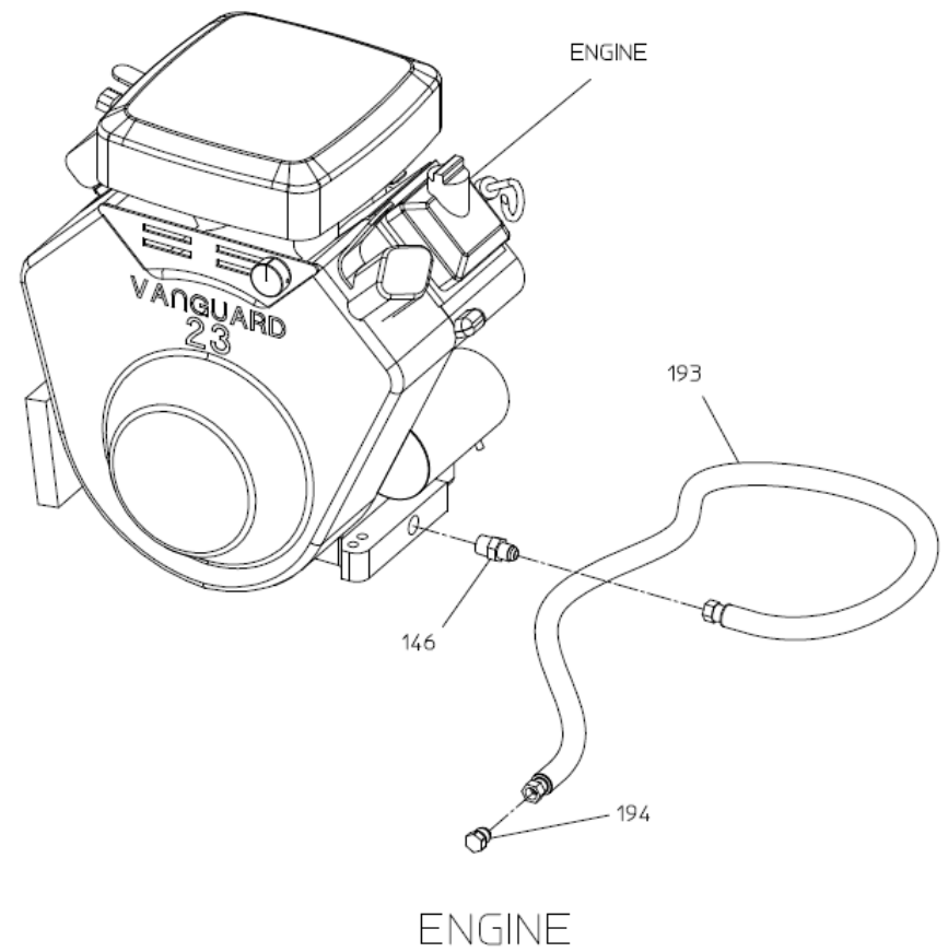
TUBING AND HOSES — OIL DRAIN SUMP AND ENGINE
