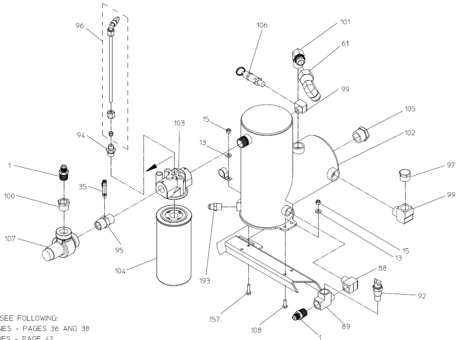
SUMP AND SEPARATOR
