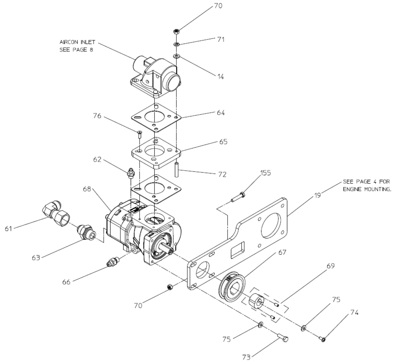
COMPRESSOR — MOUNTING
