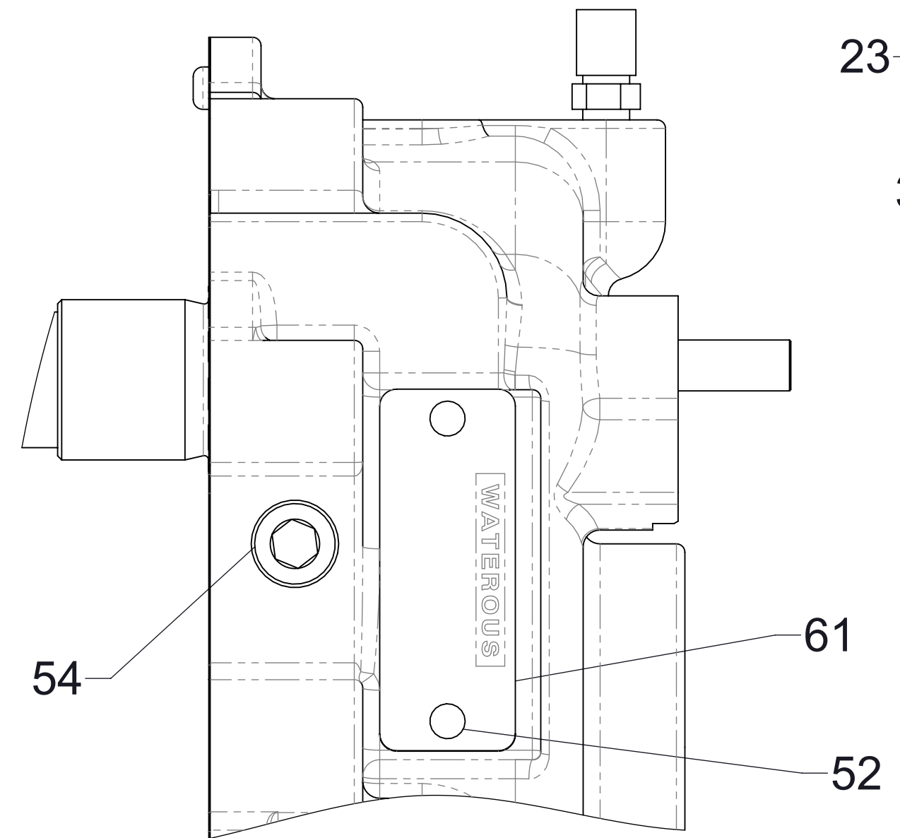
View C-C
