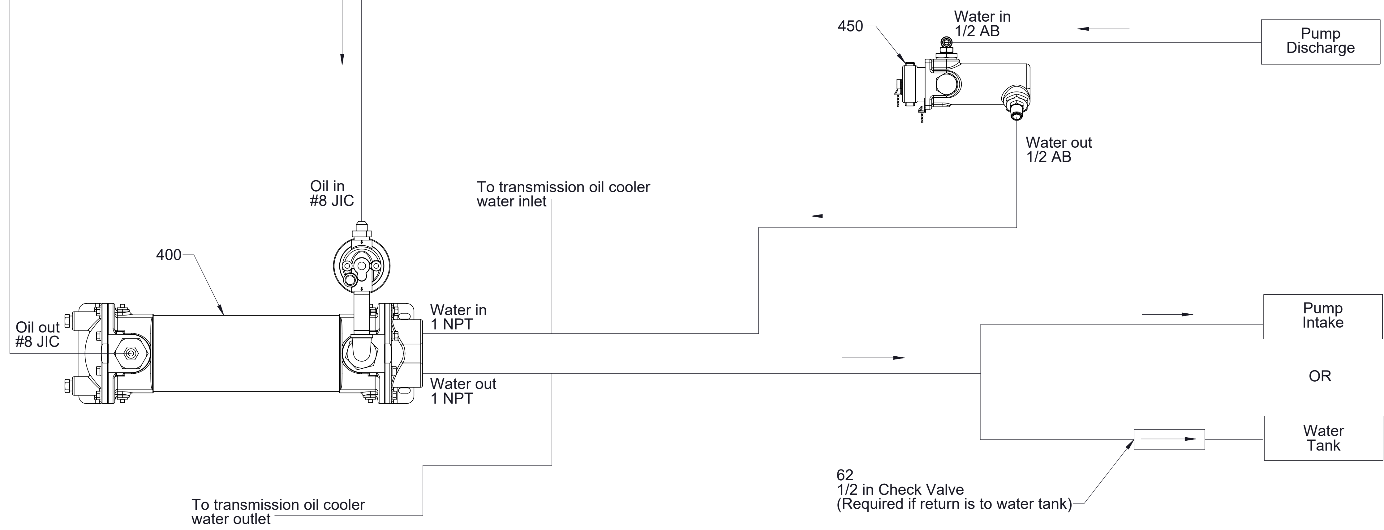
Schematic-Hydraulic Lines
