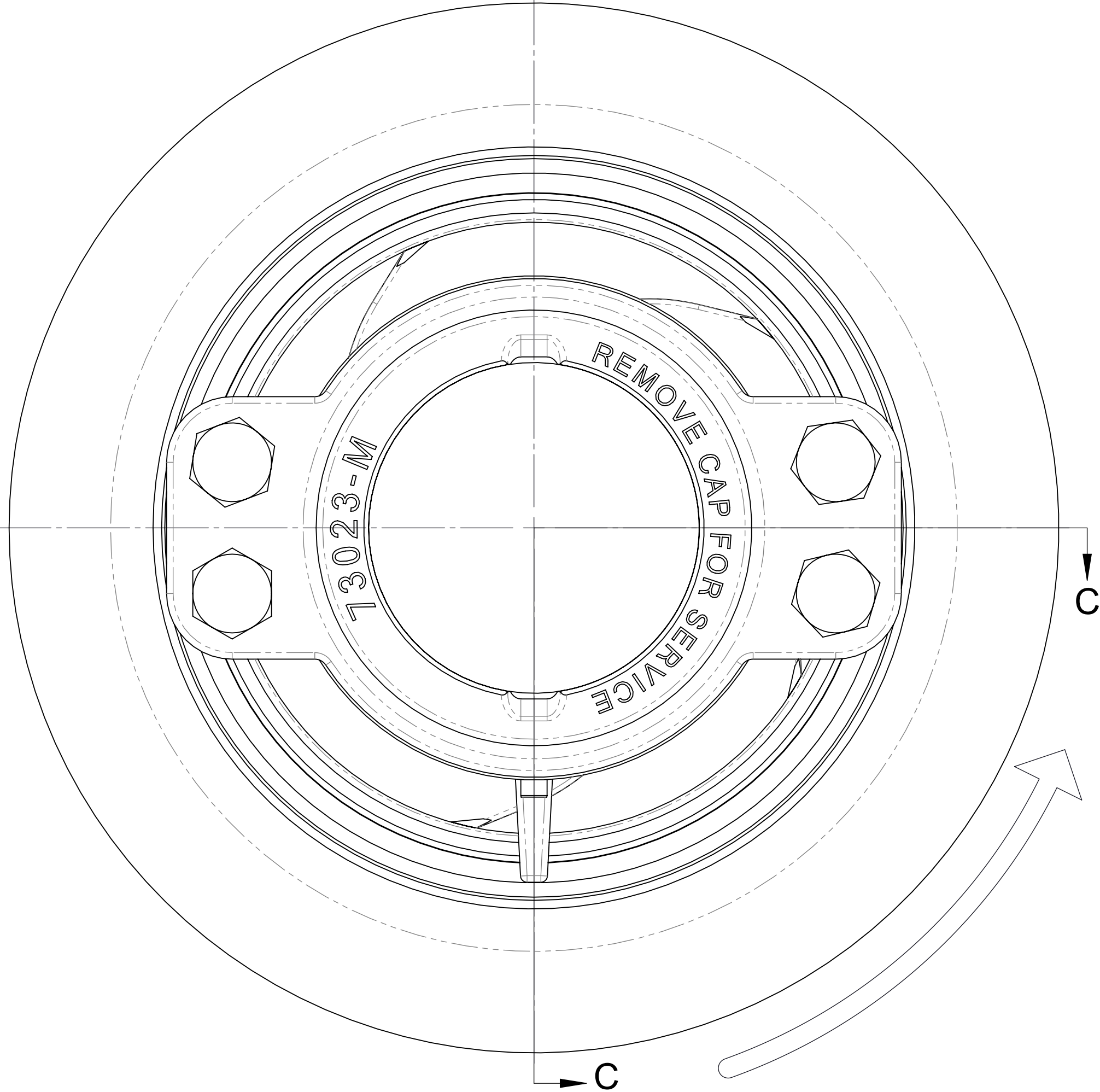
Looking into eye of first stage impeller
