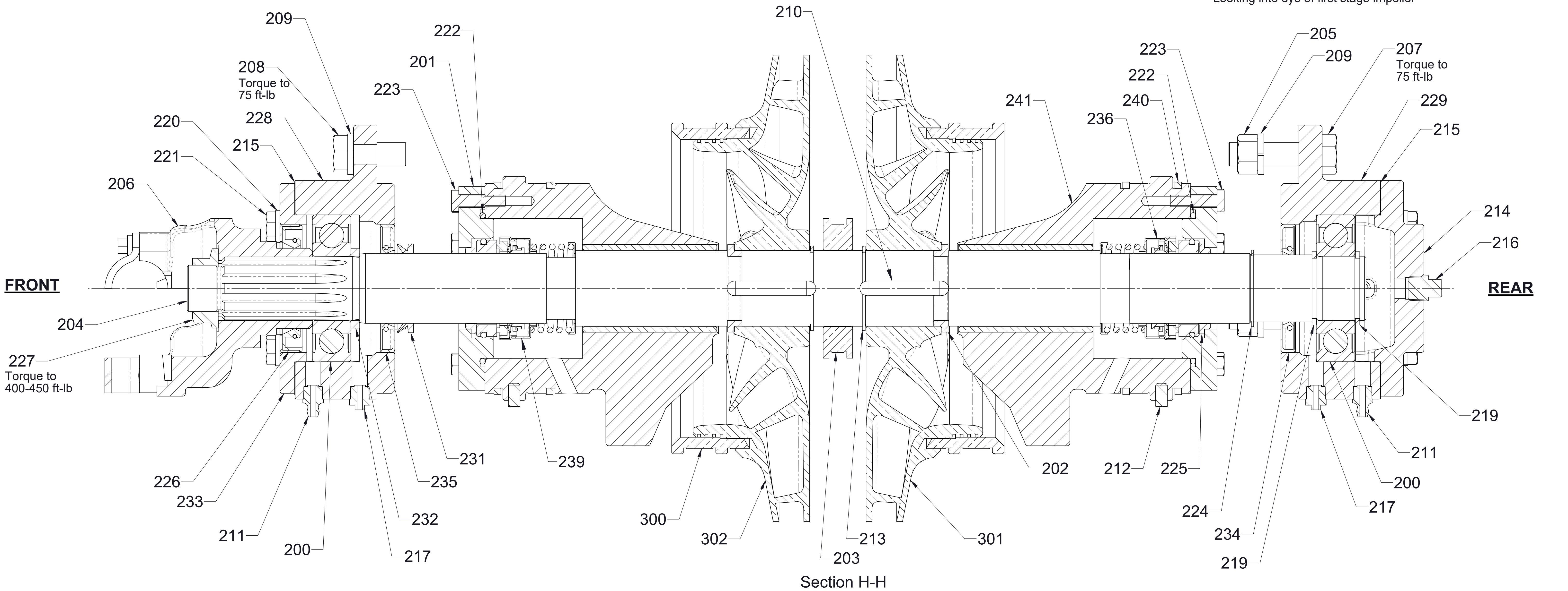
CMD, CMUD One-Piece Shaft with Mechanical Seals Front Drive (CMU Shown)
