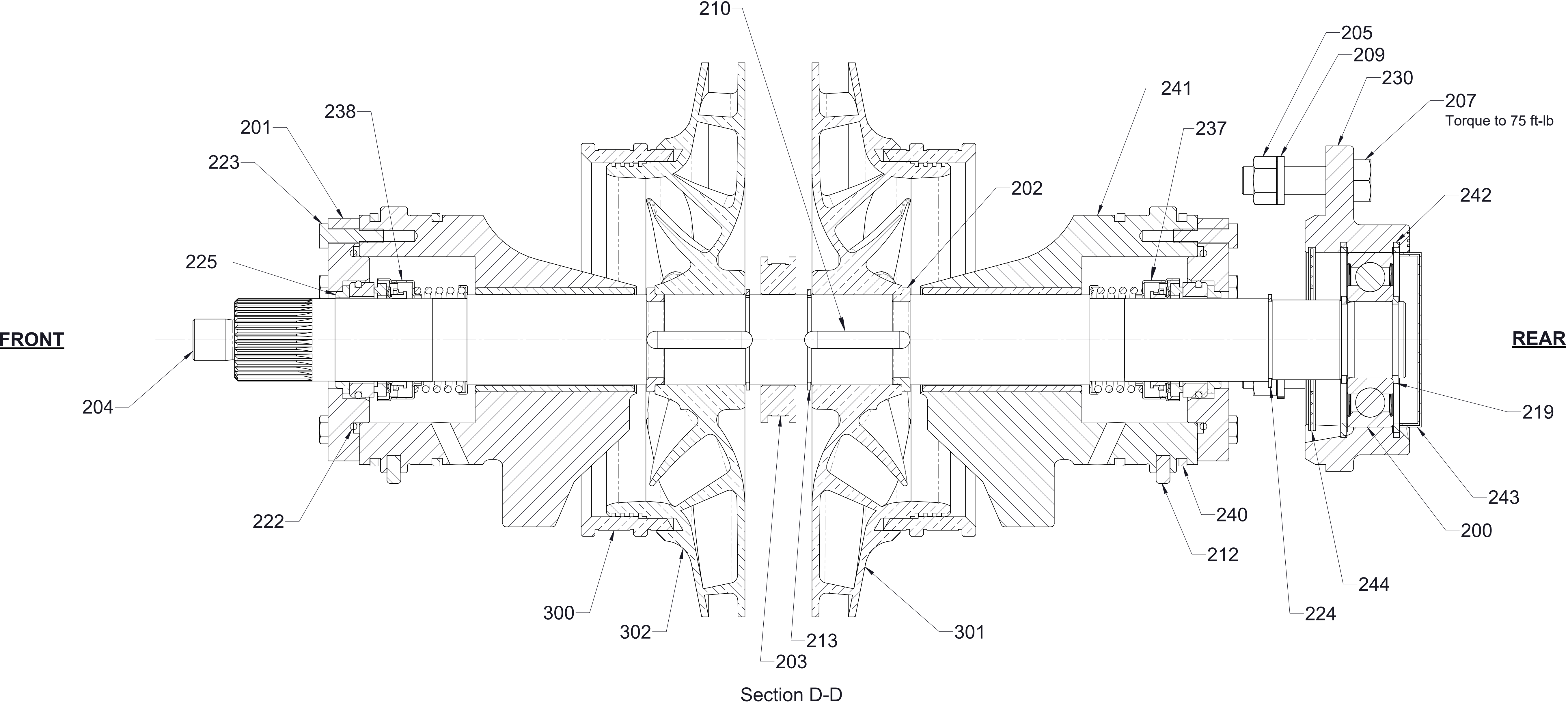
CM, CMU Separable Shaft with Mechanical Seals Front Drive (CMU Shown)
