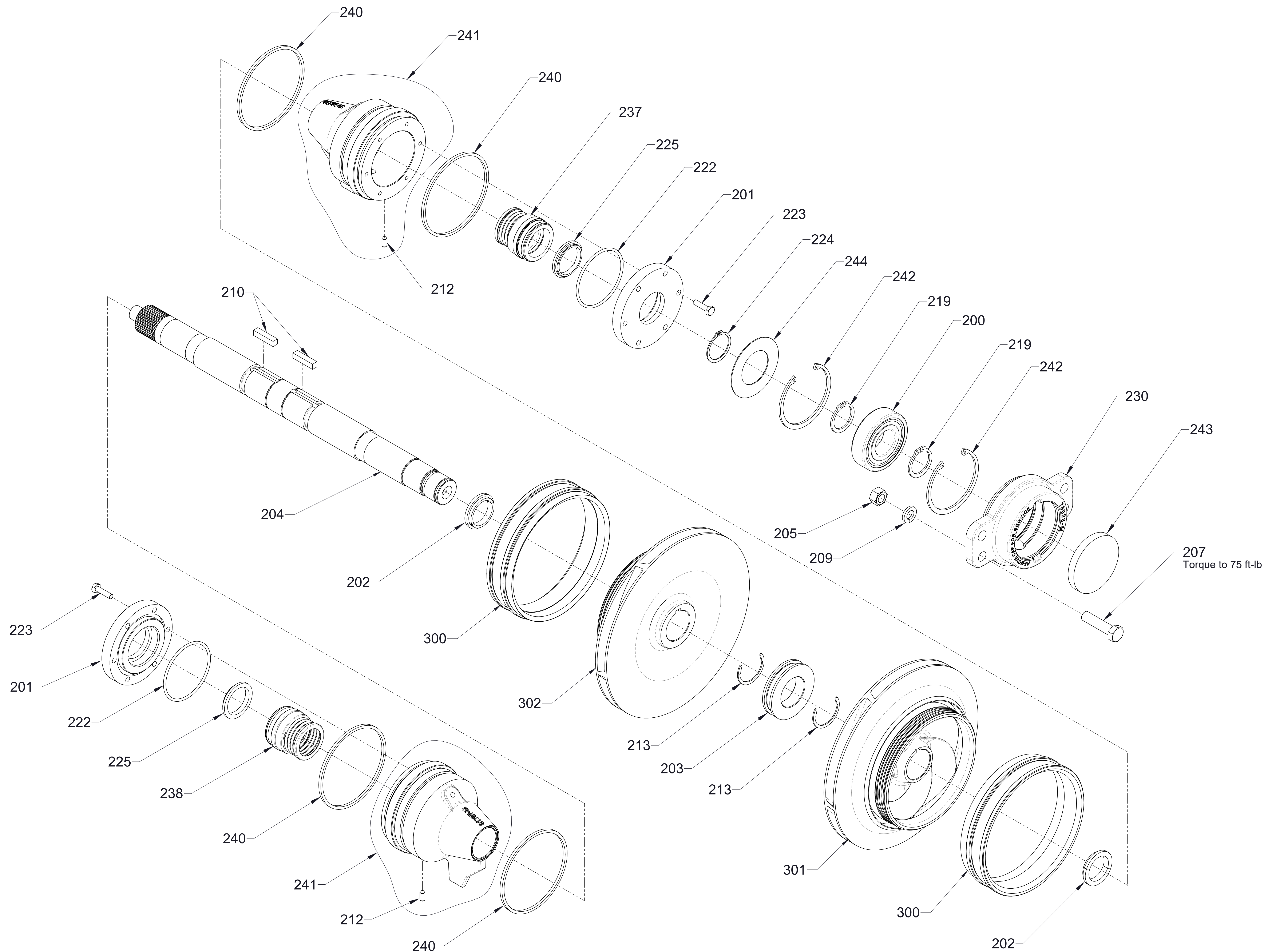
CM, CMU Separable Shaft with Mechanical Seals Front Drive (CMU Shown)
