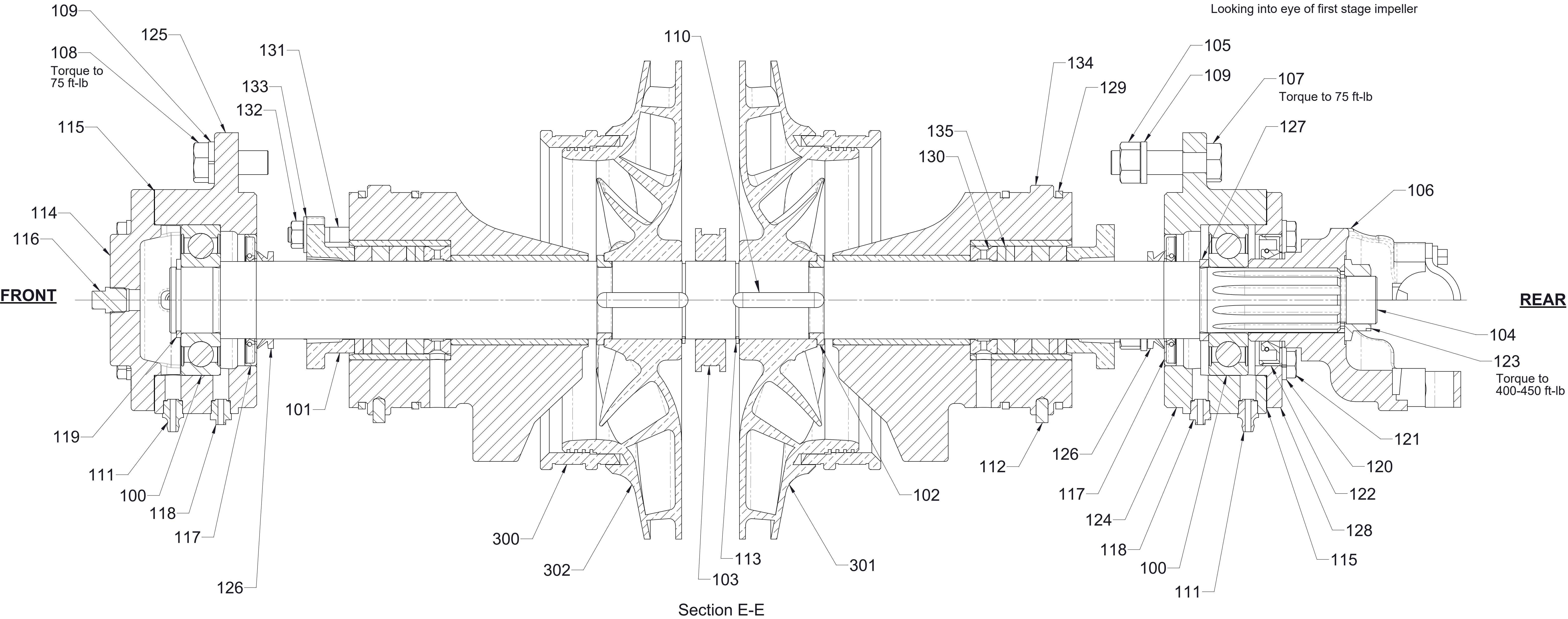
CMD, CMUD One-Piece Shaft with Packing Rear Drive (CMU Shown)
