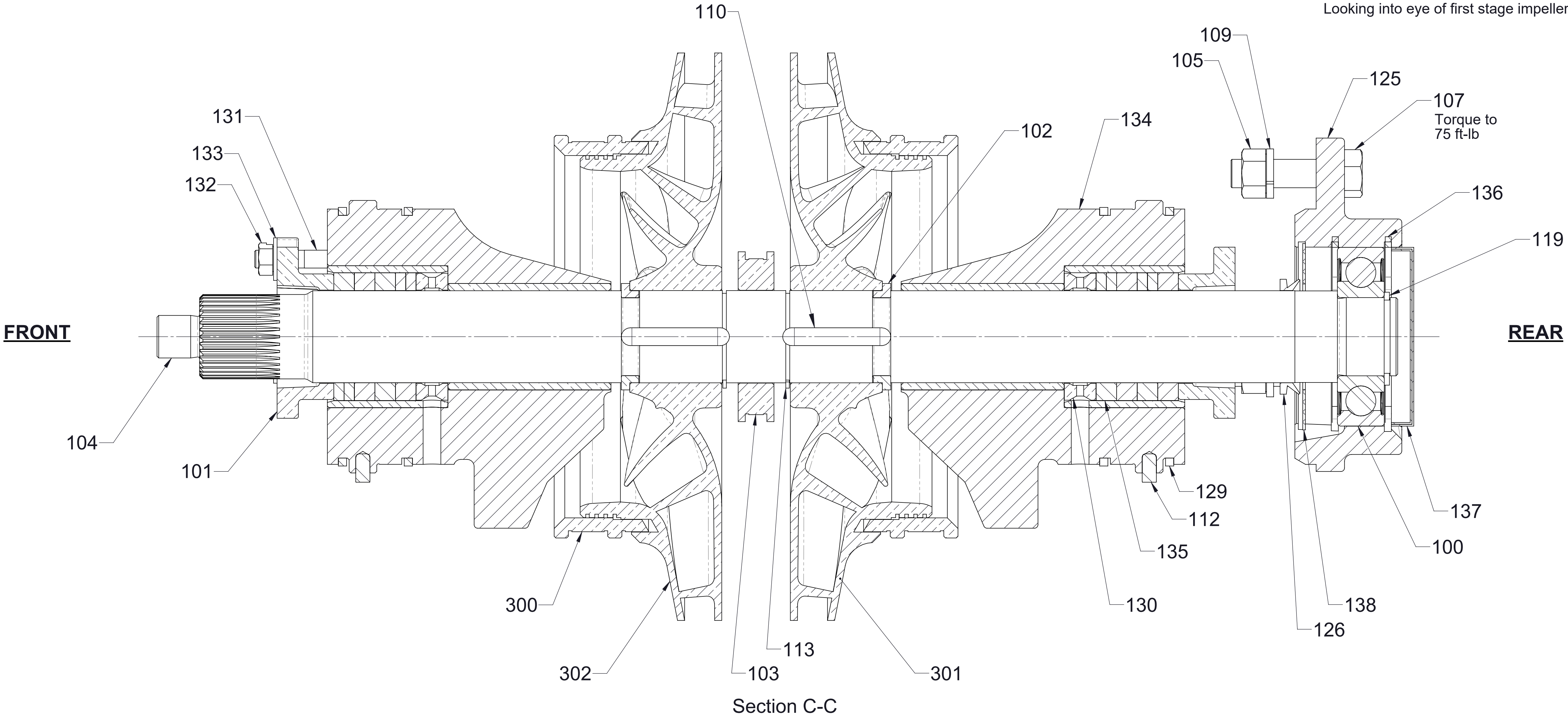
Section C-C
