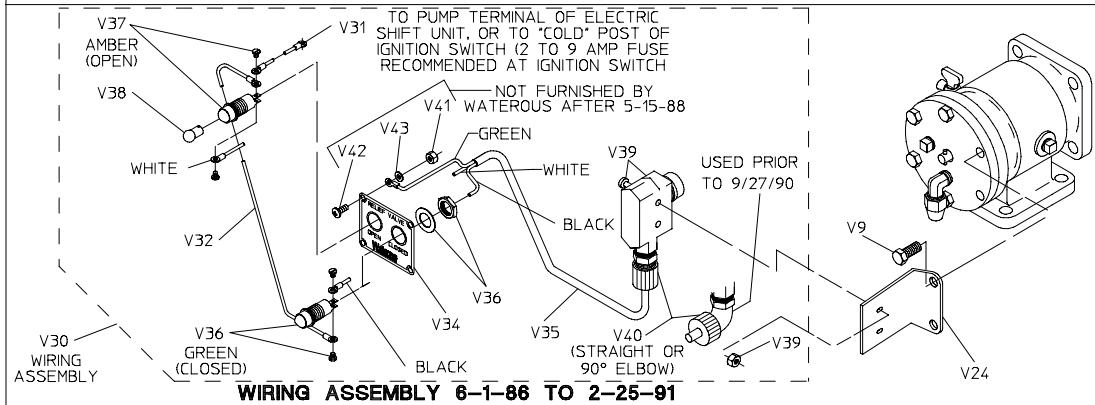
WIRING ASSEMBLY 6-1-86 TO 2-25-91
