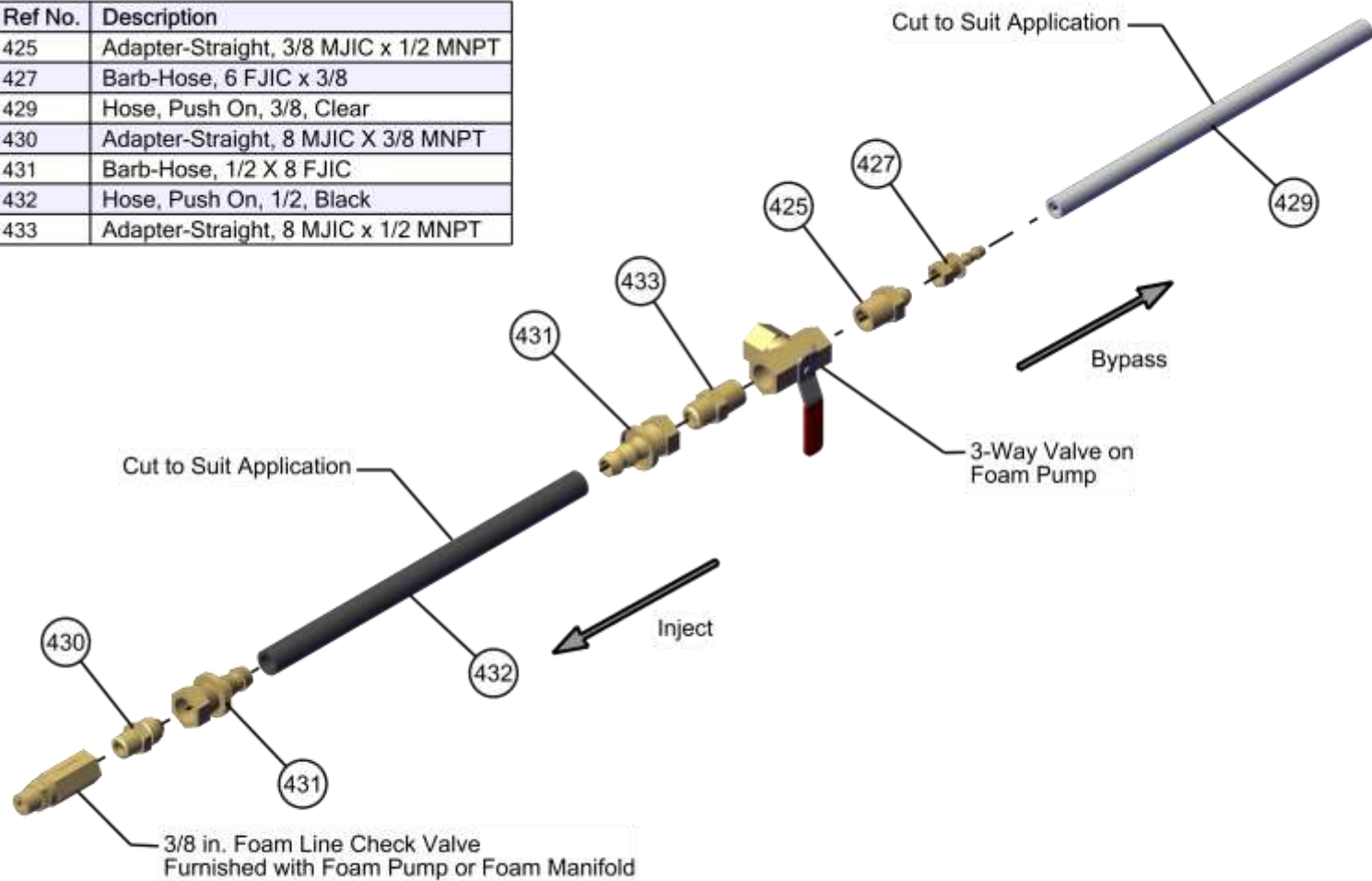
1/2 in. Foam Inject & Bypass Lines
