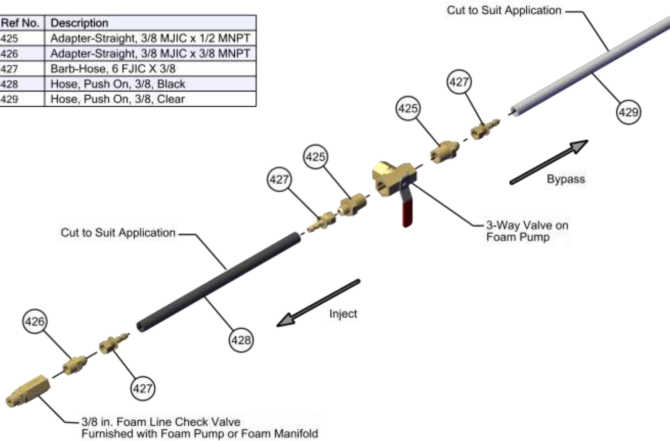
3/8 in. Foam Inject & Bypass Lines
