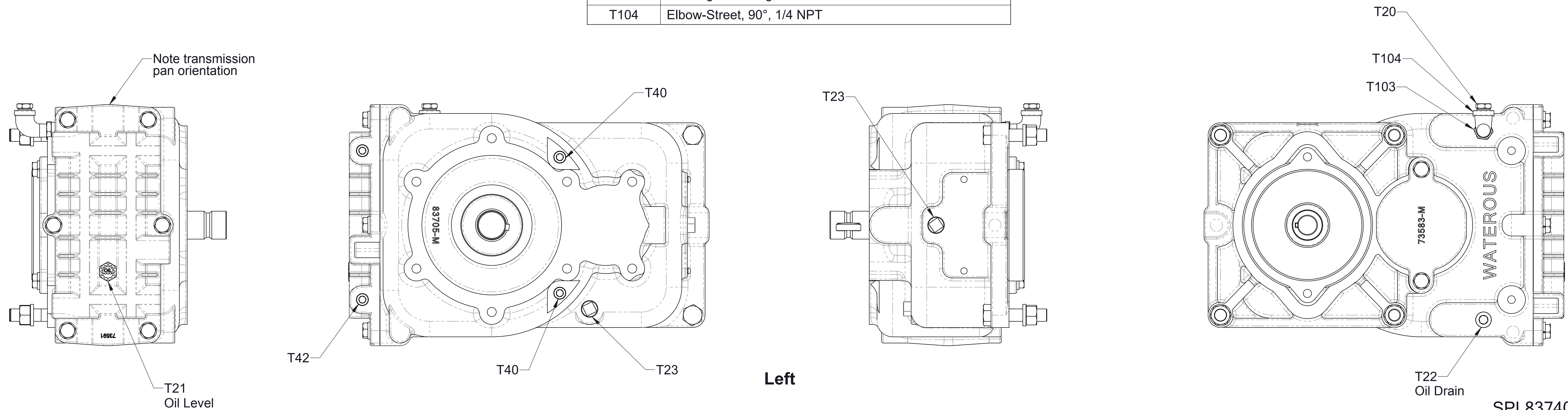
Breather, Drain, Oil Level, and Plug Locations Left and Right Mounting Positions
