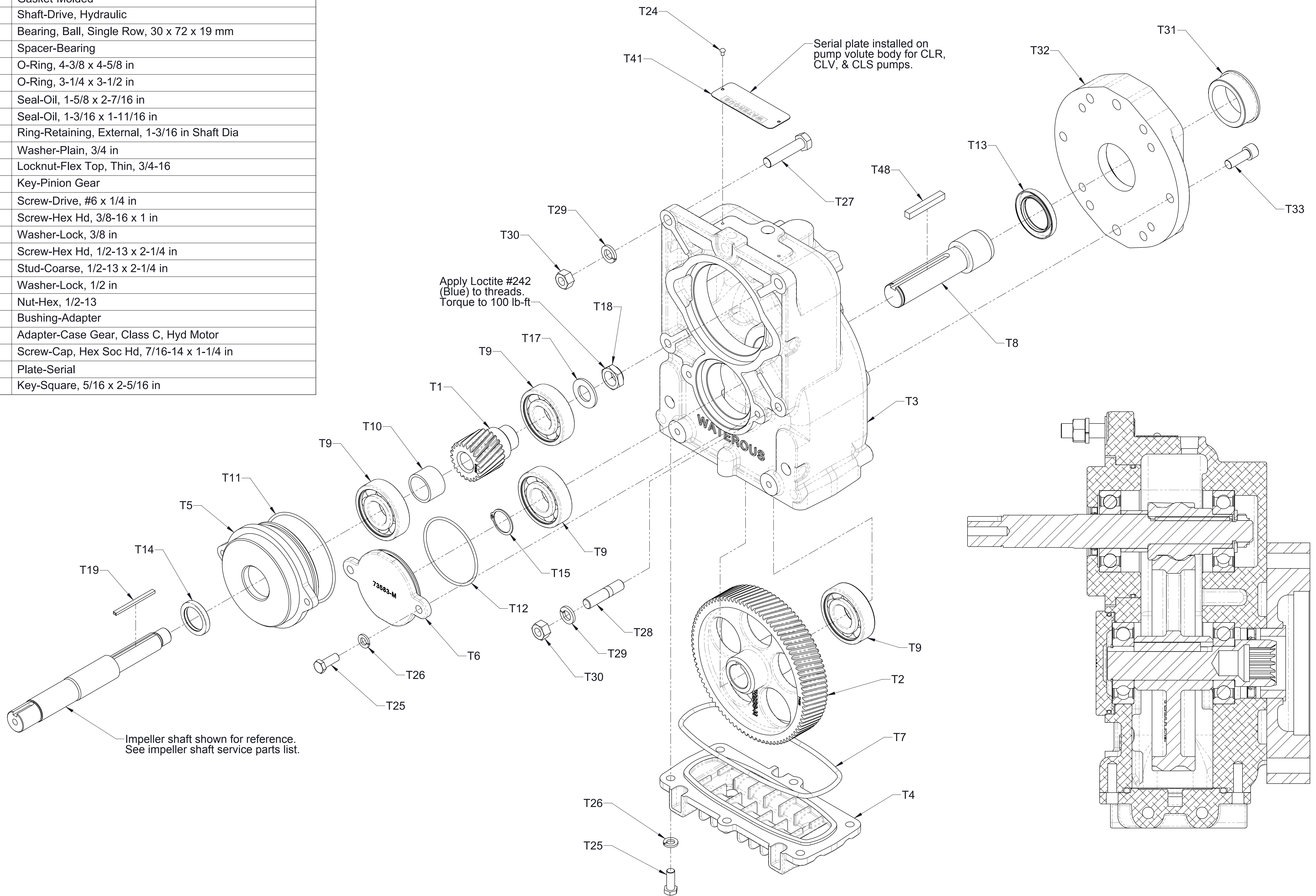
Transmission Assembly One Piece Impeller Shaft w/o Extension, SAE Class C Hydraulic Adapter CP-2, CP-4, CLR, CLV, CLS
