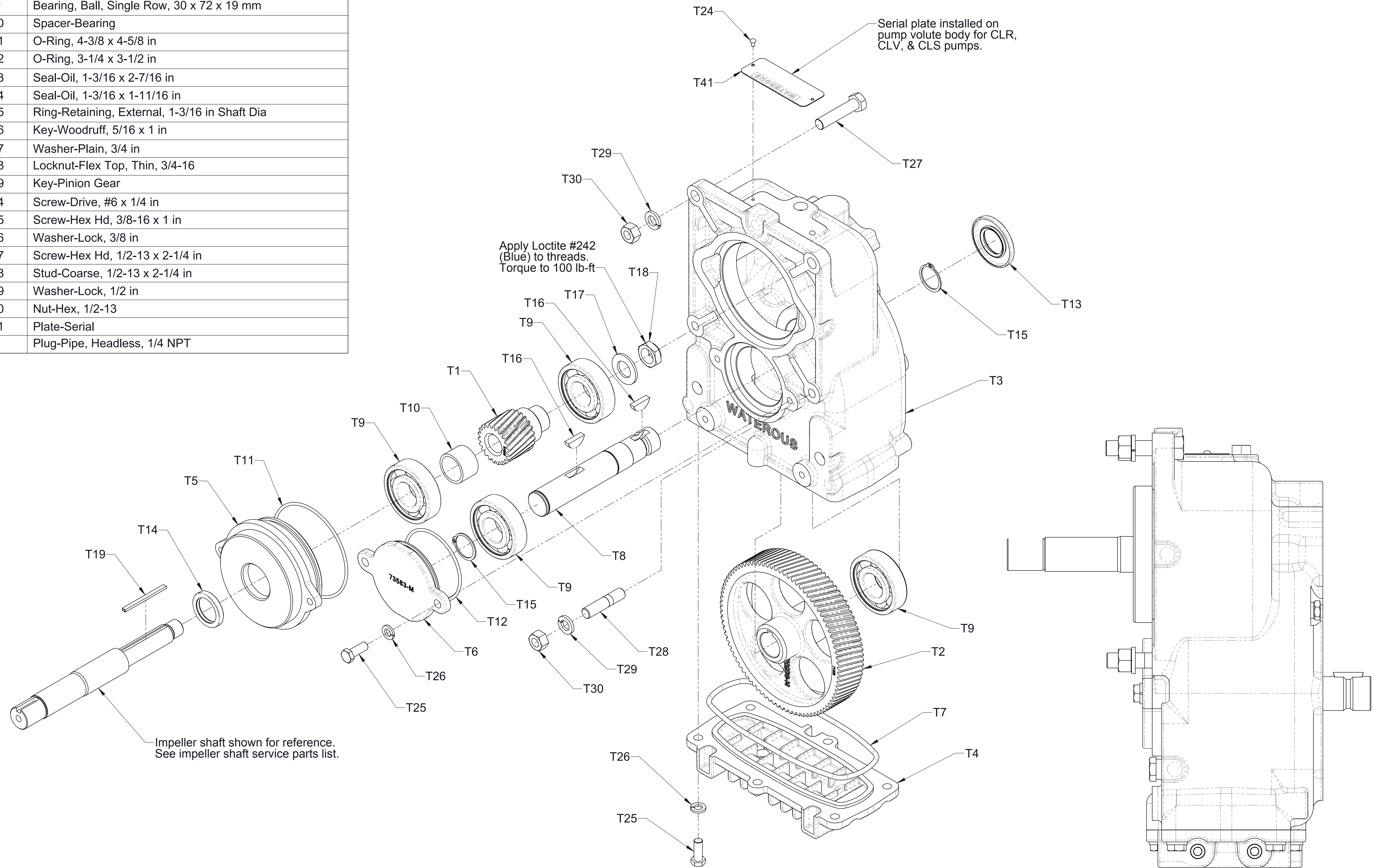
Transmission Assembly One Piece Impeller Shaft w/o Extension, 1-1/8in. Keyed Input CP-2, CP-4, CLR, CLV, CLS
